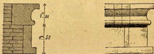
FIGS. 98, 99.—Assyrian mouldings. Section and elevation; from Botta.
