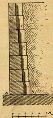
FIG. 45.—Section of wall through AB in Fig. 44; from Place.
