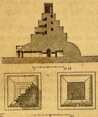
FIGS. 180—182:—Square Assyrian temple. Longitudinal section, horizontal section and plan.
