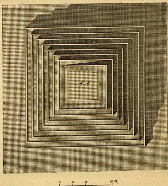
FIG. 186.—The Observatory restored. Plan.
