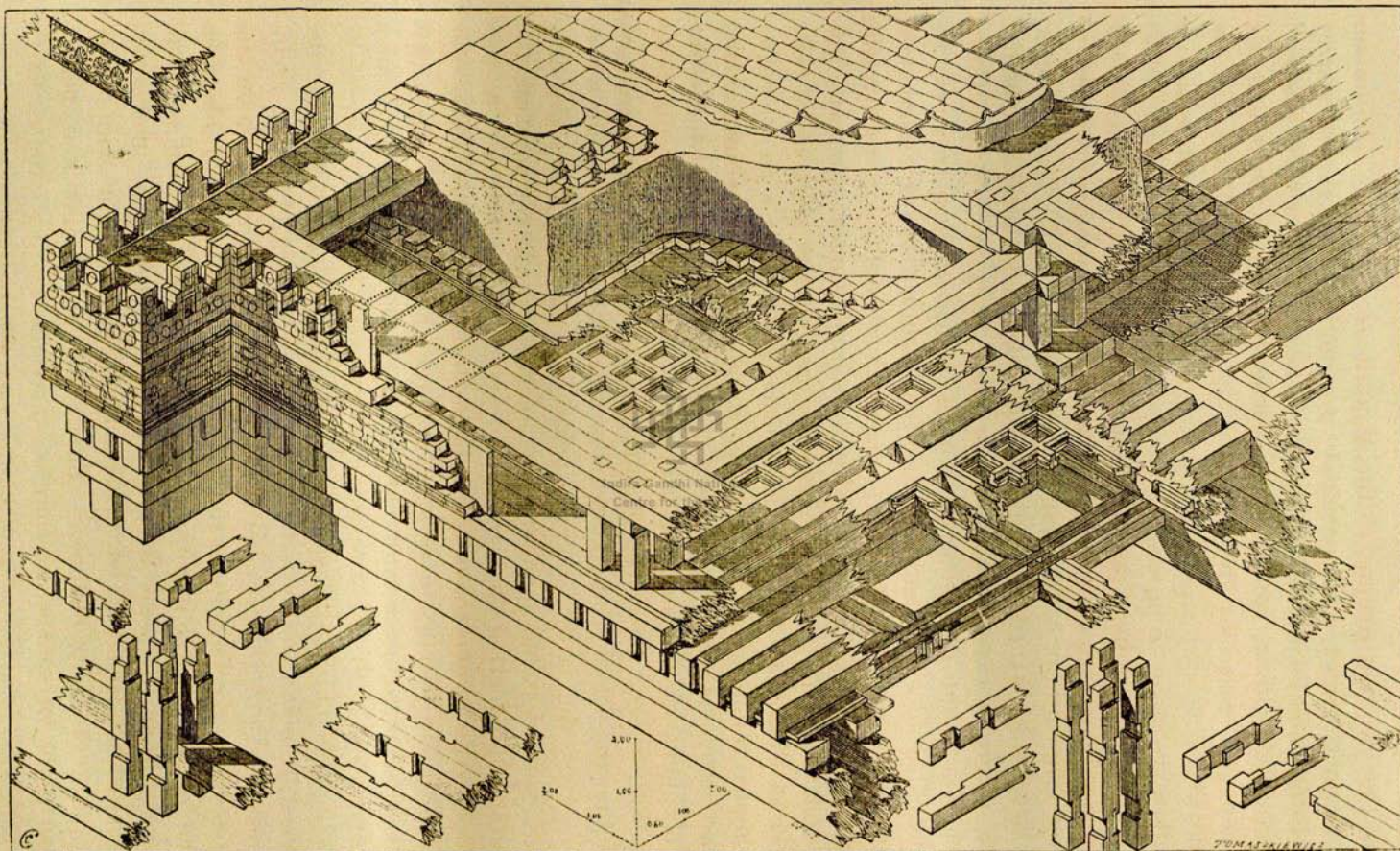
FIG. 27.—Woodwork of hypostyle hall of Xerxes. Isometric projection (No. 2 in plan) Restored by Ch. Chipiez.
