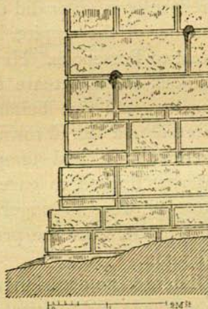
FIG. 142.—The Takht. Section of courses. Ibid.
