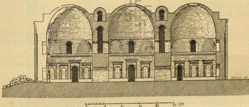
FIG. 77.—Feruz-Abad. Section through width. FLANDIN and COSTE, Ibid. , Plate XL.
