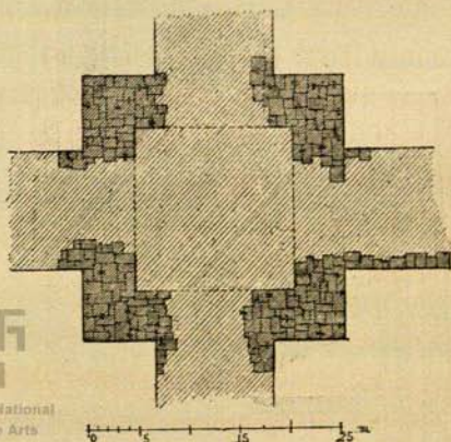
FIG. 125.—Ferüz-Abad. Fire-temple. Plan. FLANDIN and COSTE, Perse ancienne . Plate XXXVII.
