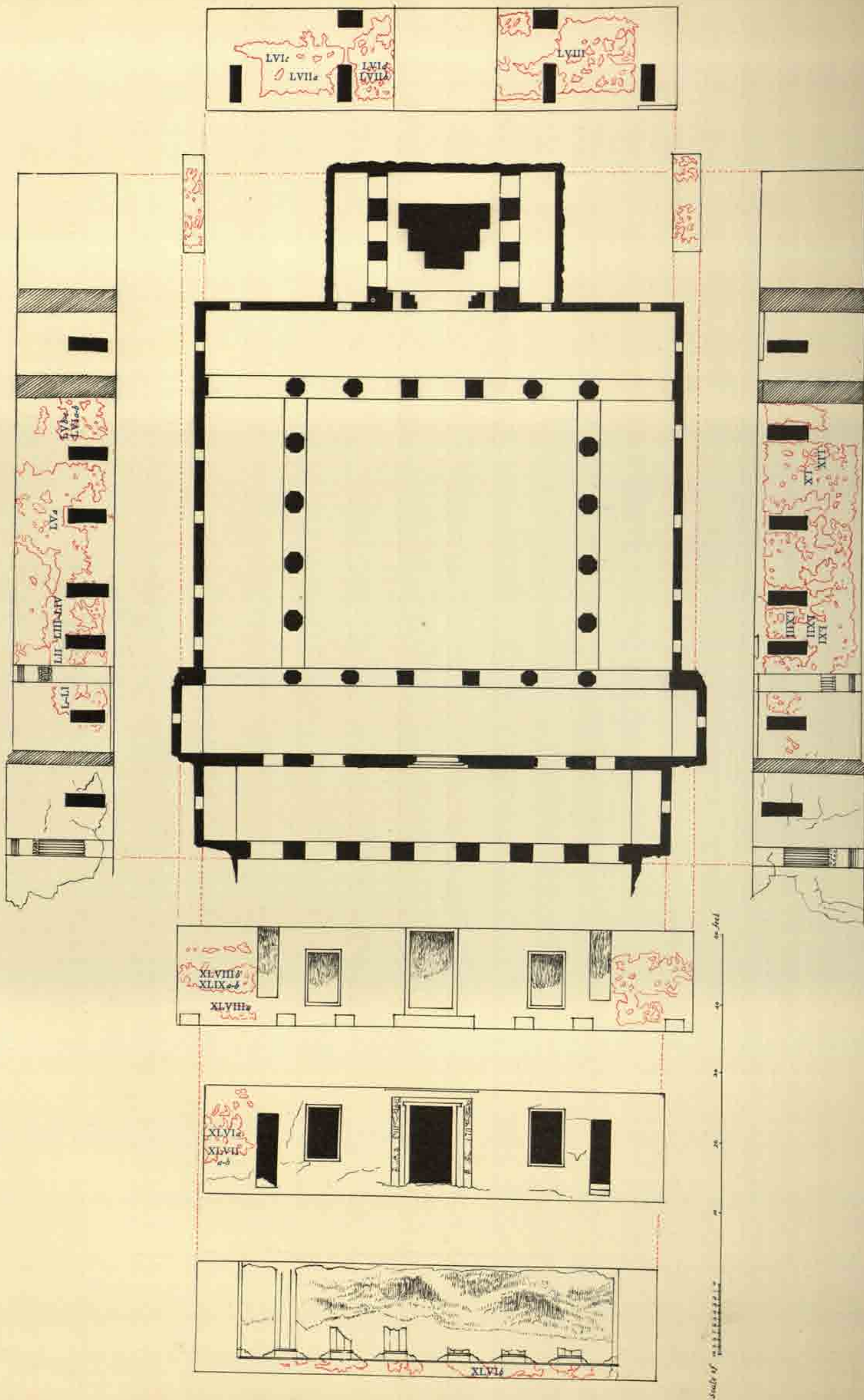
THE PLAN: CAVE XVI
