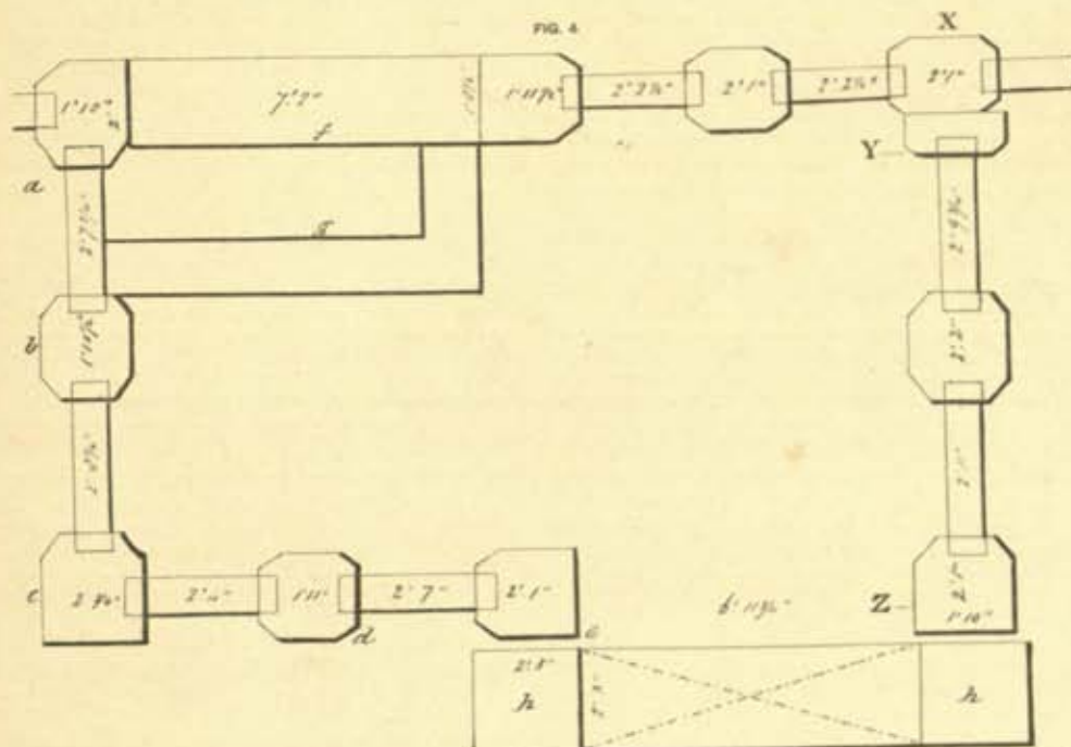
Fig. 4. Ground plan of the Northern entrance to the large, or No. 1 Sthūpa (h h are the sculptured Gate-pillars).
