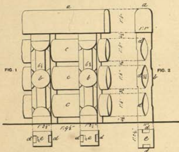
Fig. 1, 2. Front and side views of palisade of small Sthūpa (No. 2). a.a. coping: b.b. uprights: c.c. cross pieces: d.d. sockets for do.: e.e. section of uprights. Fig. 3. Upright on a large scale, showing the style of decoration of the bases. Fig. 4. Stone cauldron or cistern, between the large and small Sthūpas; interior dimensions, 4' 6" diam. 2' 6" deep.
