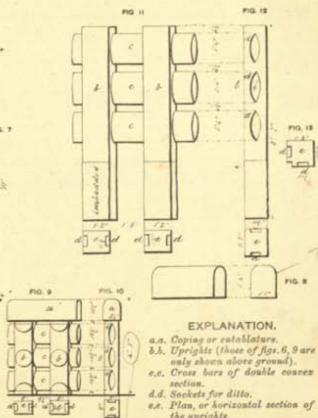
Figs. 6, 7. Front and side view of lower palisade (Plate II. a.a). 8. Rail or balustrade, which probably encircled Berm (Pl. II. c.) 9, 10. Front and side view of upper palisade (Pl. II. c.v.) 11, 12. " " enclosure round Tee. 13. Angle of do. (Plate II. t.t.)
