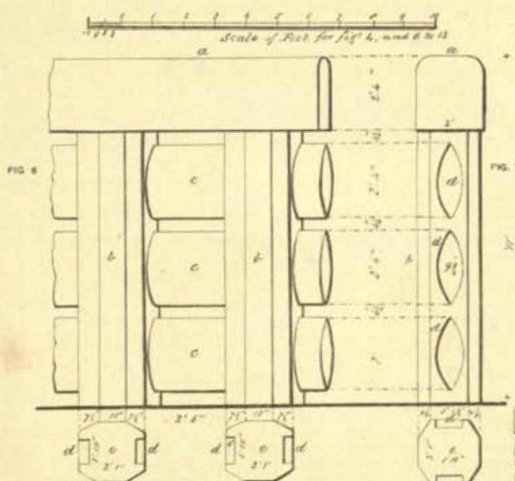
Figs. 6, 7. Front and side view of lower palisade (Plate II. a.a). 8. Rail or balustrade, which probably encircled Berm (Pl. II. c.) 9, 10. Front and side view of upper palisade (Pl. II. c.v.) 11, 12. " " enclosure round Tee. 13. Angle of do. (Plate II. t.t.)
