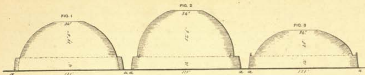
Figs. 1, 2, 3. Comparative sections of the large, or No. 1 Sthūpa, as represented by different writers on Sānchi.
