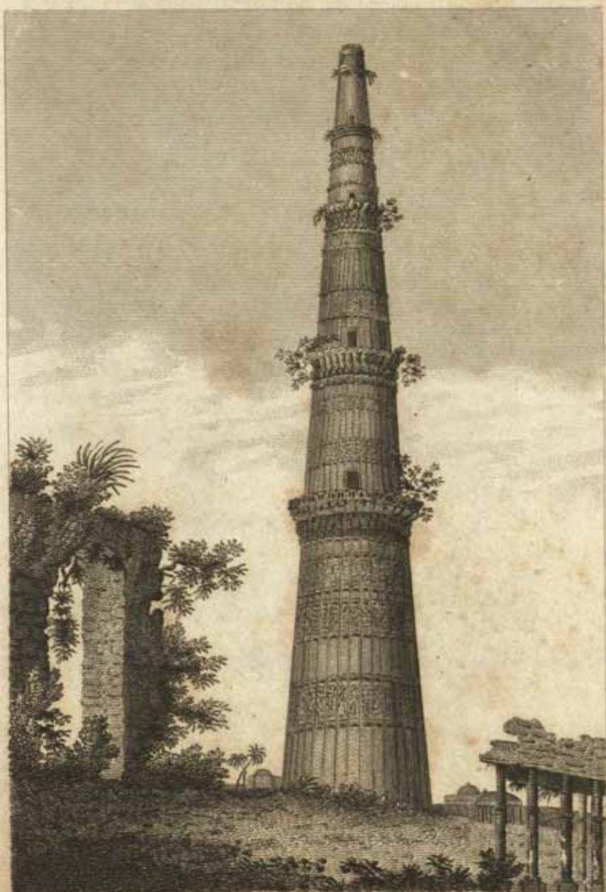
S.W.VIEW OF THE CÔÔTUB MINAR .
