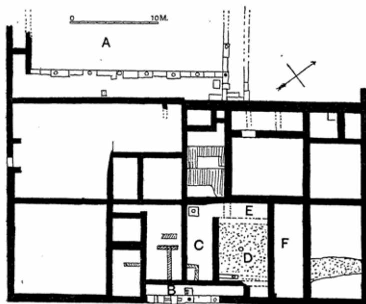
Fig. 38. House at Peiraeus
