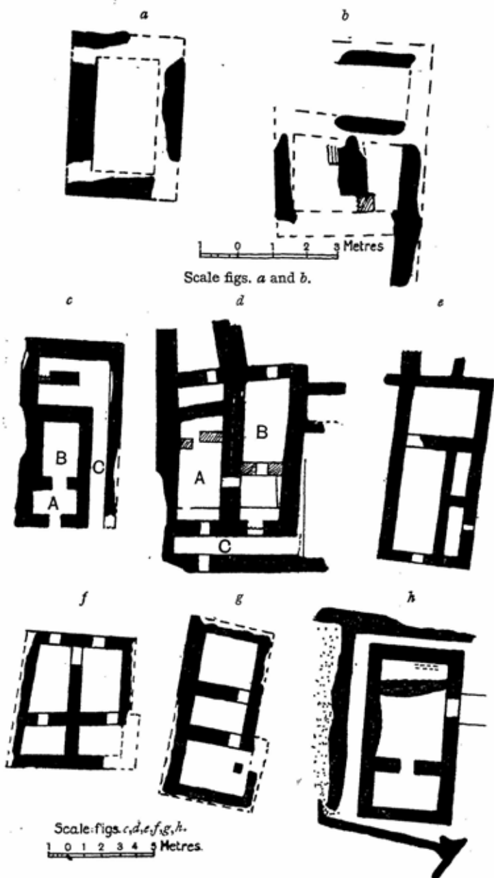
Fig. 31. Houses at Phylakopi.
