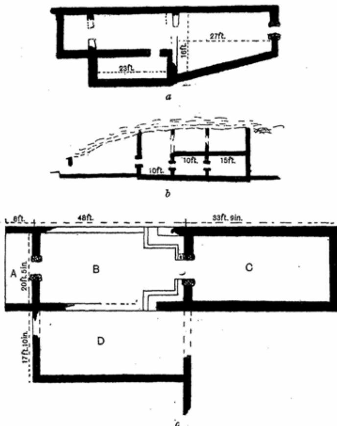
Fig. 30. Houses at Goulas.
