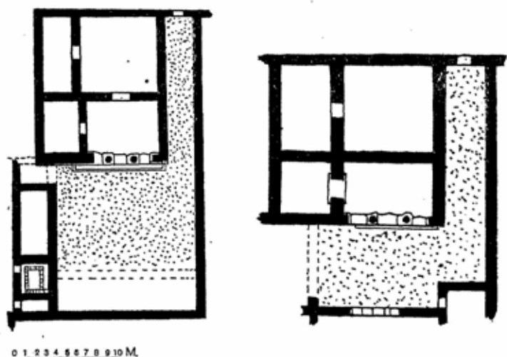
Fig. 43. Houses at Priene.
