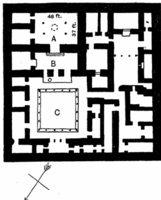
Fig. 41. Palace at Nippur
