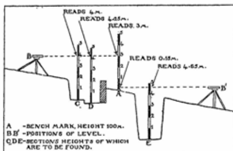
Fig. 4. The use of the Dumpy Level.
