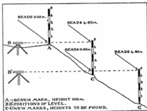
Fig. 5. The use of the Dumpy Level.
