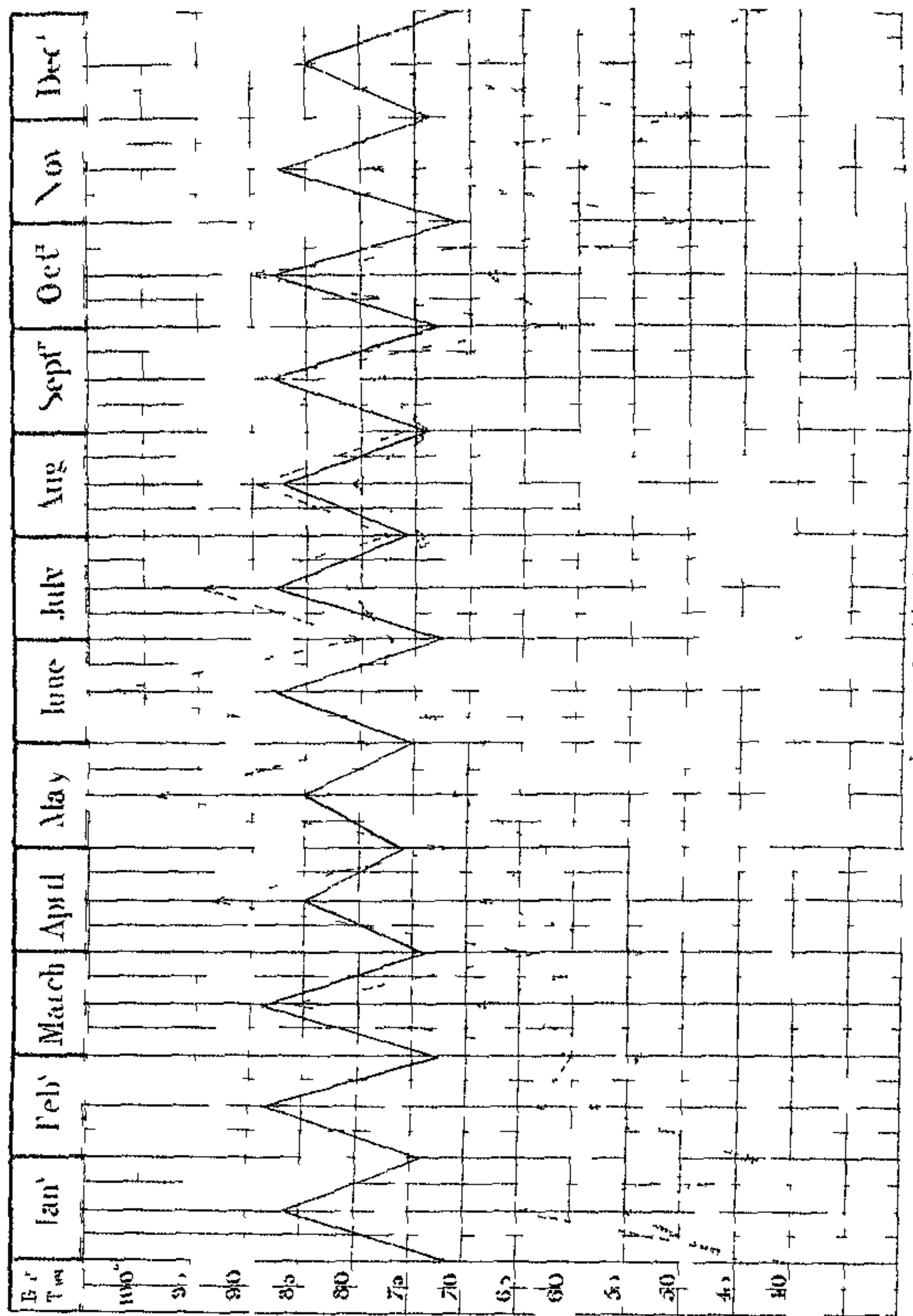
DIAGRAM OF THE CLIMATE OF INDIA.
