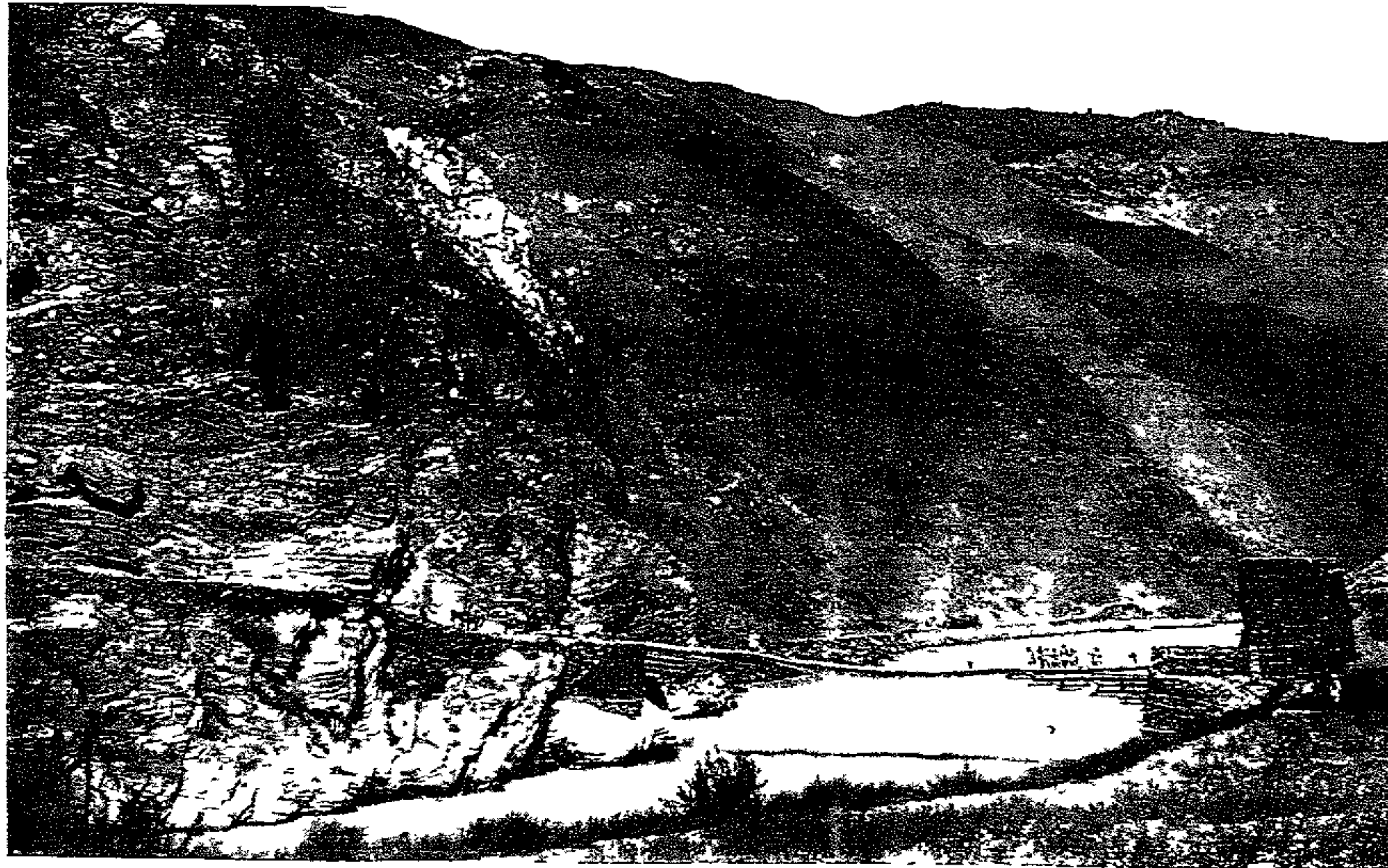
CHIRAL BRIDGE
