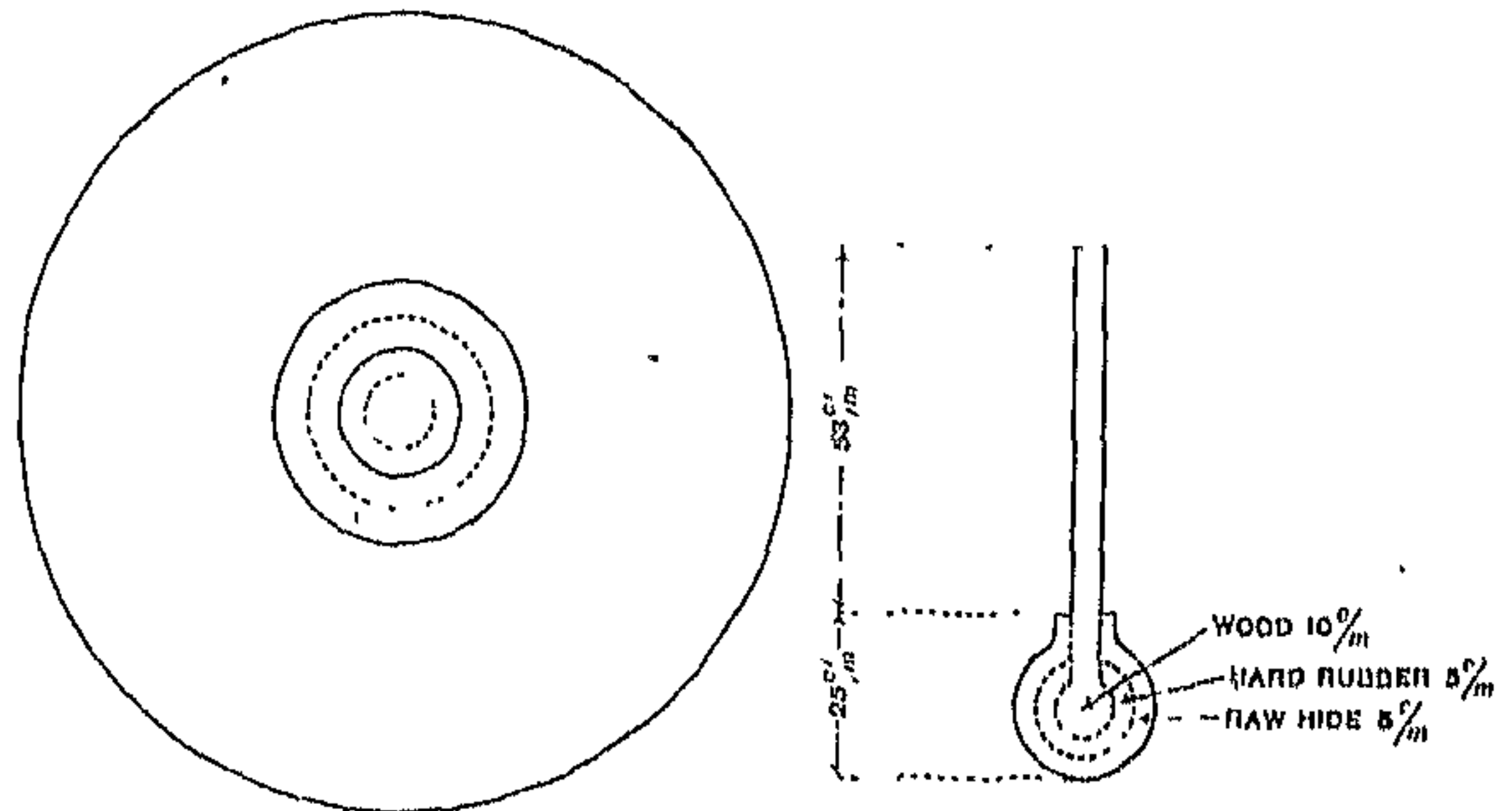
Fig. 28. Signalling gong from the Catuquimar Indians. After Church. This gong or drum is, as apparent from the drawing, partly buried in the ground.
