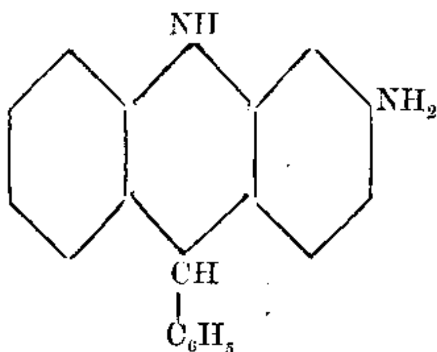
Diamidohydrophenylacridine.
