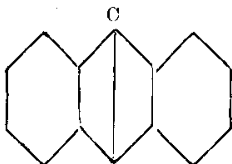
Phenazine.
