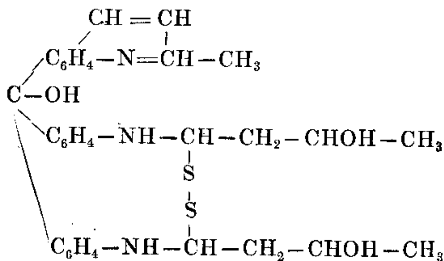
Lucius's Green.
