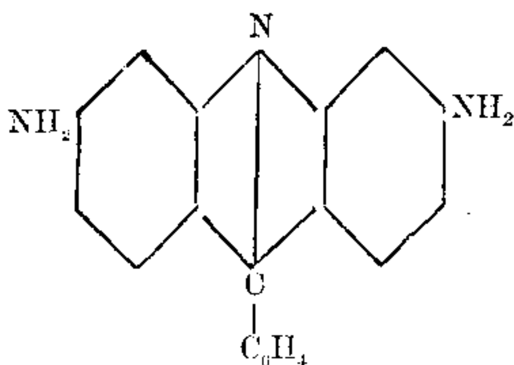
Benzoflavine.
