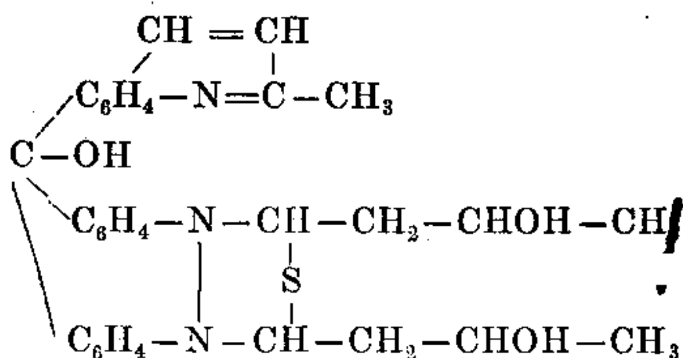
Usèbe's Green.
