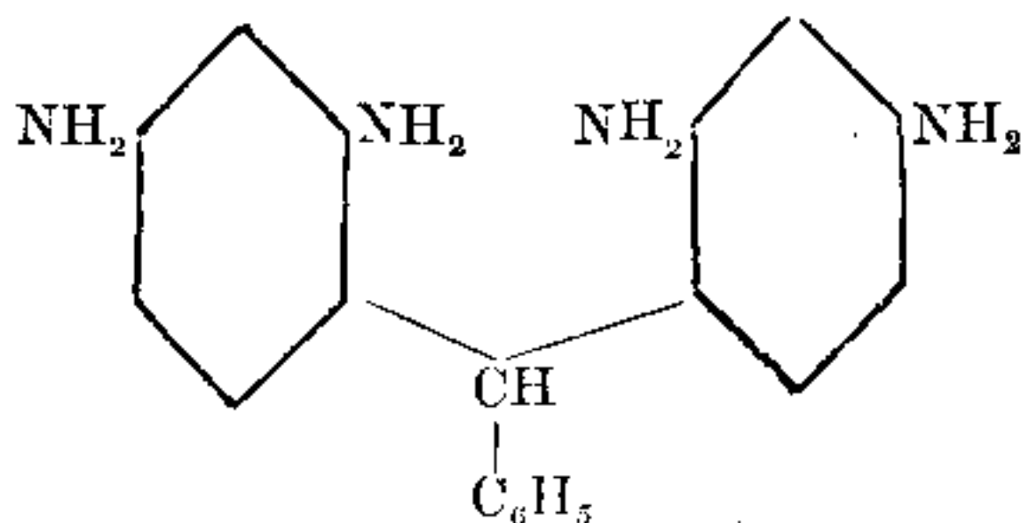
Tetramidotriphenylmethane.
