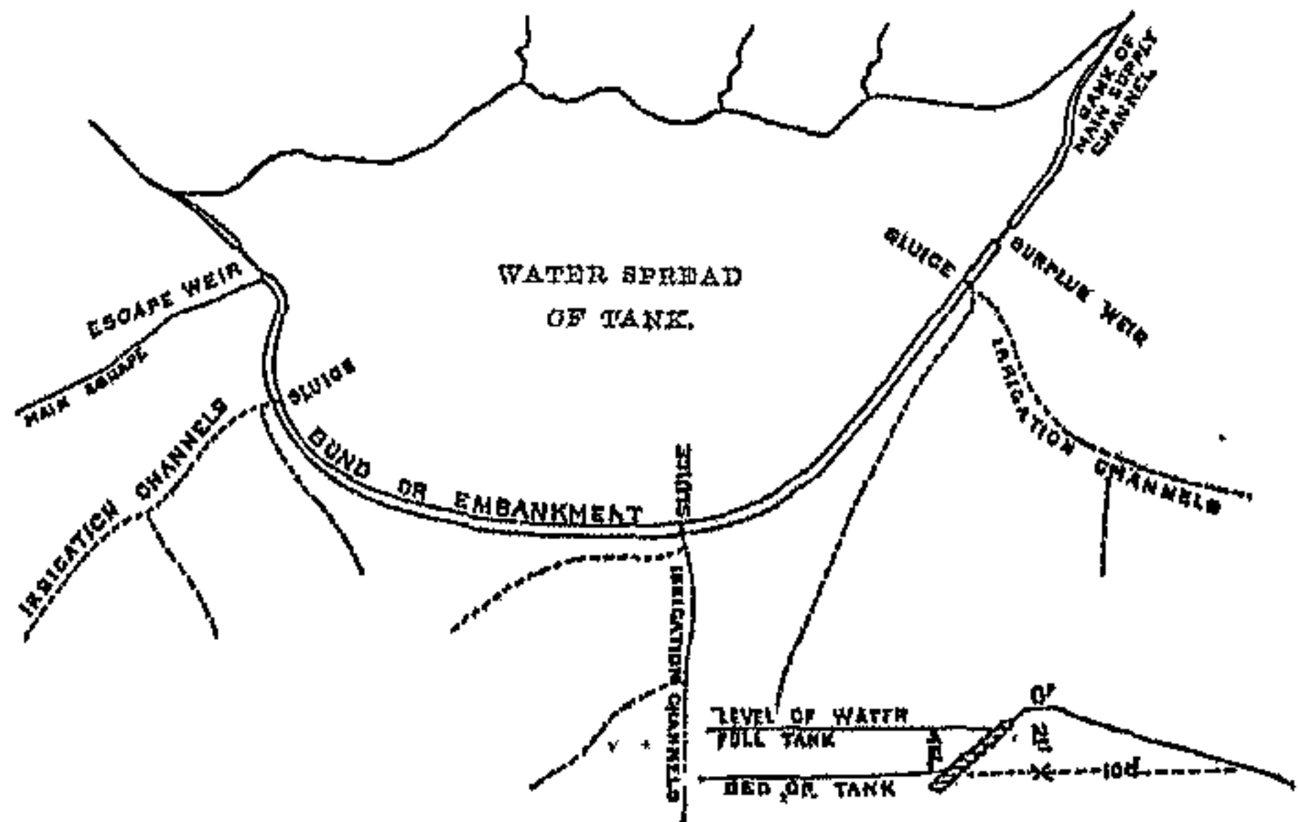
PLAN OF HORSESHOE TANK ON THE INCLINE WITHOUT BLUFFS.
