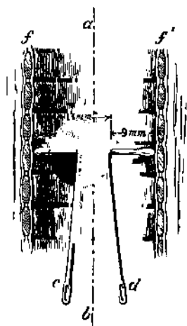
Fig. 15.—Diagram with half of the trachea supposed to be removed. f f' represent the outer walls of the trachea; the other letters are the same as in Fig. 13. It will be seen that Bramann's incision, instead of being in the median line, was three millimetres to the right of it.
