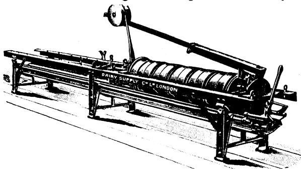
FACTORY OR GANG CHEESE PRESS
