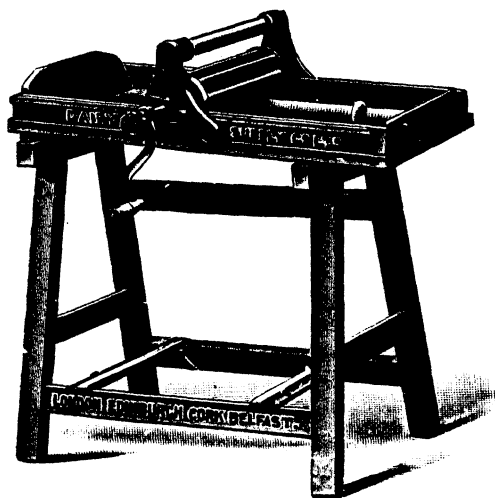
HAND-POWER BUTTER WORKER
