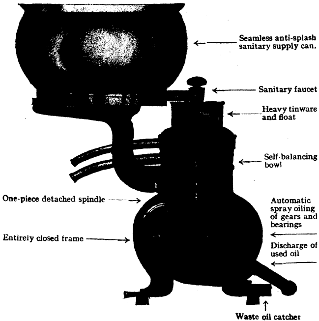
A CREAM SEPARATOR (sectional cut)
