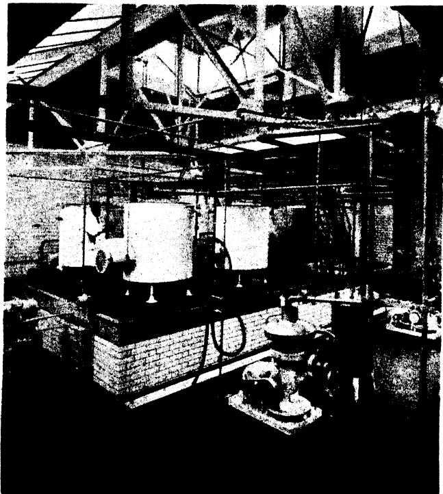
A compact and conveniently arranged modern dairy, showing "Pfaudler" glass-lined steel pasteurizer-holders in the background
