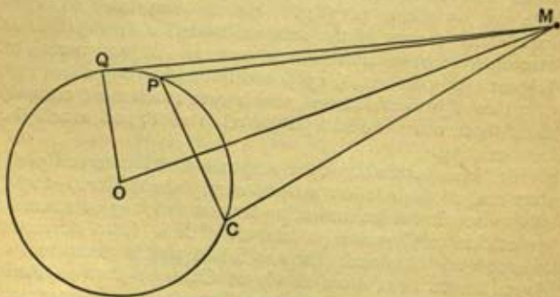
FIG. 69.—The parallax of a planet.
