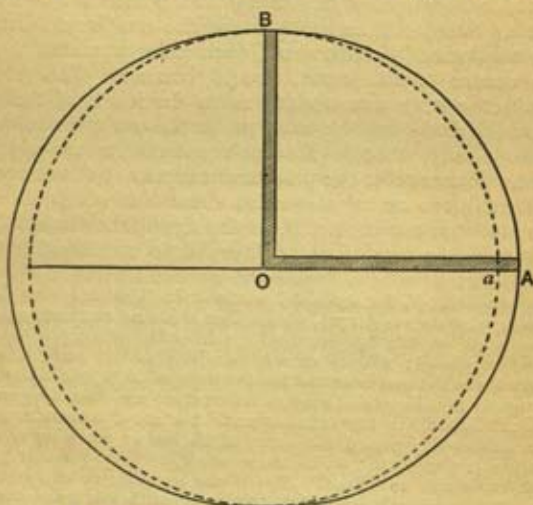
FIG. 72.—The spheroidal form of the earth.
