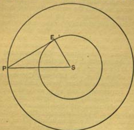
FIG. 46.—The relative sizes of the orbits of the earth and of a superior planet.
