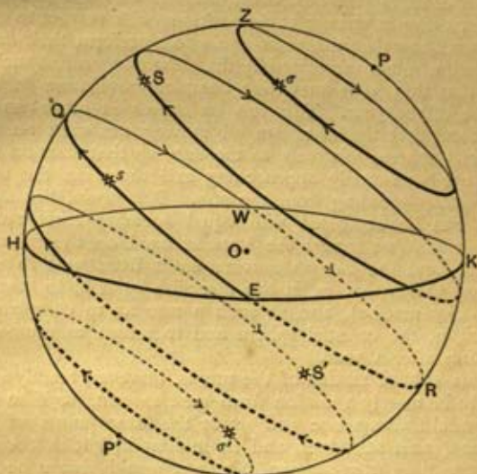
FIG. 3.—The circles of the celestial sphere.
