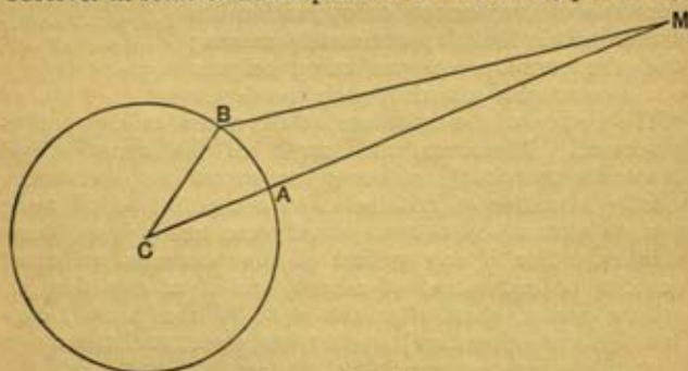
FIG. 31.—Parallax.
