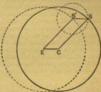
FIG. 19.—The epicycle and the deferent.
