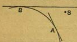
FIG. 12.—The curvature of the earth.
