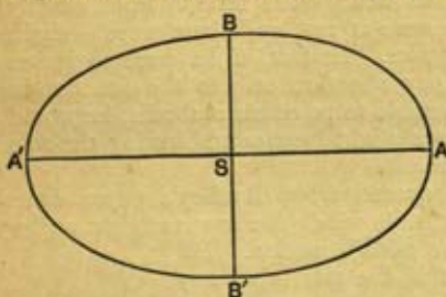
FIG. 76.—The aberrational ellipse.
