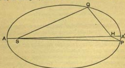
FIG. 59.—An ellipse.
