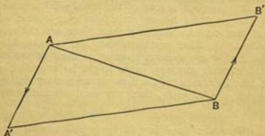
FIG. 37.—Relative motion.
