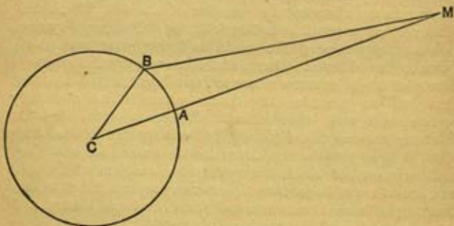
FIG. 33.—Parallax.
