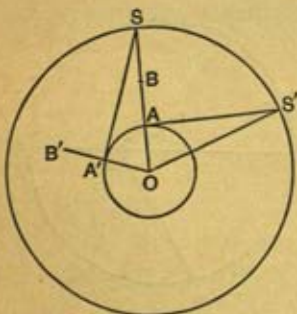
Fig. 39.—The daily rotation of the earth.
