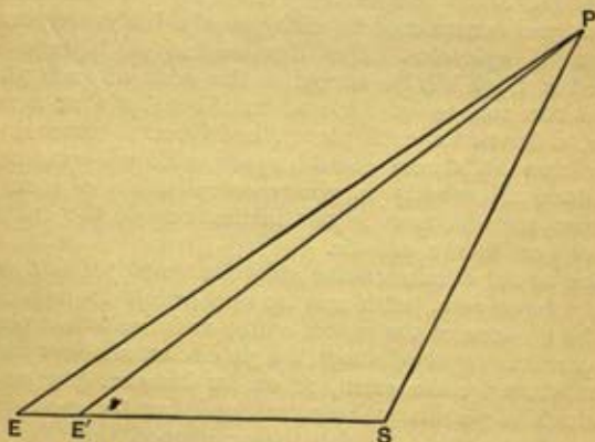
FIG. 49.—The alteration in a planet's apparent position due to an alteration in the earth's distance from the sun.
