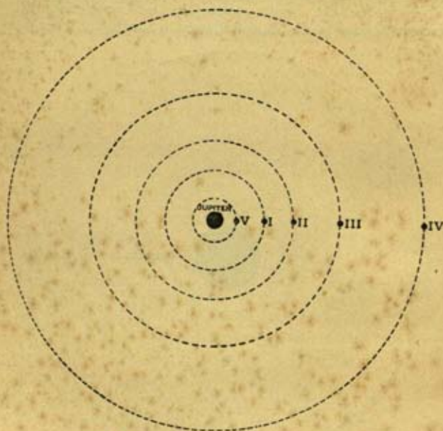
FIG. 93.—Jupiter and its satellites.
