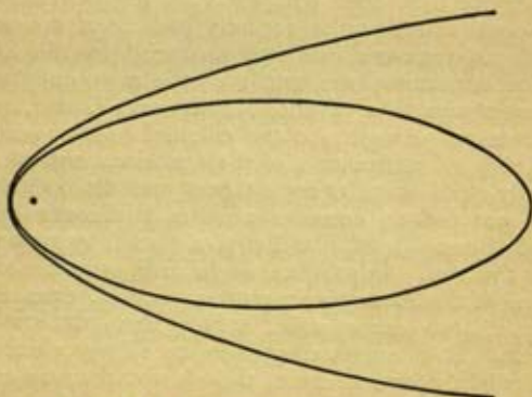
FIG. 73.—An elongated ellipse and a parabola.
