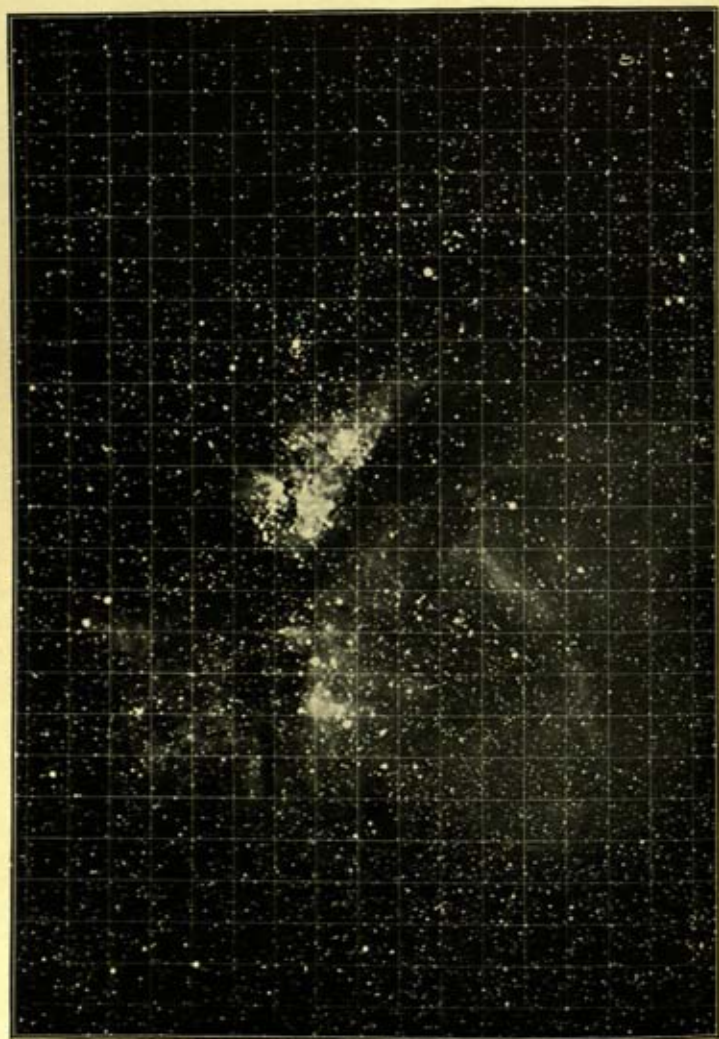
FIG. 100.—The nebula about \eta Argus. From a photograph by Dr. Gill.
