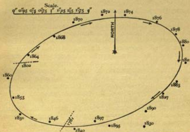
FIG. 101.—The orbit of \xi Ursae, shewing the relative positions of the two components at various times between 1781 and 1897. (The observations of 1781 and 1802 were only enough to determine the direction of the line joining the two components, not its length.)
