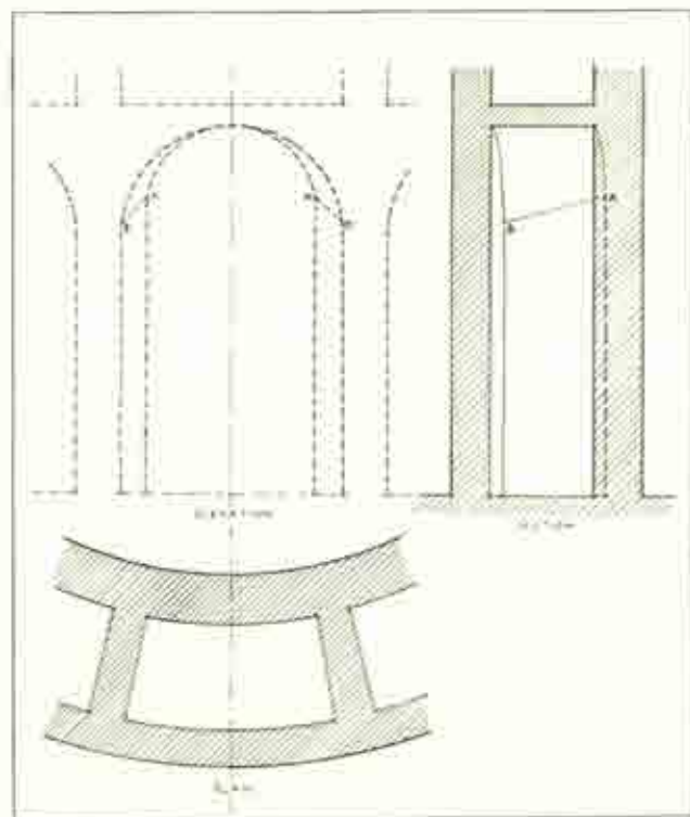
FIG. 1. WEDGE-SHAPED CHAMBERS.
