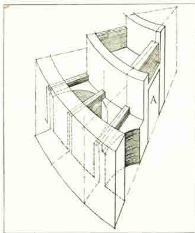
FIG. 2. TRANSMISSION OF STRESS: (A is one of the wedge-shaped chambers).
