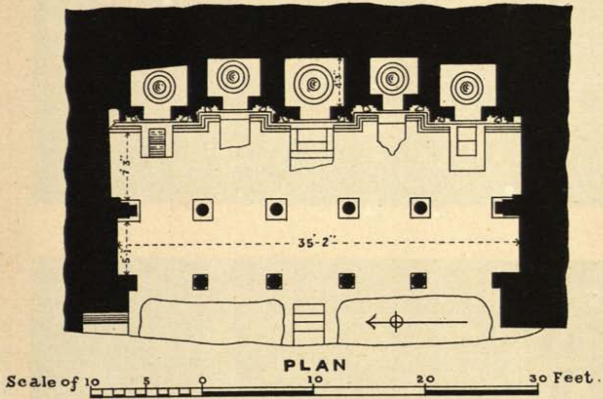
(a) TEMPLE NO. 3.
