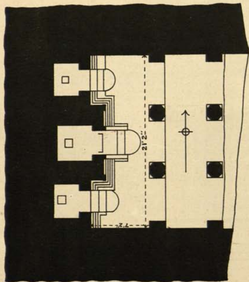
(a) DHARMARAJA'S MANDAPA (No. 1)
