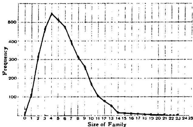
Fig. 3. Curve showing distribution of size of 3837 families in America containing deaf-mutes. (After Schuster, 'Hereditary Deafness,' Biometrika , Vol. iv. 1906, p. 474.)
