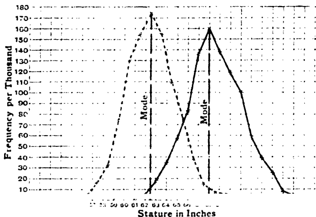
Fig. 2. Curves showing distribution of stature in women (mothers)—dotted line; and in men (fathers)—continuous line. The curves approach the 'normal curve.' (Data from Pearson.)
