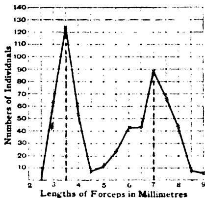
Fig. 5. Curve with two modes, representing frequency of lengths of forceps of male Earwigs from the Farne Islands. (After Bateson.)
