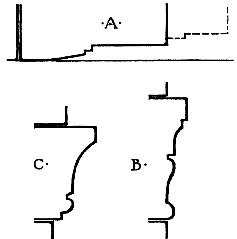
FIG. 45.—DETAILS OF VARIOUS MOULDINGS.
