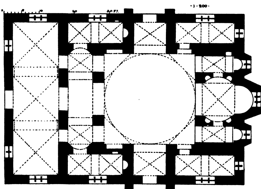
FIG. 7.—DAPHNI : ATTICA. PLAN AND SECTION.
