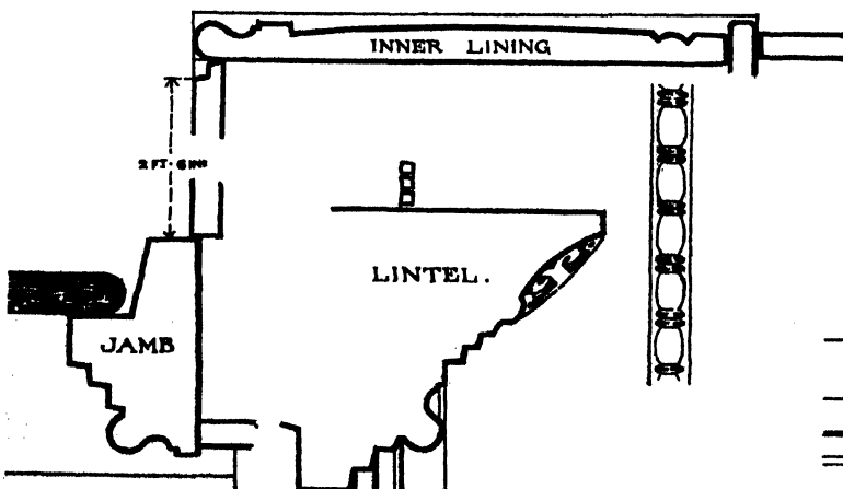
DETAILS OF DOOR FROM NARTHEX INTO GREAT CHURCH
