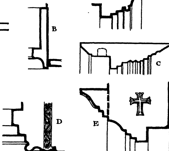
DETAILS OF VARIOUS DOORS
