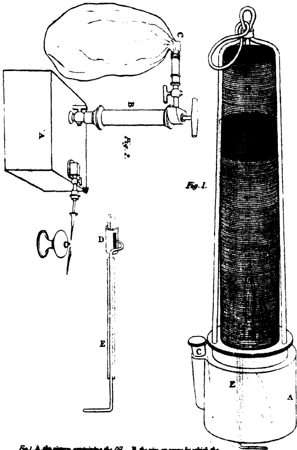
Fig. 1. A. the cistern containing the Oil. — B. the rim or screw by which the gauge cage is fixed to the cistern. — C. aperture for supplying Oil. E. a wire for tripping the wick. D. F. the wire gauge cylinder. — G. a double tip. Fig. 2. A. the reservoir of condensed air. — B. the condensing syringe. C. the bladder for Oxygen. — D. the movable jet.
