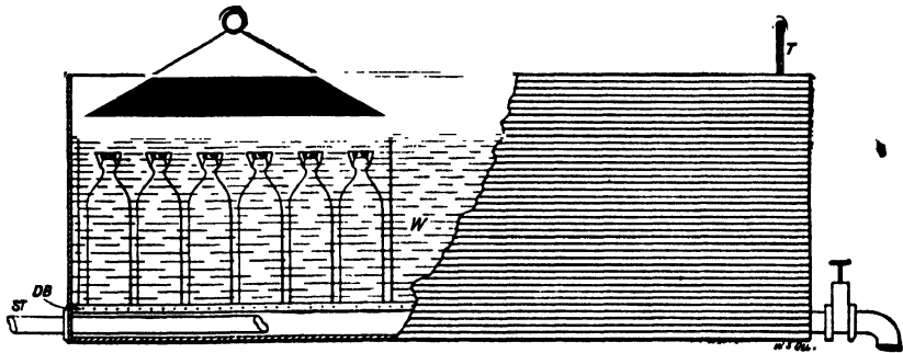
FIG. 3.—PASTEURIZER FOR JUICE IN BOTTLES
