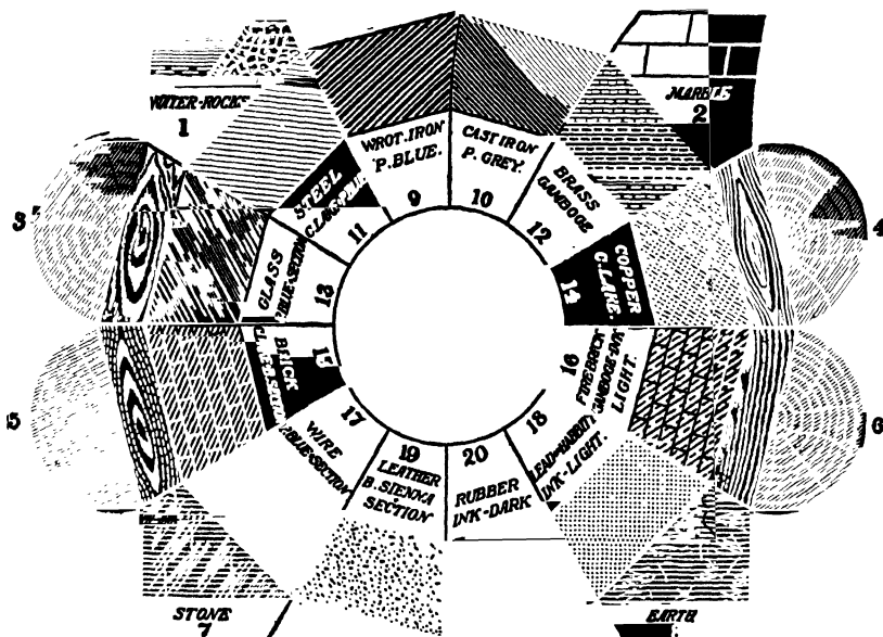
STANDARD CONVENTIONAL SECTIONS FOR DRAWINGS.
