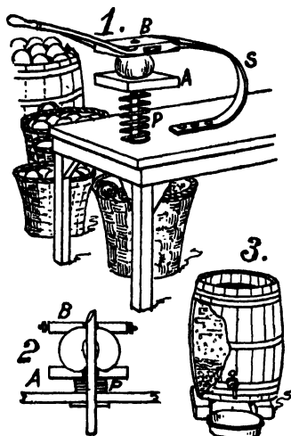
Coring Machine and Filter CIDER MAKING
