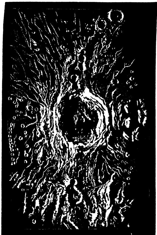
FIG. 2. —Lunar Crater Copernicus.
