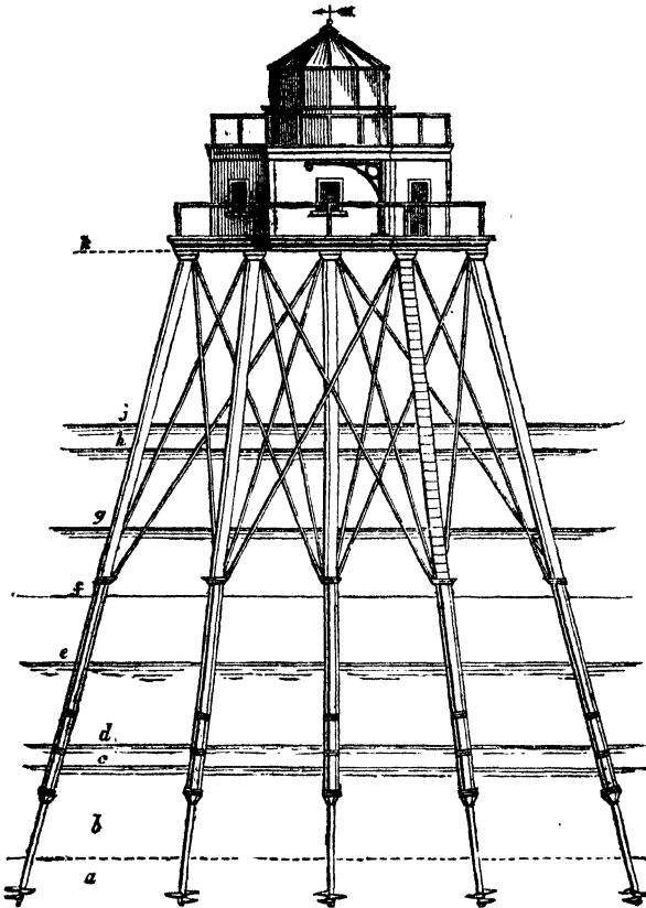
(The Wyre Screw-pile Lighthouse.)
