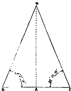
FIG. 105. Range-taking without a direction point (using second prism only).
