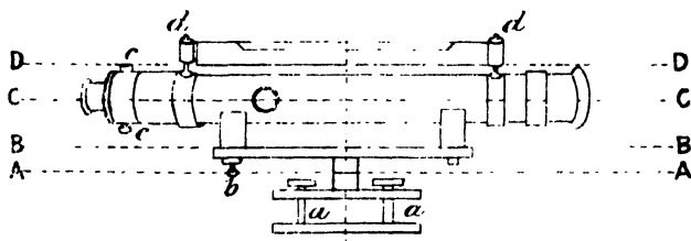
FIG. 86. DUMPY LEVEL.
