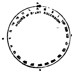
FIG. 132.—Position of the Celestial Equator at Culmination of Star at 0 hr. 14 min. 31 st 16 sec. Mean Time, May 18, and 4 hrs. Sidereal Time.
