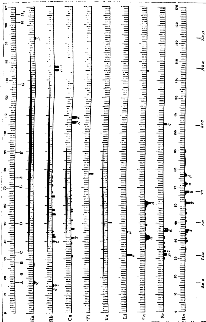
MAP OF THE SPECTRA OF THE ALKALIES AND ALKALINE EARTHS.
