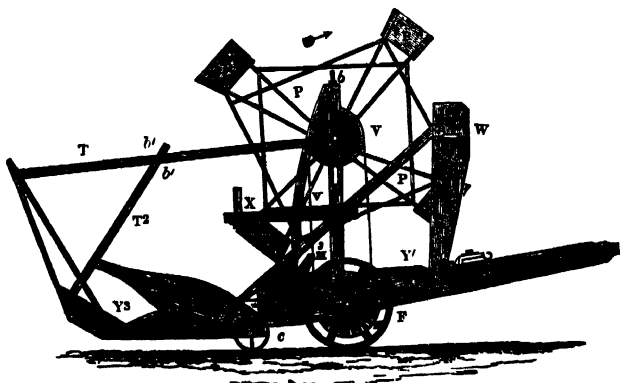
Fig. 27.—Elevation.
