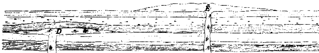
Interbedded and Overlying Igneous Rocks.
