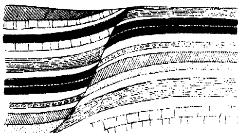
Distorted Fault
