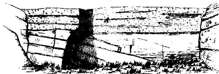
Unconformability. — Cheswardine, Salop.
