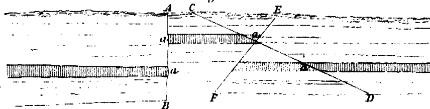
Direction of Throw.
