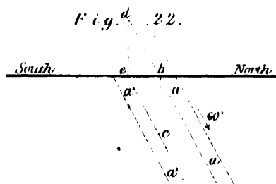
Lateral Shift - Section.
