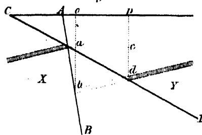
Throw in Inclined Bed
