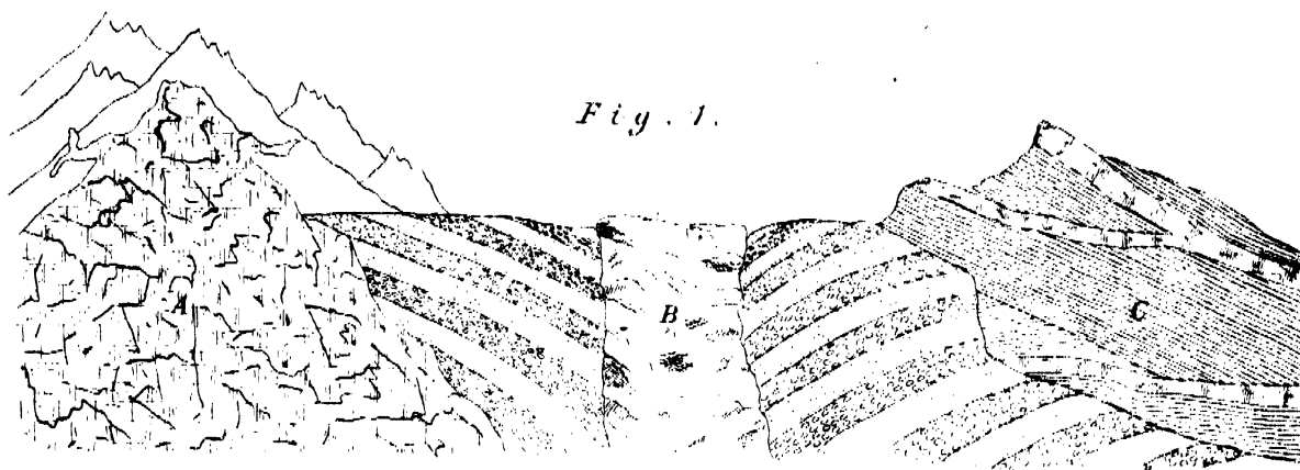
Eruptive, Disruptive and Intrusive Igneous Rocks.
