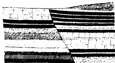
Fault of Dislocation.
