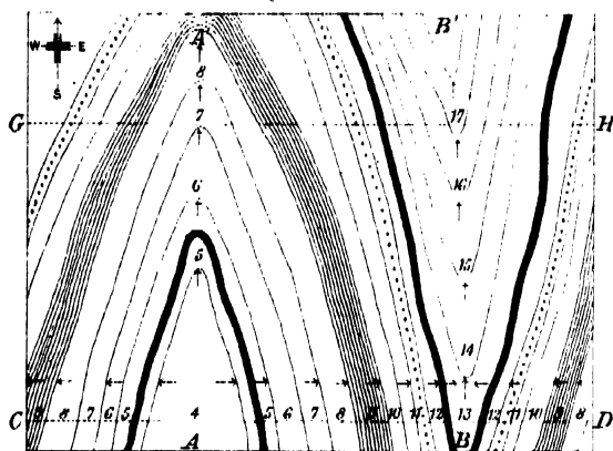
Anticlinal and Synclinal Curves — Plan.
