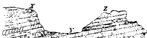
Effects of Denudation.
