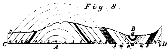
Anticlinal and Synclinal Curves. Section through C.D.
