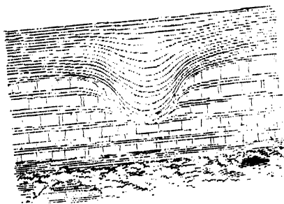
Trough near Paris.
