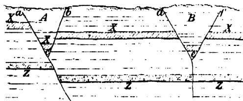
Trough Faults
