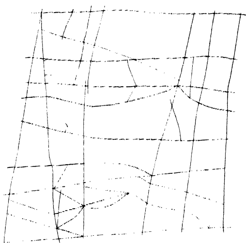
Plan of Joints in Rock — Burren, Co. Clare.
