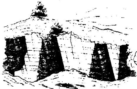
Rock Joints. Mallow, Co. Cork.
