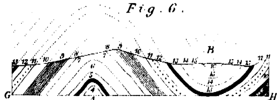
Anticlinal and Synclinal Curves. Section through G.H.
