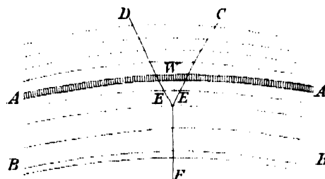
Trough Faults.
