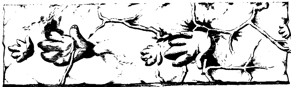
Footprints of Labyrinthodon giganteum .
