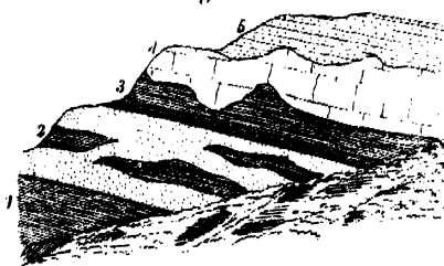
Fault of Erosion.
