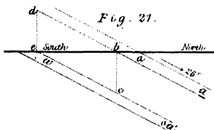
Lateral Shift - Section.
