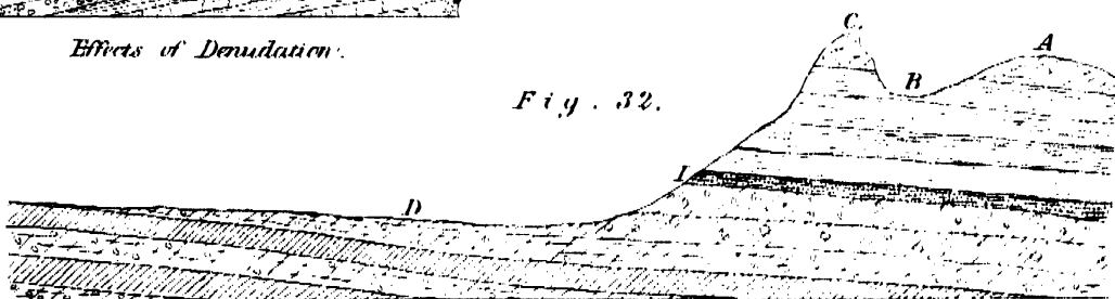
Effects of Denudation. — Newton, Yorkshire.
