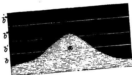
Swell or Horse's Back.
