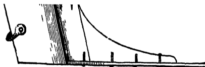
Stern of a Fowling Punt, fitted.
