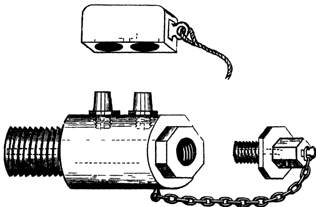
Double-cap side Plug for Muzzle-loading Swivel-guns.
