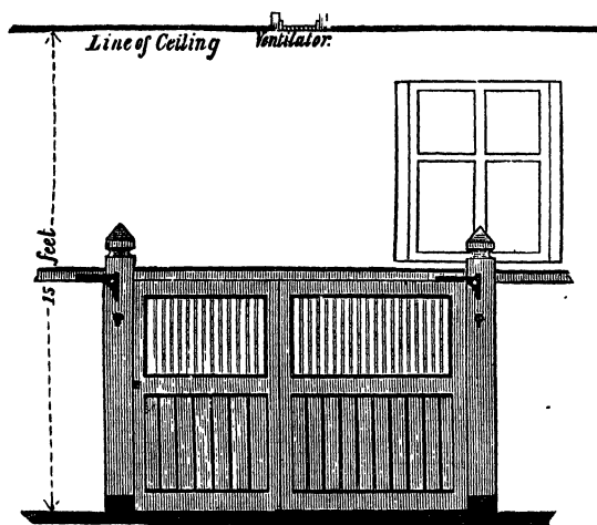
Elevation of Front of Loose Boxes, showing Height of Ceiling.
