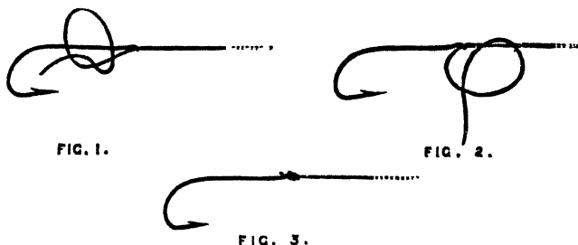
TWO METHODS OF TYING THE HALF-HITCH JAM KNOT FOR A BARE HOOK.
