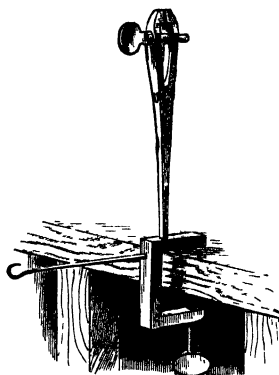
A TACKLE VICE.
