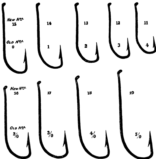
'PENNEL-LIMERICK' SALMON HOOKS WITH UP-TURN SHANKS AND TURN-DOWN EYES. (Patent United Kingdom, and U.S.A.)
