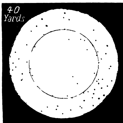
Pattern of the same CHOKE-BORED Gun at 40 Yards, with 49 grains of ® Schultze Powder and 1 1/4 oz. No. 6 Chilled Shot.
