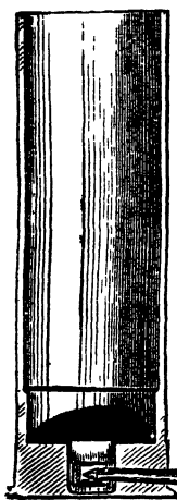
The Pin-fire Cartridge Case.
