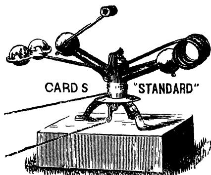
The "Card" Trap.
