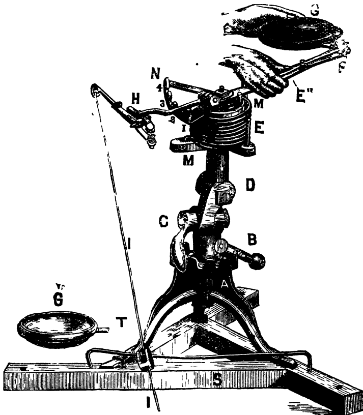
The Lagousky Clay Pigeon Trap.
