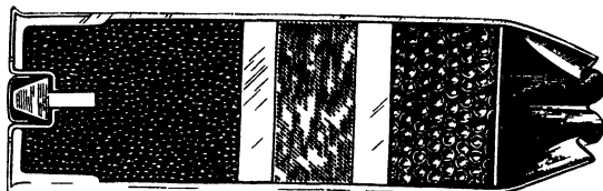
Brass Cartridge Case Wadded for Close Shooting
