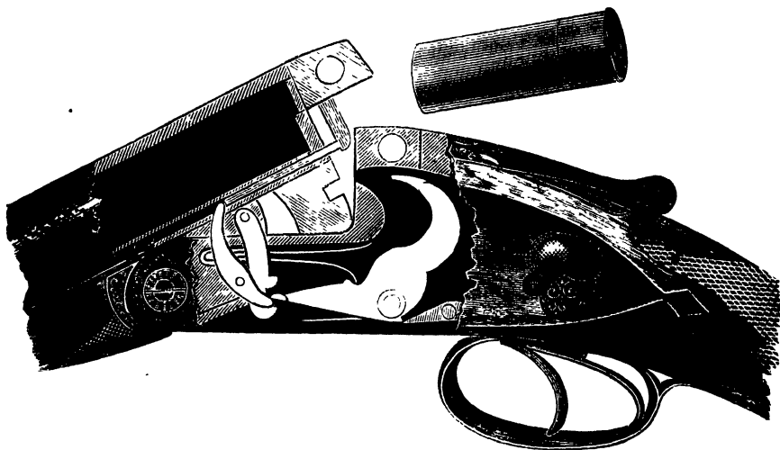
Mechanism of Greener's Ejector Gun.
