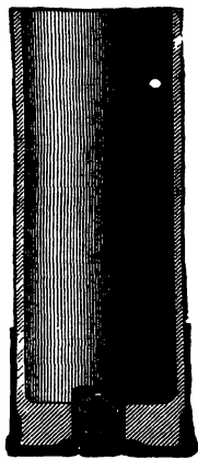
Section of the Patent Bailey Case, and View of Gas-tight Base.
