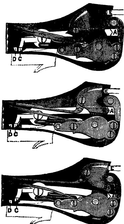
Scott's Automatic Intercepting Safety Bolt.
