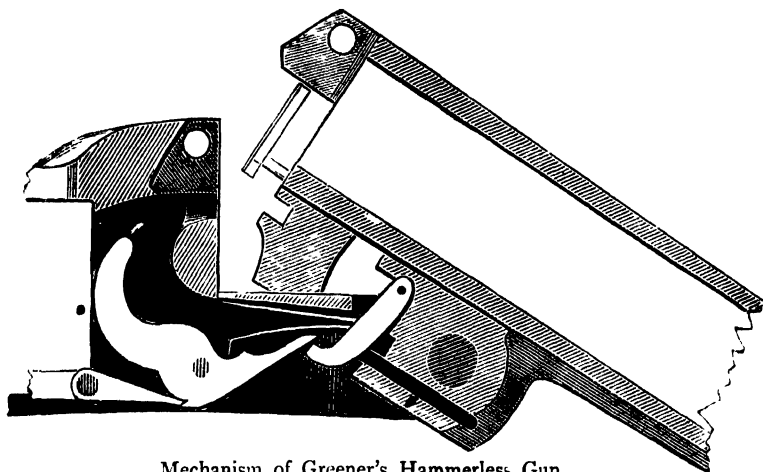
Mechanism of Greener's Hammerless Gun.
