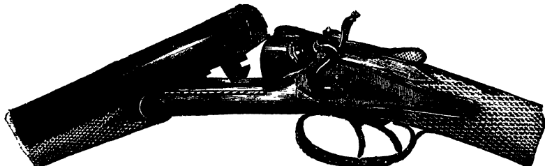
Top-Lever Gun, with Back-action Locks.
