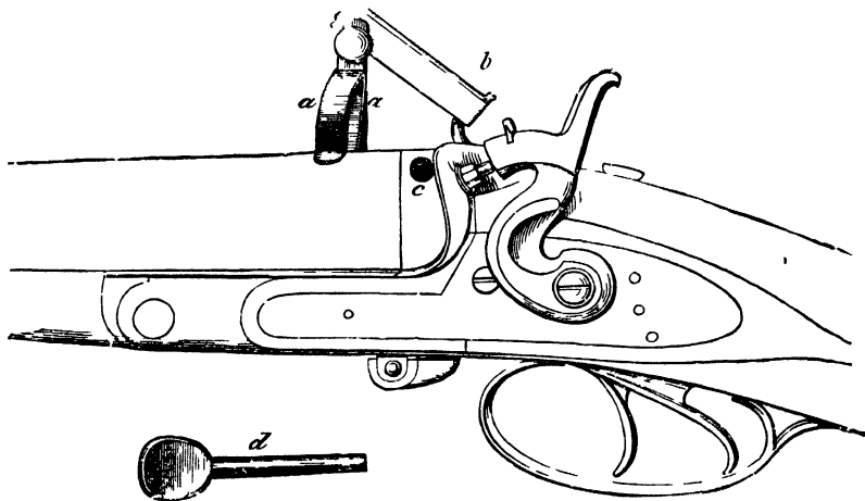
Experimental Breech-Action.
