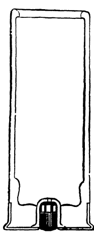
Section of the Central-fire Cartridge Case (Eley's).
