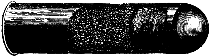
8-BORE BRASS CARTRIDGE FOR ELEPHANT RIFLE.
