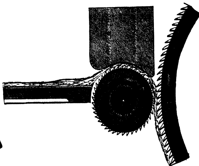
Fig. 119.—Tatham's Improved Feed Roller.
