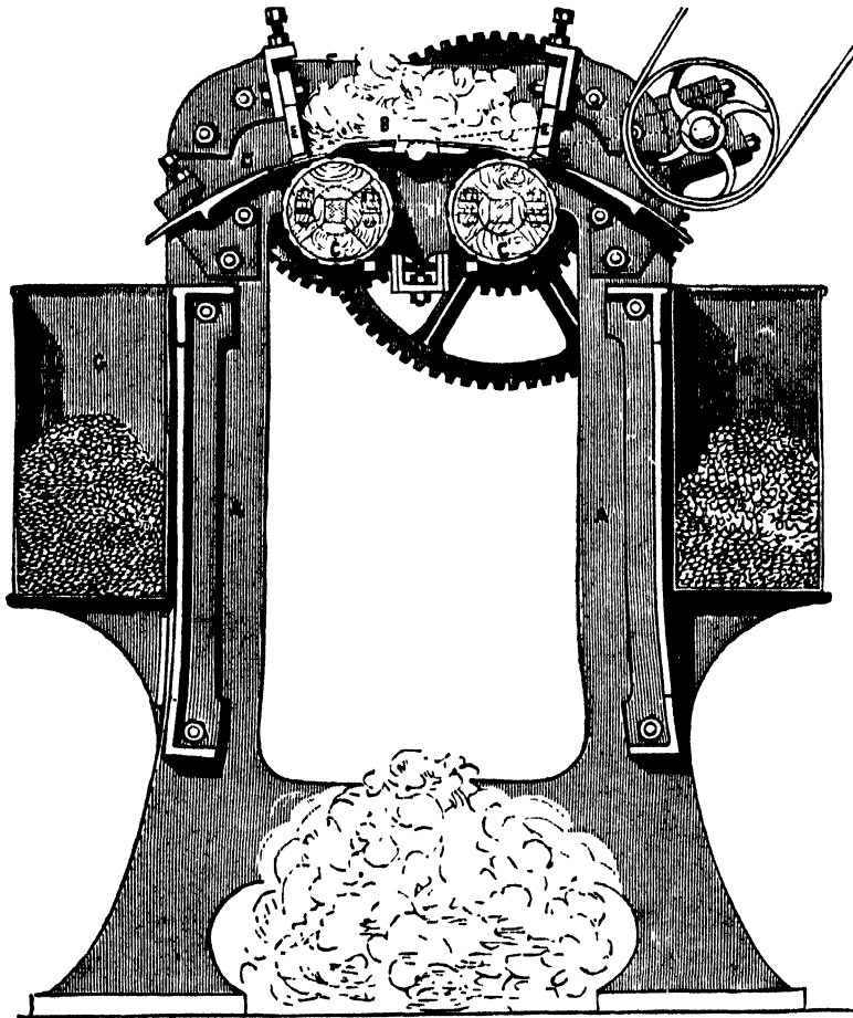
Fig. 20.—The Double Macarthy Gin. (E. & F. A. Leigh's Patent.)
