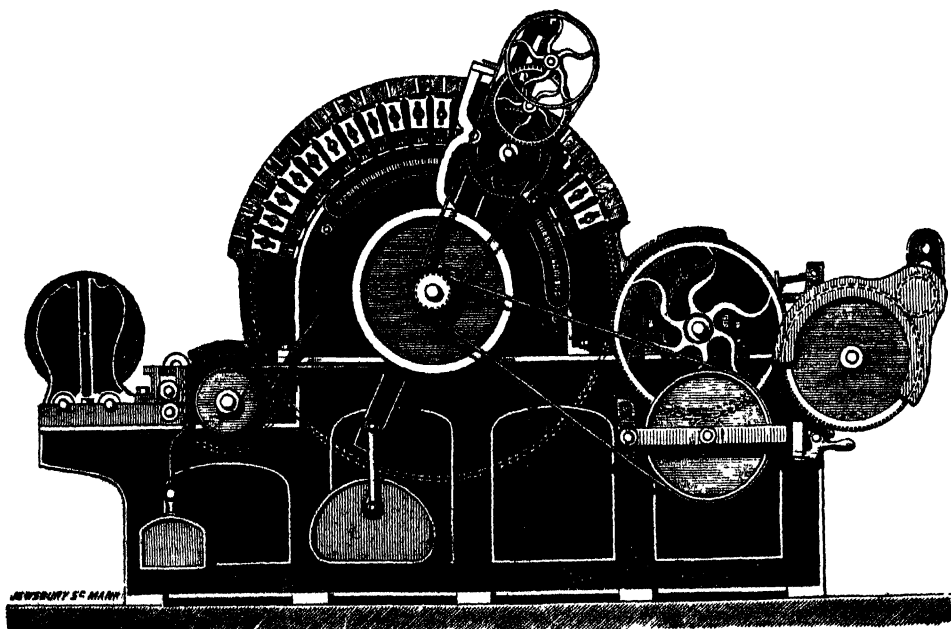
Fig. 115.—Wellman Card, by Dobson and Barlow. (Scale \frac{1}{4} inch=1 foot.)
