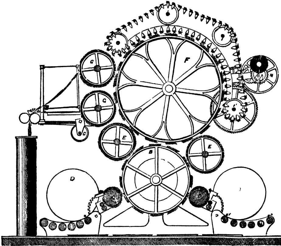
Fig. 90.—Smith's Self-stripping Carding Engine.
