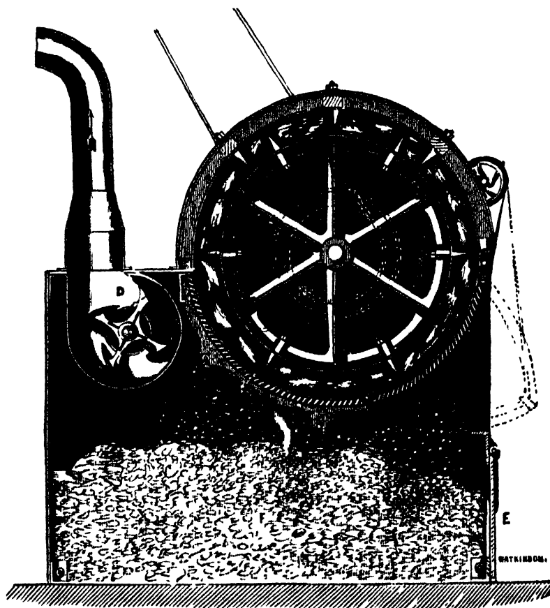
Fig. 34. —The Oldham Willow (1).
