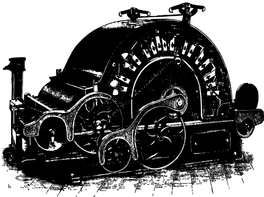
Fig. 69.—Single Roller Carding Engine, as made by John Tatham.
