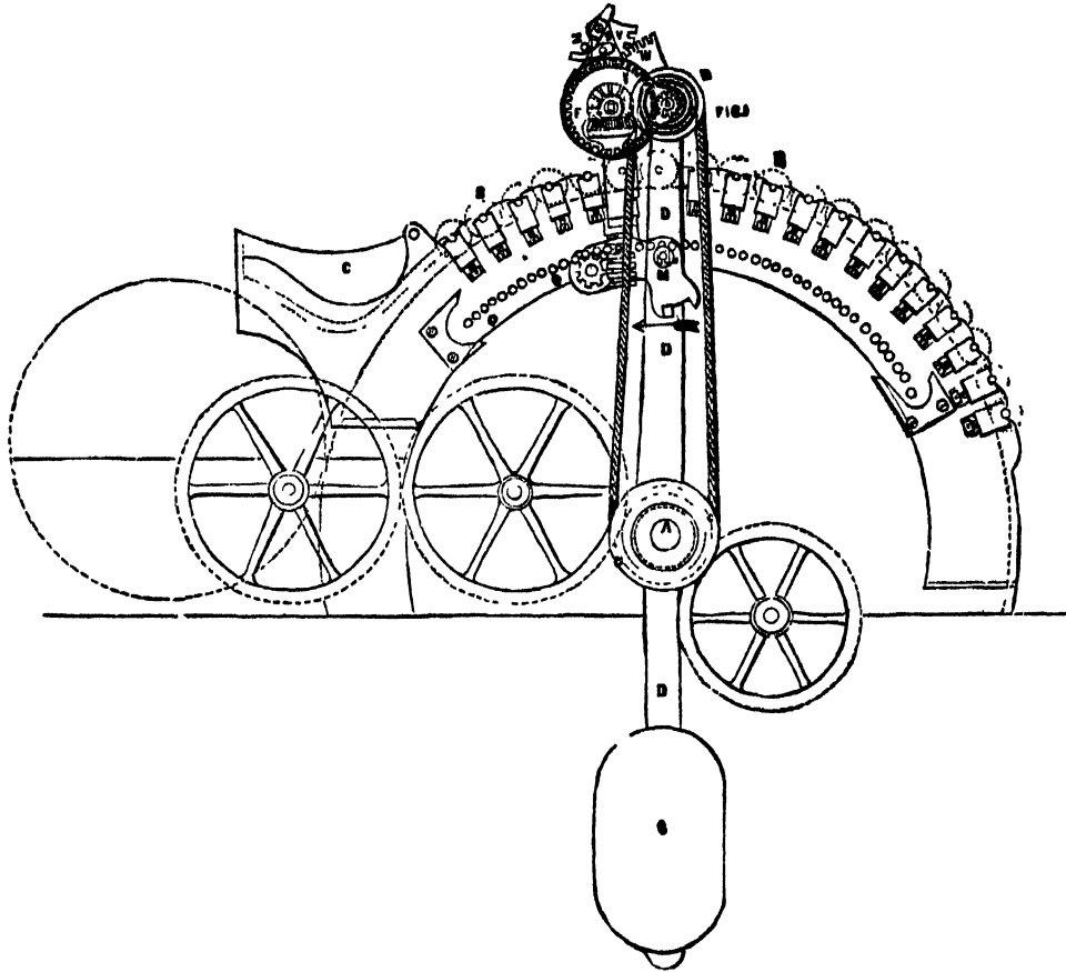
Fig. 78.—Robert Wilkinson's Patent (Scale \frac{1}{2} inch = 1 foot).
