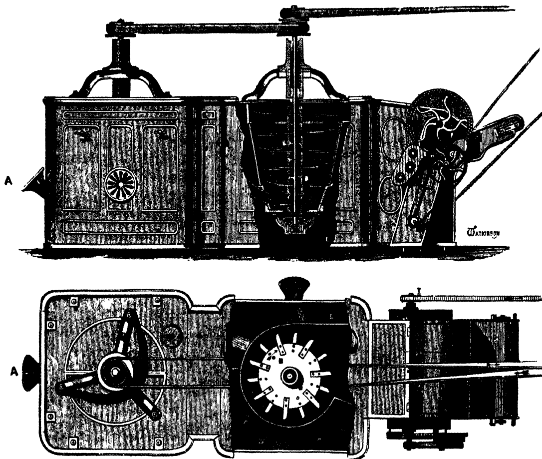
Figs. 36 and 37.—Crighton's Cotton Opener.
