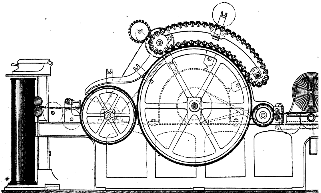
Fig. 110.—Section of Finisher Carding Engine (Leigh's Fourth Patent.)
