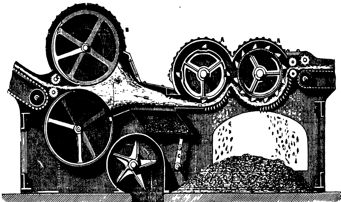
Fig. 43.—The Porcupine Opener.
