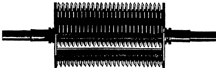
Fig. 44. Cylinder of Porcupine Opener.
