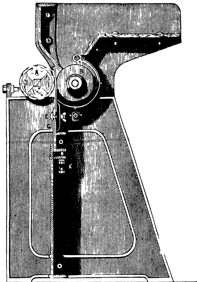
Fig 21.—The Knife Roller Gin.
