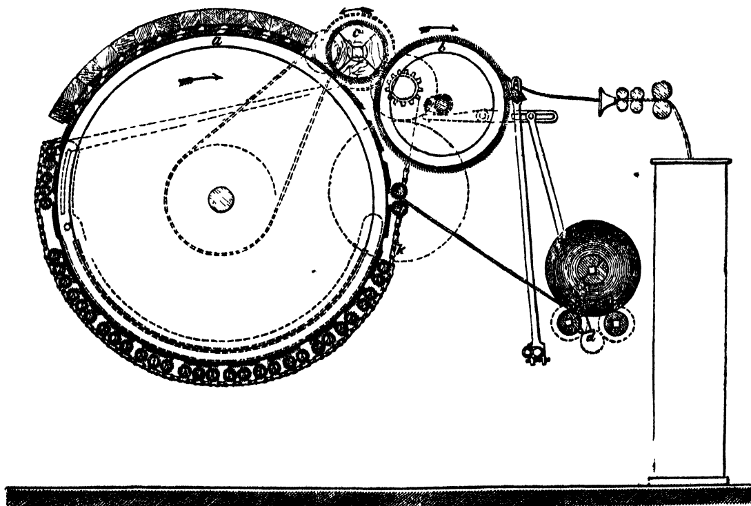
Fig. 77.—Pooley's Patent Card.
