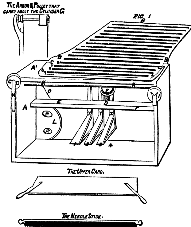
Fig. 65.—Paul's Carding Engine (No. 1)
