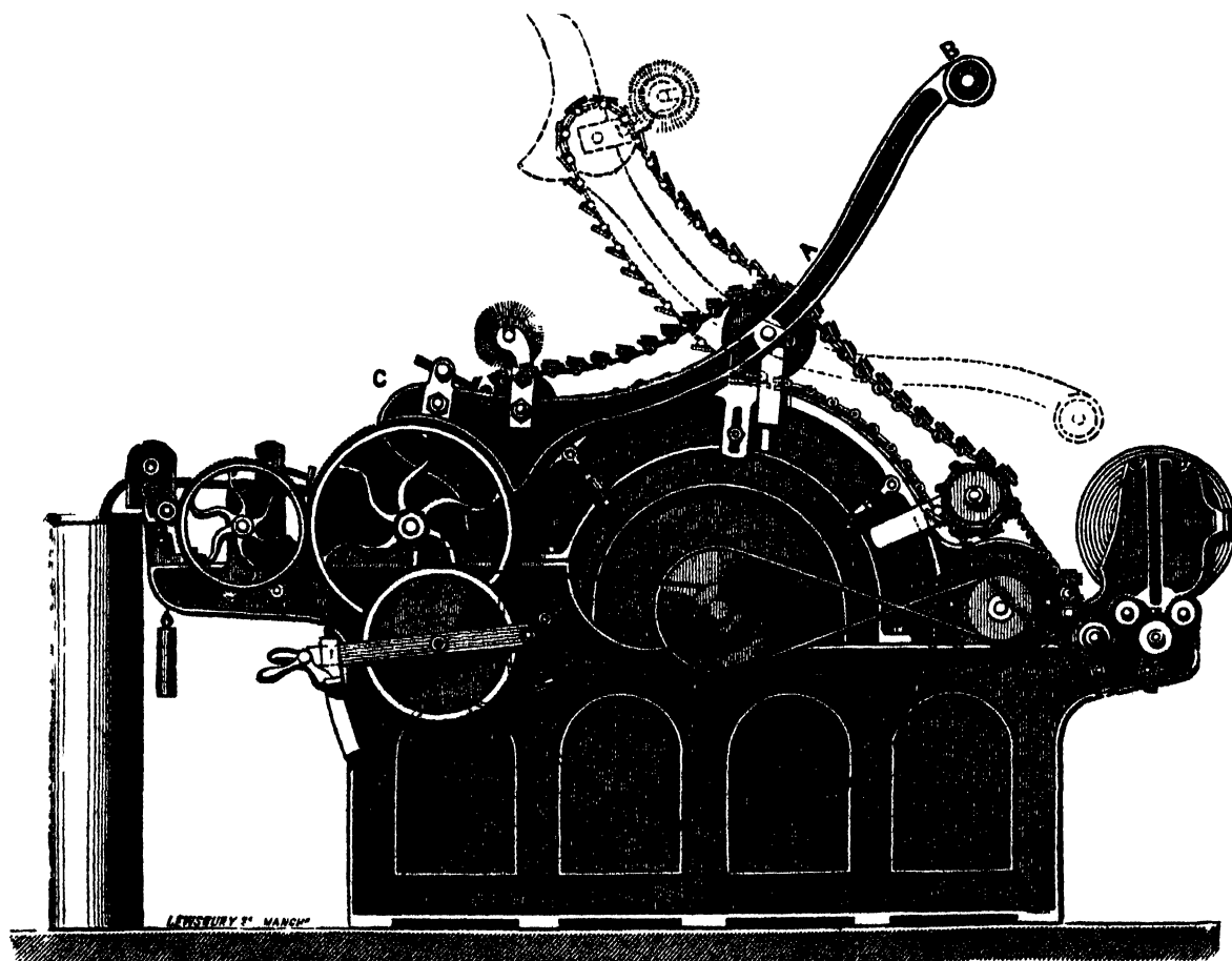
Fig. 105.—Finisher Card altered to Leigh's Self-stripper.
