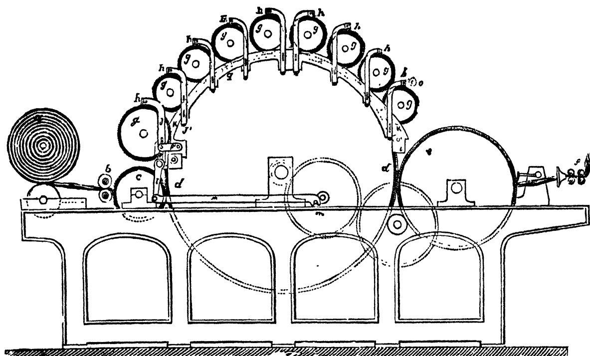
Fig. 79.—Adshead & Holden's Patent Roller Carding Engine (Scale \frac{1}{2} inch=1 foot).
