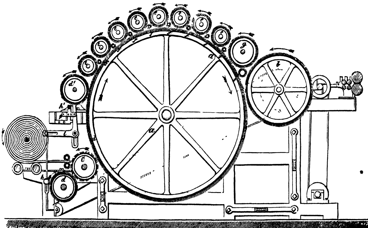
Fig. 72.—Birch's Roller Engine ( \frac{3}{4} of inch=1 foot)
