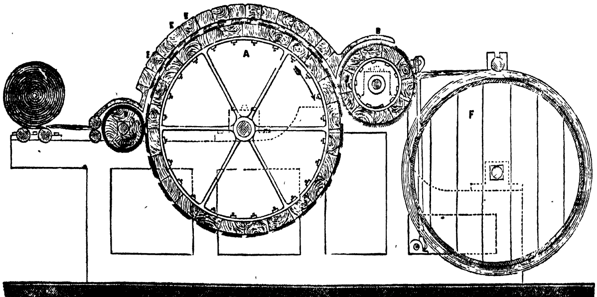
Fig. 83. —Breaker Carding Engine.
