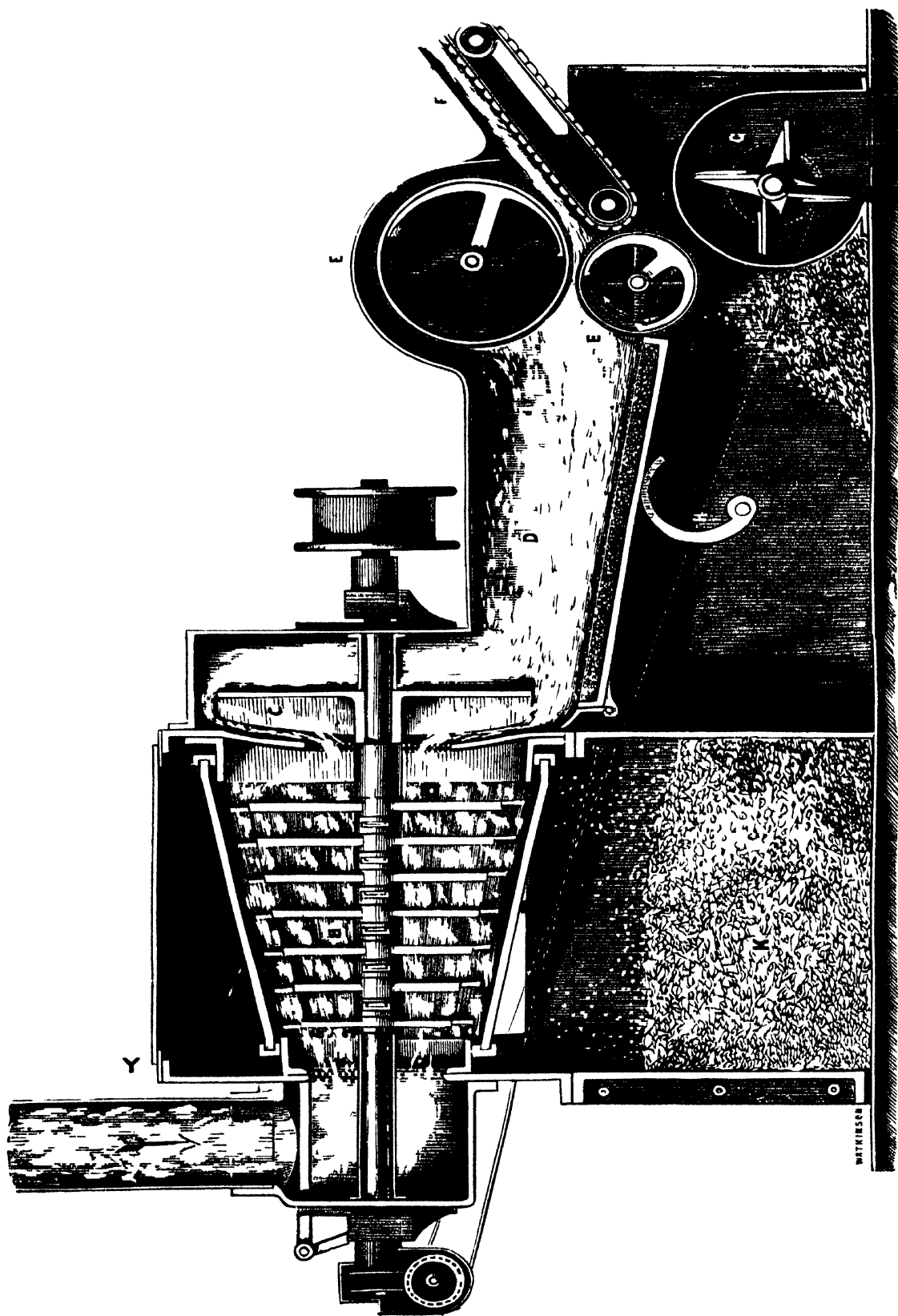
Fig. 39—Lord's Patent Cotton Opener
