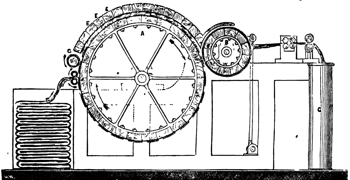
Fig. 85—Finisher Carding Engine.
