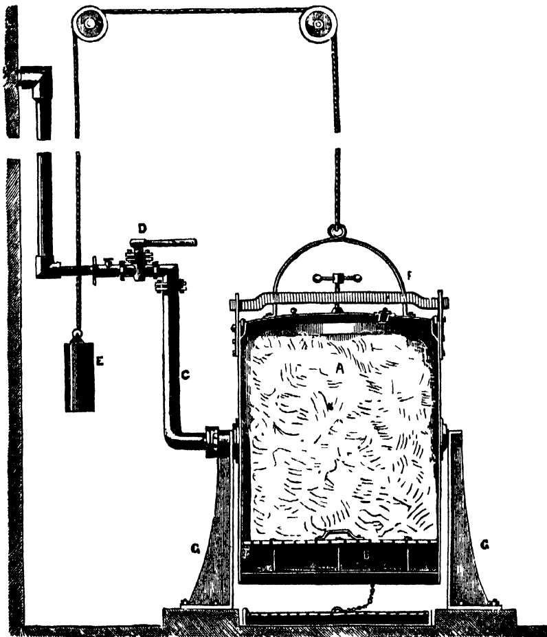
Fig. 38.—Cotton Steaming Apparatus.
