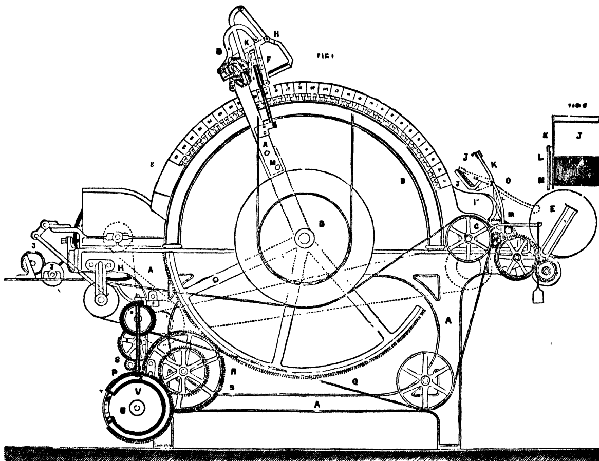
Fig. 100.—Wellman's Self-stripping Card. (Scale \frac{1}{2} inch = 1 foot.)
