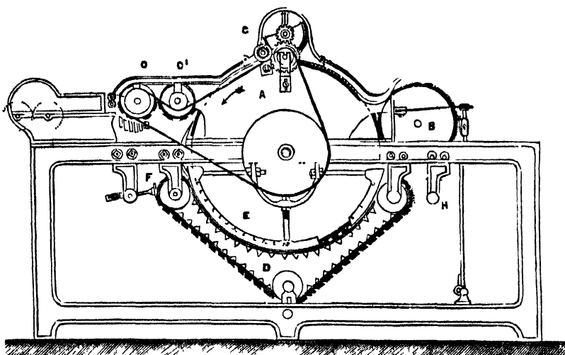
Fig. 92.—Leigh's Self stripping Card. (Scale \frac{1}{4} inch = 1 foot.)
