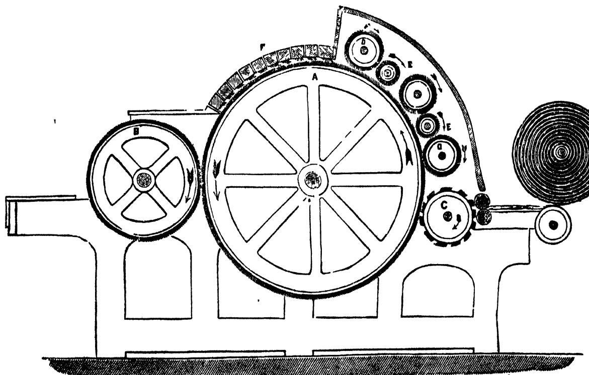
Fig. 80.—The Union Carding Engine.
