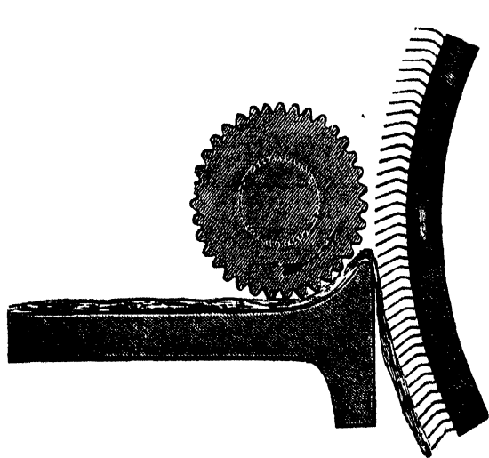
Fig. 118.—Bennett's Feed Roller (half size).
