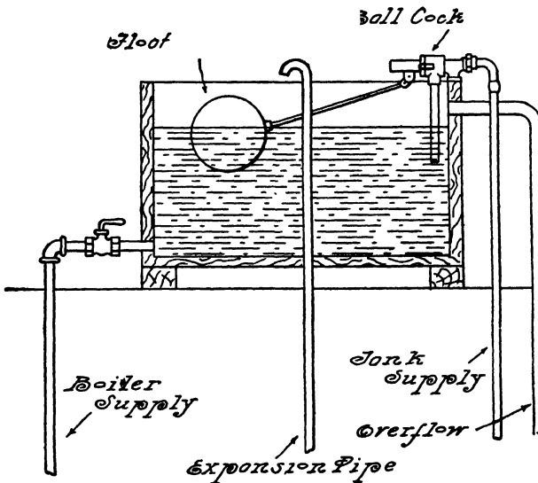
FIG. 254.—Attic Tank and Connections.
