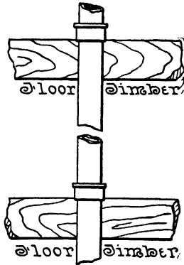
FIG. 79.—Vertical Line of Soil Pipe Supported by Hub at Each Floor.
