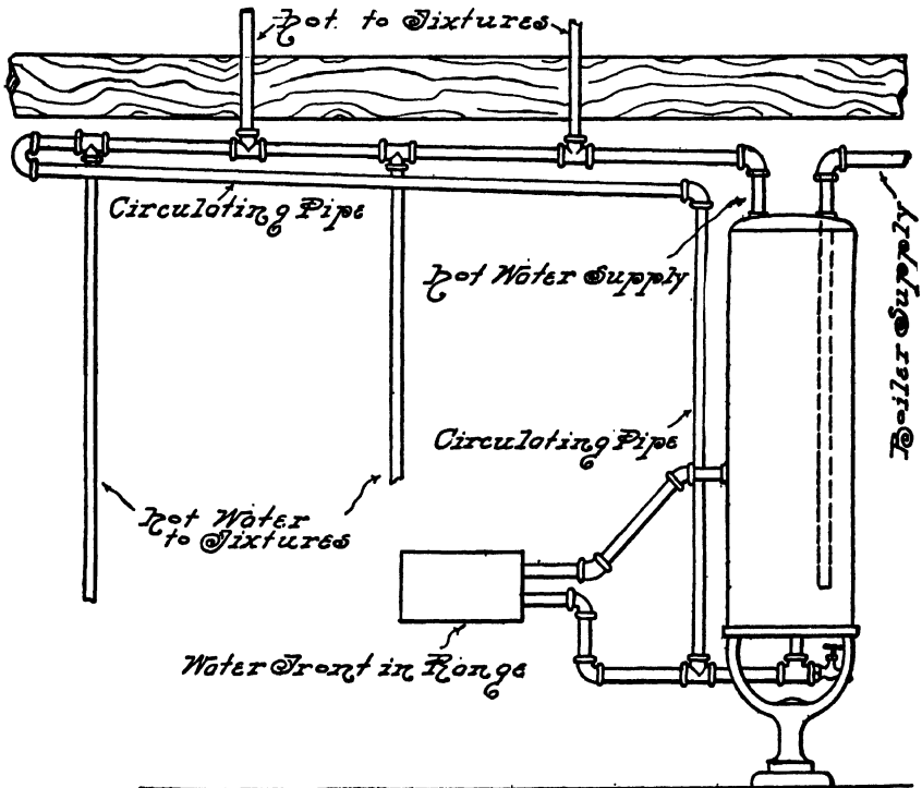
FIG. 291.—Circulation Applied to Fixtures of Small House.
