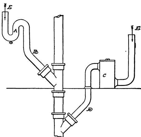
FIG. 35.—The Siphonage of Traps.
