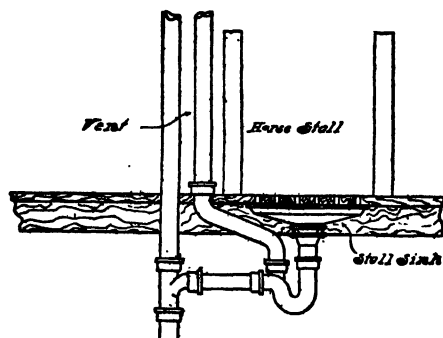
FIG. 214.—Plumbing for Horse Stall.
