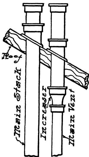
FIG. 52.—Main Vent and Main Stack Separately through Roof.
