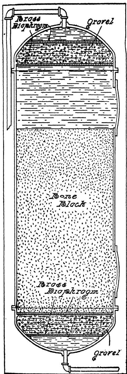
FIG. 233.—Pressure Filter; Use of Bone Black.
