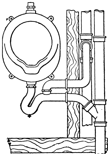
FIG. 197.—Connections for Urinal.
