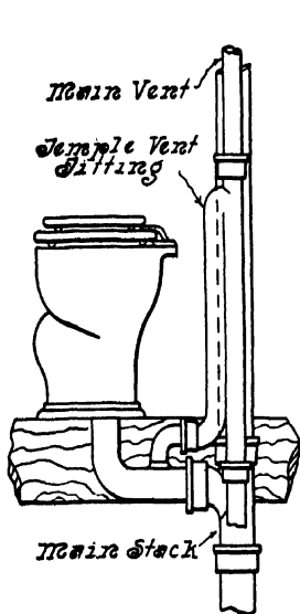
FIG. 147.—Water-Closet Vented into Temple Vent Fitting.
