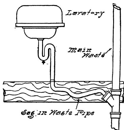
FIG. 117.—Double-Trapping Produced by Sagging of Waste Pipe.
