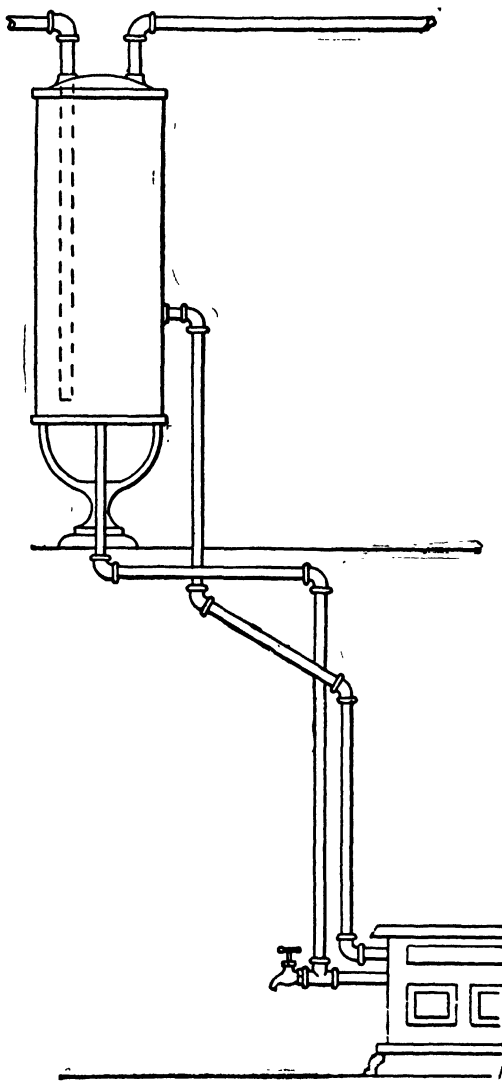
FIG. 302.—Range Boiler Heated by Range on Floor Below.
