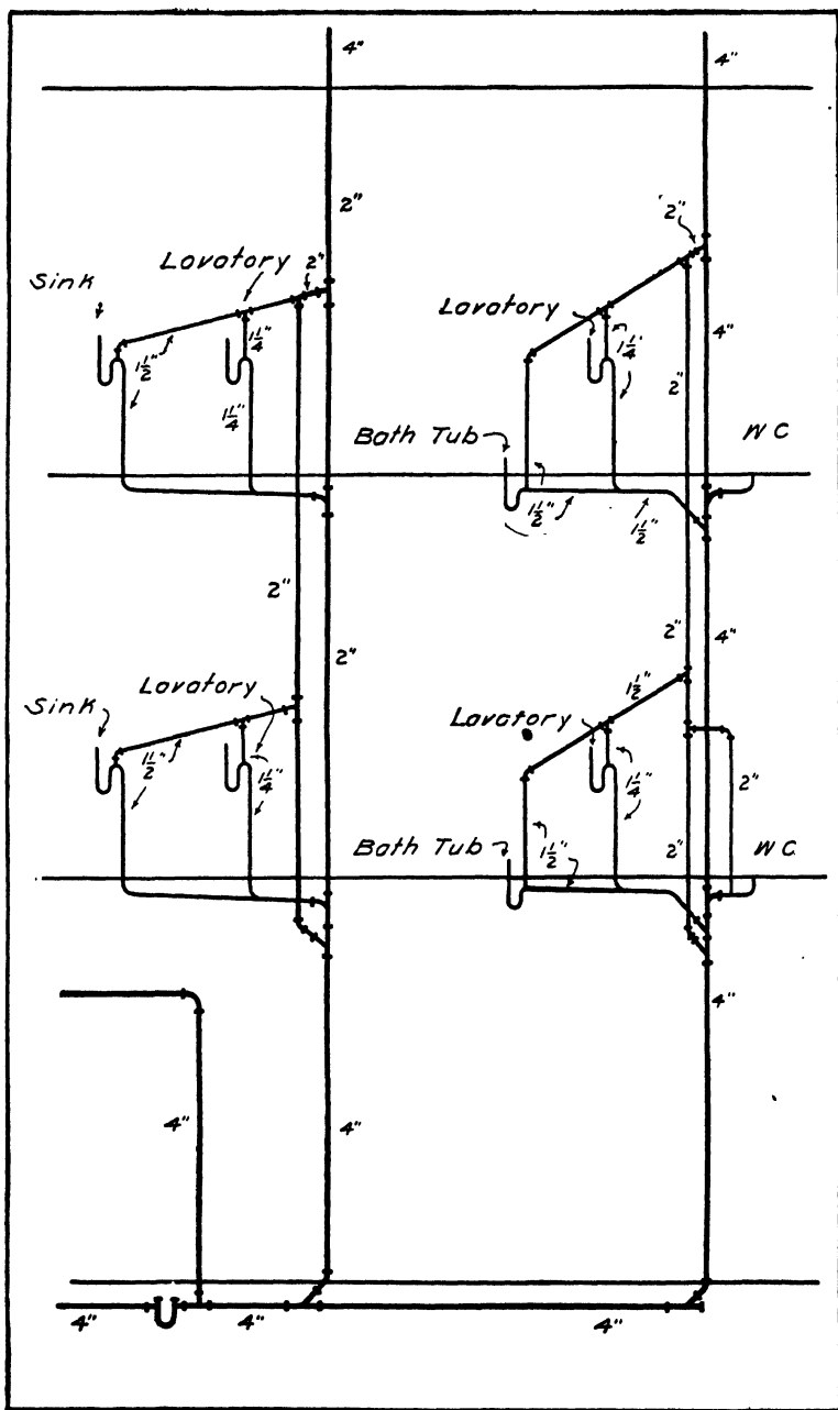
FIG. 340.—Single-Line Elevation of Plumbing System.
