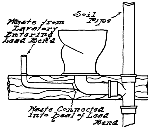
FIG. 156.—Waste Connected into Heel of Lead Bend.
