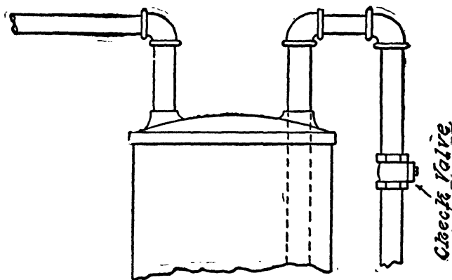
FIG. 258.—Wrong Use of Check Valve to Prevent Siphonage.
