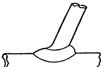
FIG. 9.—Poorly Shaped Wiped Joints.
