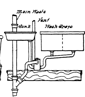
FIG. 121.—Sink and Wash Trays Connected into Drum Trap.—Poor Practice.
