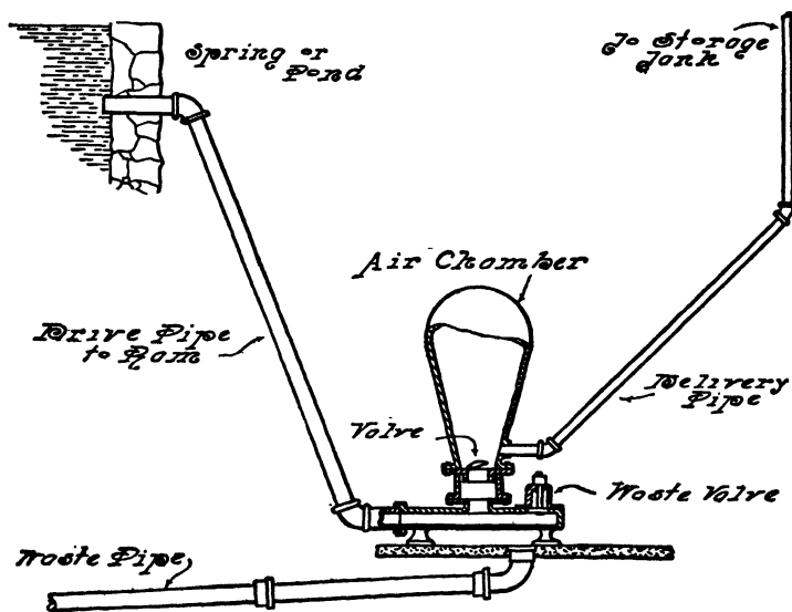
FIG. 228.—The Hydraulic Ram and Its Connection.
