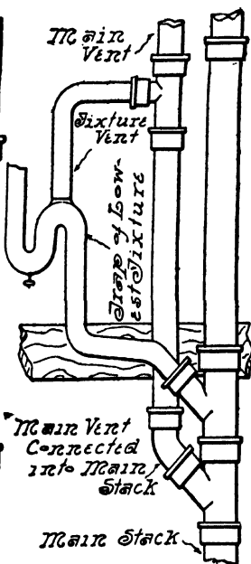
FIG. 57.—Improved Lower Connection of Main Vent into Main Stack.
