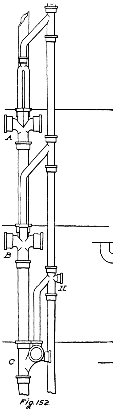
FIGS. 152-155.—The Use of Special Water-Closet Waste and Vent Fittings.
