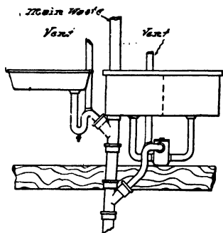
FIG. 190.—Connections for Kitchen Sink and Laundry Tubs.
