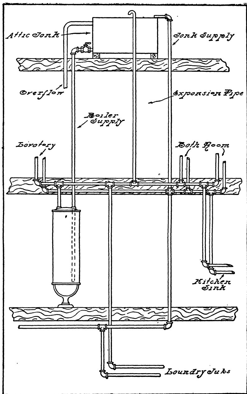
FIG. 255.—Tank System of Supply for Residence
