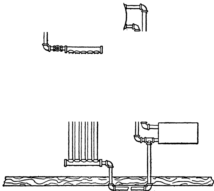
FIG. 329.—Wall Coil and Fixtures of Apartment Supplied by Horizontal Boiler.
