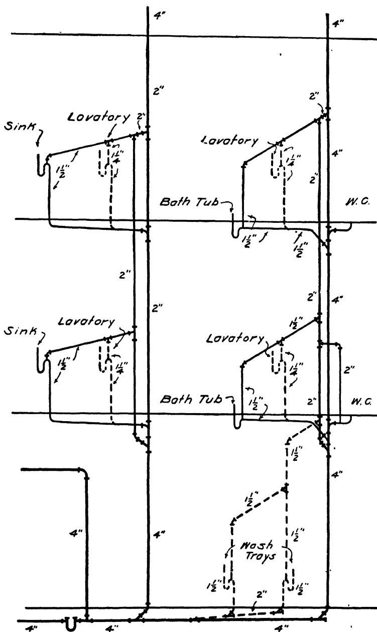
FIG. 341.—Single-Line Elevation Showing Changes on Old Plumbing System.
