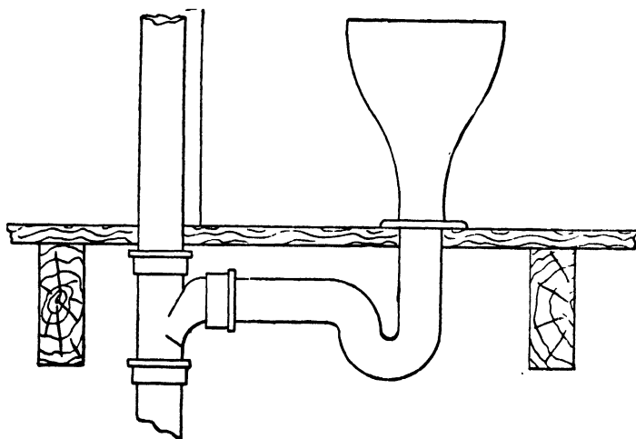
FIG. 128.—The Long Hopper Closet.
