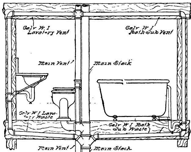
FIG. 201.—Bath-Room Connections, Durham System; Galvanized Wrought-Iron Wastes and Vents.
