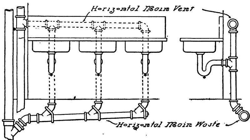
FIG. 62.—Continuous Venting for Line of Fixtures.
