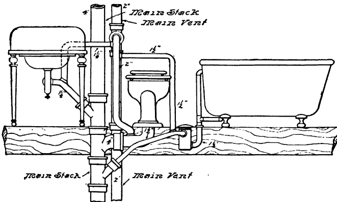
FIG. 183.—Connections for Bath Room. Separate Entrance into Stack for Each Fixture.
