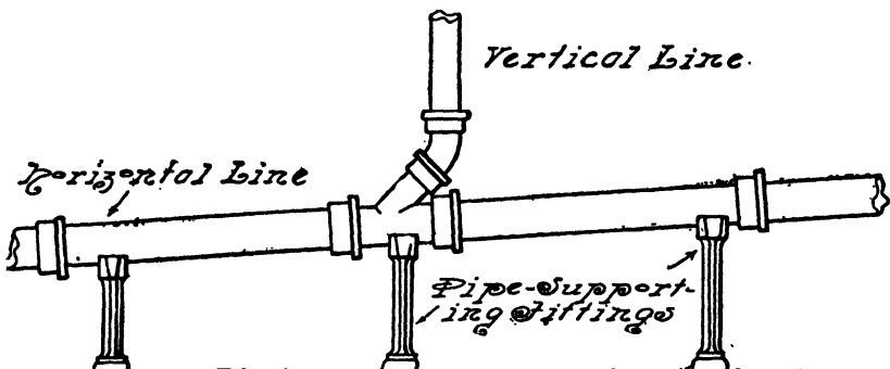
FIG. 108.—Horizontal Line of Pipe Supported by Pipe-Supporting Fittings.
