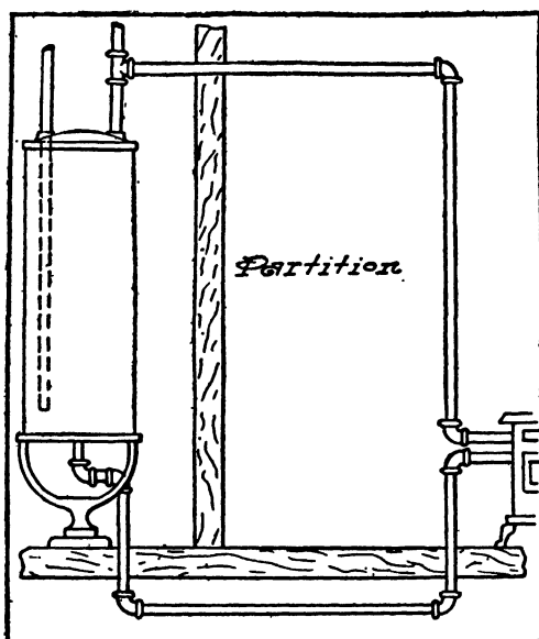
FIG. 301.—Boiler Heated by Range in Adjoining Room.
