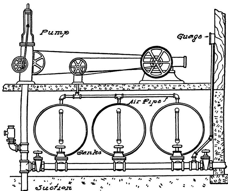
FIG. 227.—Pneumatic Public Water Supply.
