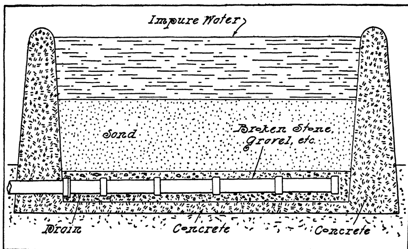
FIG. 236.—Sand Filter Bed.
