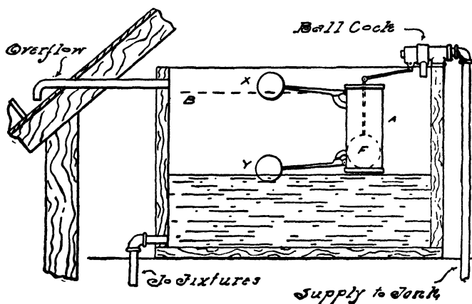
FIG. 325.—Automatic Storage Tank.
