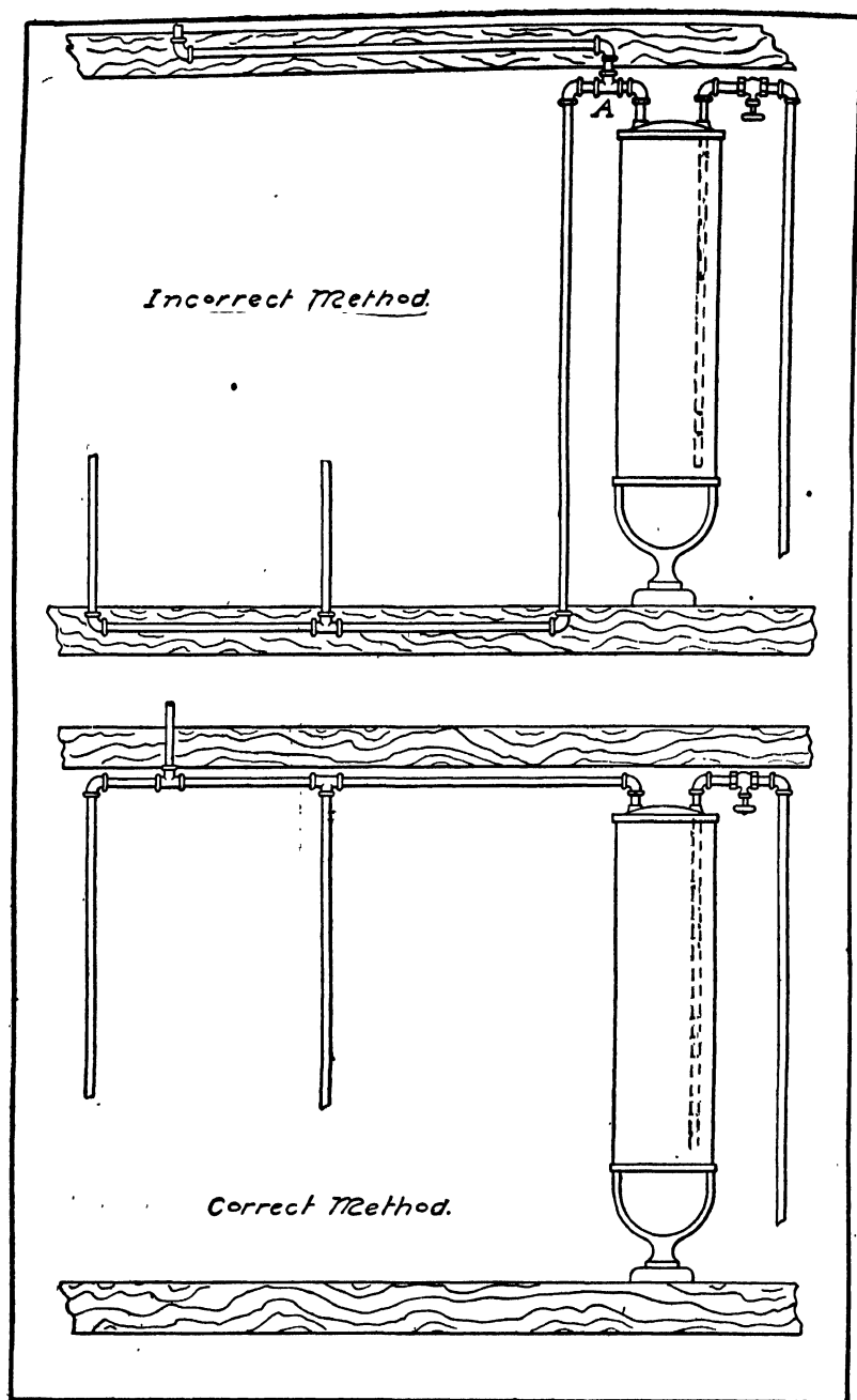
FIG. 284.—Method of Running Hot-Water Pipes.
