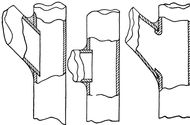
FIG. 15.—Wrong Methods of Making Wiped Joints.
