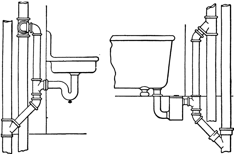
FIG. 61.—The Continuous Vent.
