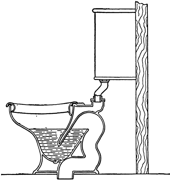
FIG. 134.—The Siphon-Jet, Low-Down Water-Closet.
