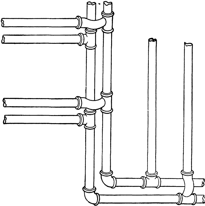
FIG. 265.—Use of Straddle Fittings.
