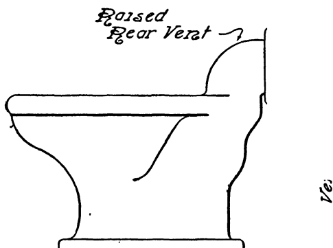
FIG. 165.—Water-Closet with Raised Rear Vent.
