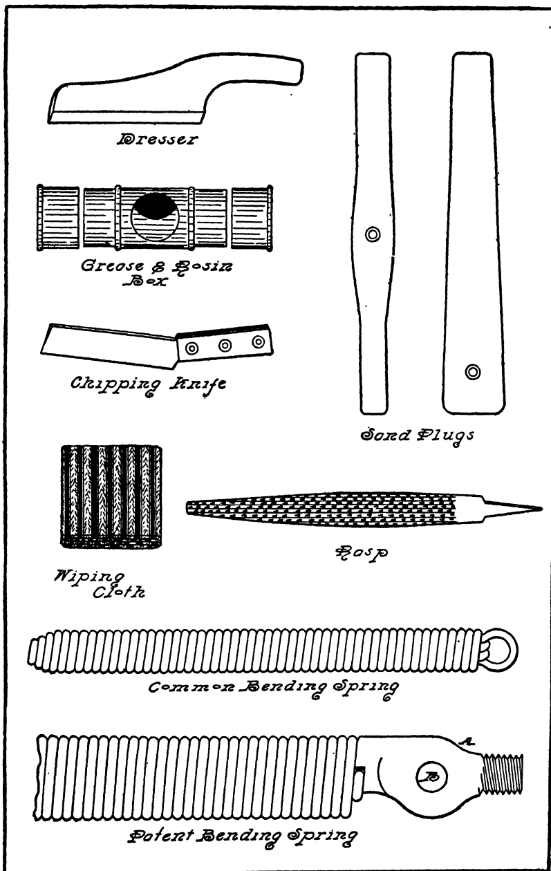
FIG. 2.—A Few of the Plumber's Tools.
