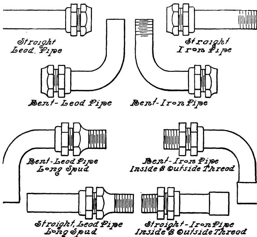
FIG. 282.—Water Back Couplings.
