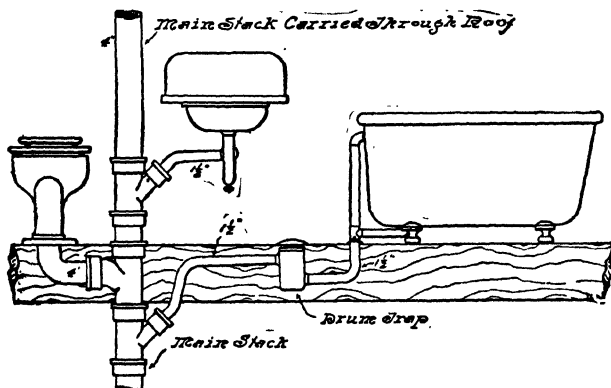
FIG. 124.—Separate Waste Entrance for Each Fixture.
