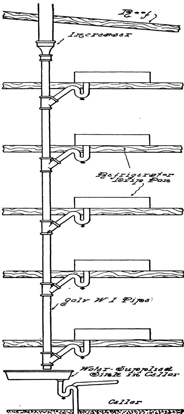
FIG. 213.—Connections for Line of Refrigerators on Different Floors.
