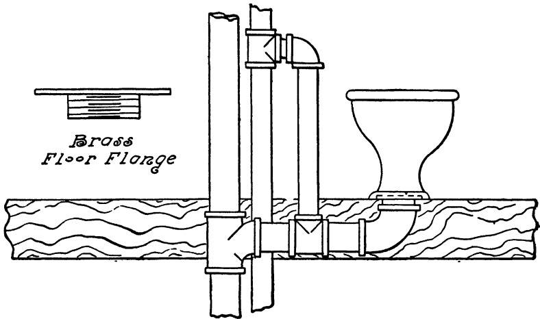
FIG. 137.—Connections of Water-Closet on the Durham System.
