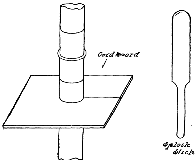
FIG. 14.—Wiping of Upright Joints.
