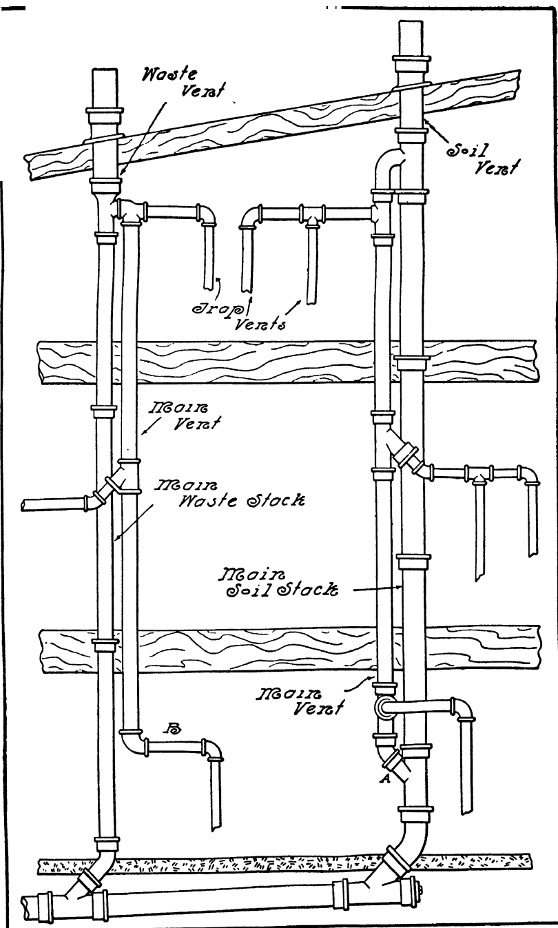
FIG. 59.—Vent System, Showing Main and Trap Vents, Use of Fittings, etc.
