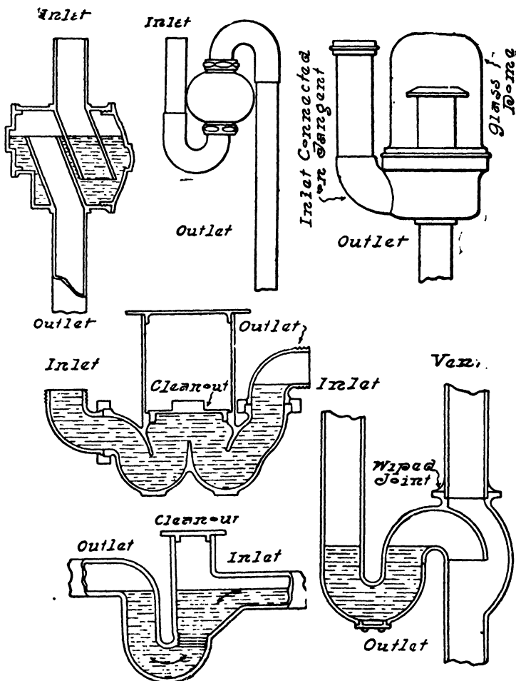
FIG. 30.—Various Patented Forms of Traps.
