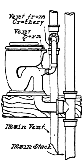
FIG. 140.—Water-Closet Vented from the Bowl.
