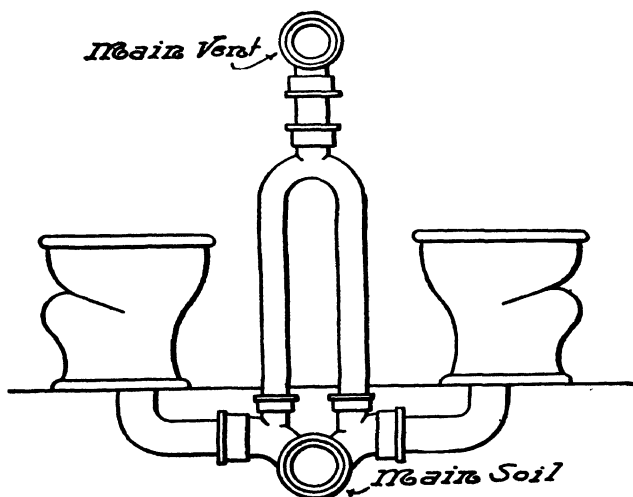
FIG. 177.—Special Fitting for Double Line of Water-Closets.
