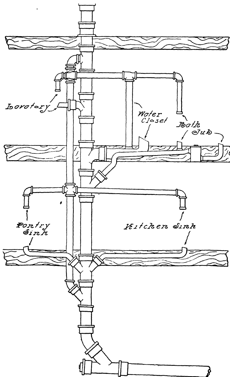
FIG. 110.—Soil Pipe Stack Ready for Water Test.
