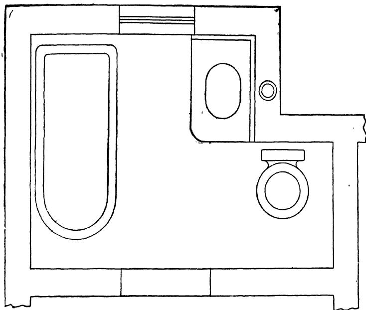
FIG. 91.—Floor Plan of Bath Room.
