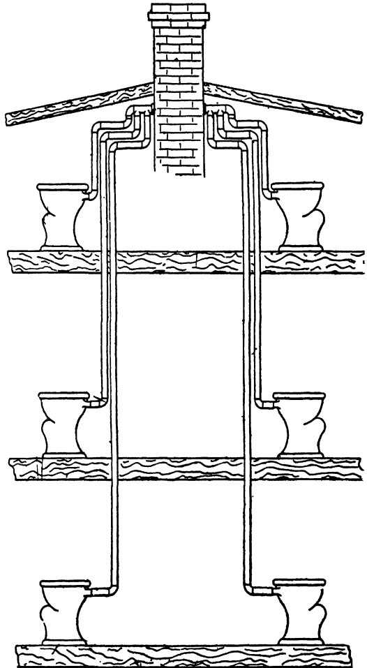
FIG. 162.—Good Method of Constructing Local Vents.
