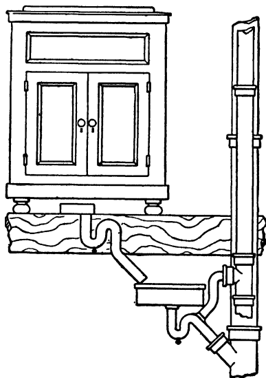
FIG. 192.—Proper Refrigerator Connections.
