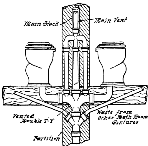
FIG. 150.—Waste and Vent for Water-Closets on Opposite Sides of Partition.
