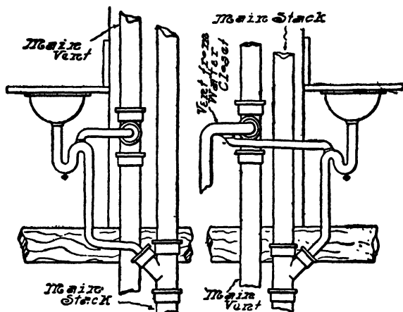
FIGS. 42, 43.—Wrong Connection of Vent.
