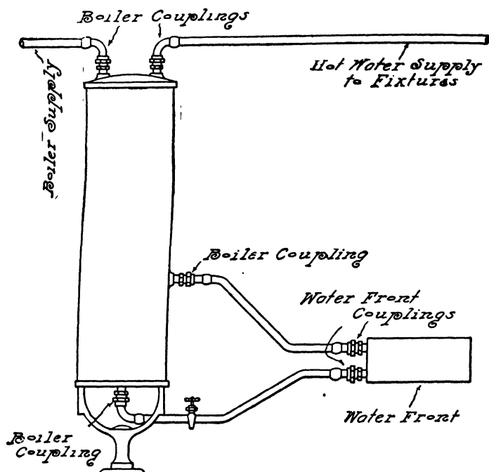
FIG. 279.—Lead Pipe Range and Boiler Connections.
