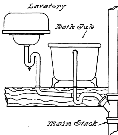
FIG. 118.—Lavatory Double-Trapped.
