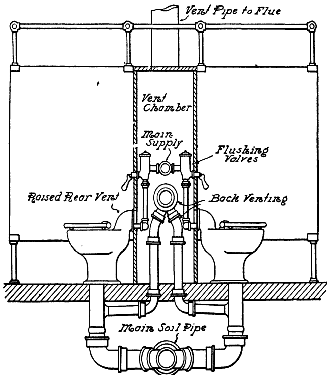
FIG. 171.—End View of Local Vent System for Double Line of Water-Closets.
