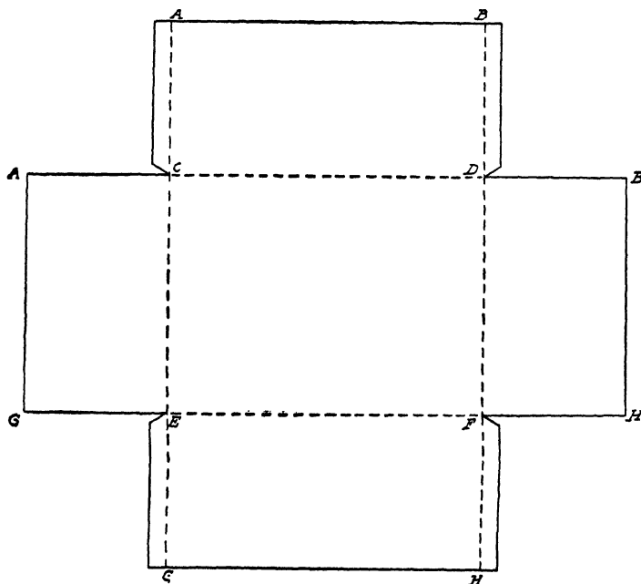
FIG. 20.—Layout of Lead or Copper Lining for Tank.
