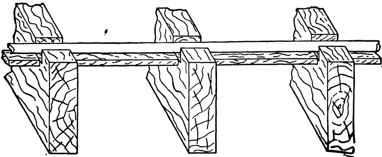
FIG. 23.—Supporting of Lead Pipe between Timbers.
