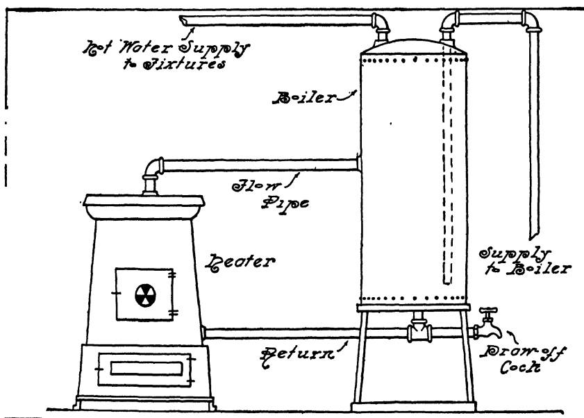
FIG. 310.—Connections for Vertical Boiler and Tank Heater.
