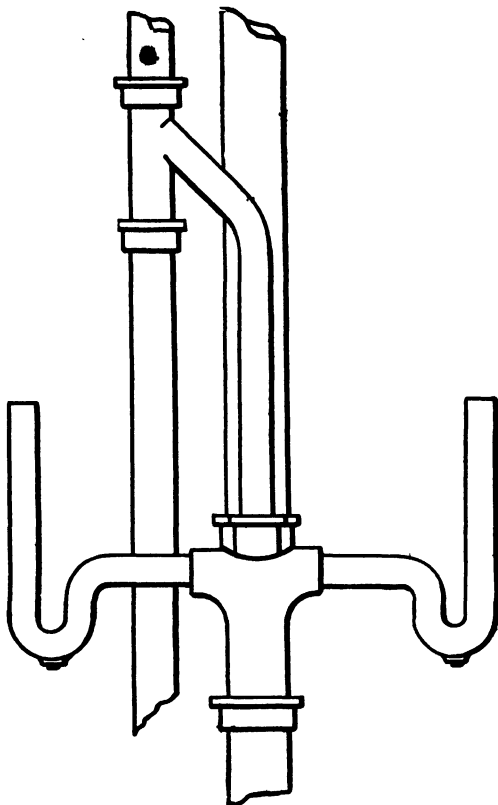
FIG. 175.—Use of Vented Cross.
