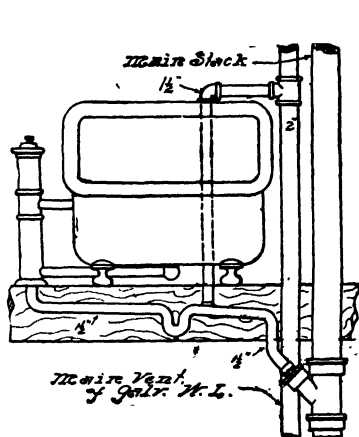
FIG. 184.—Connections for Sitz Bath.
