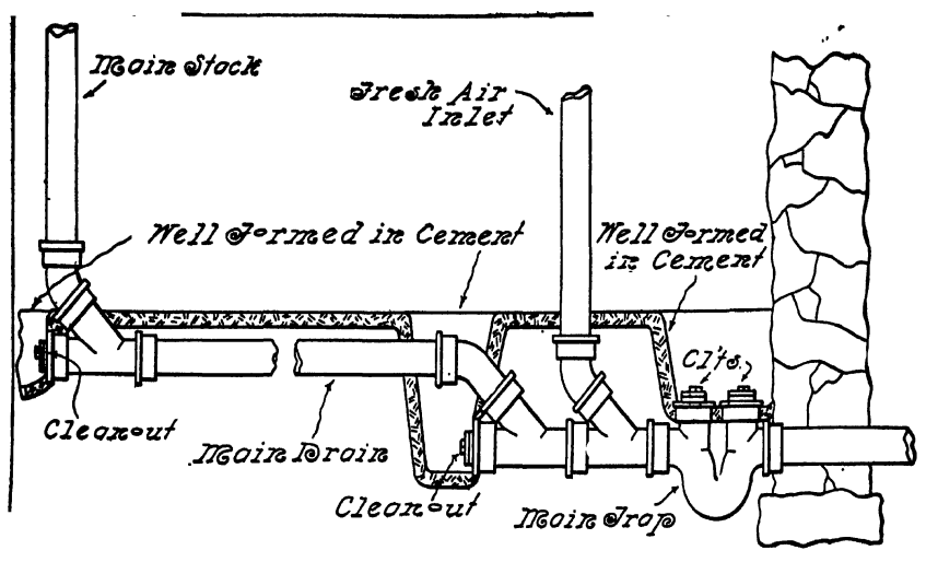
FIG. 102.—Good Method of Running House Drain Underground.
