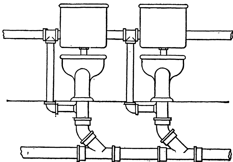
FIG. 138.—Connections for Line of Water-Closets.
