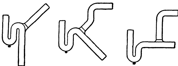
FIG. 44.—Venting of S-Traps.
