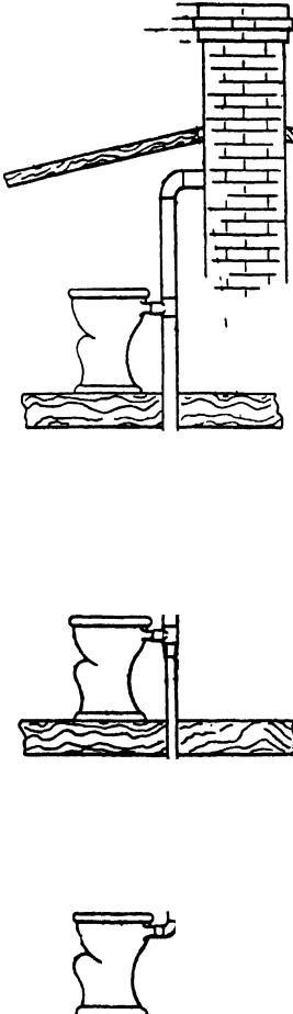
FIG. 161.—Common Method of Constructing Local Vents.
