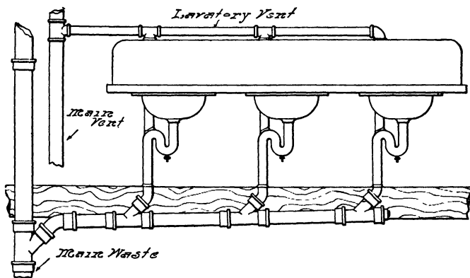
FIG. 196.—Proper Connections for Line of Lavatories.
