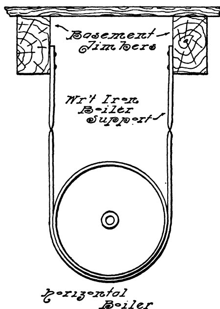
FIG. 312.—Supporting of Horizontal Boiler.
