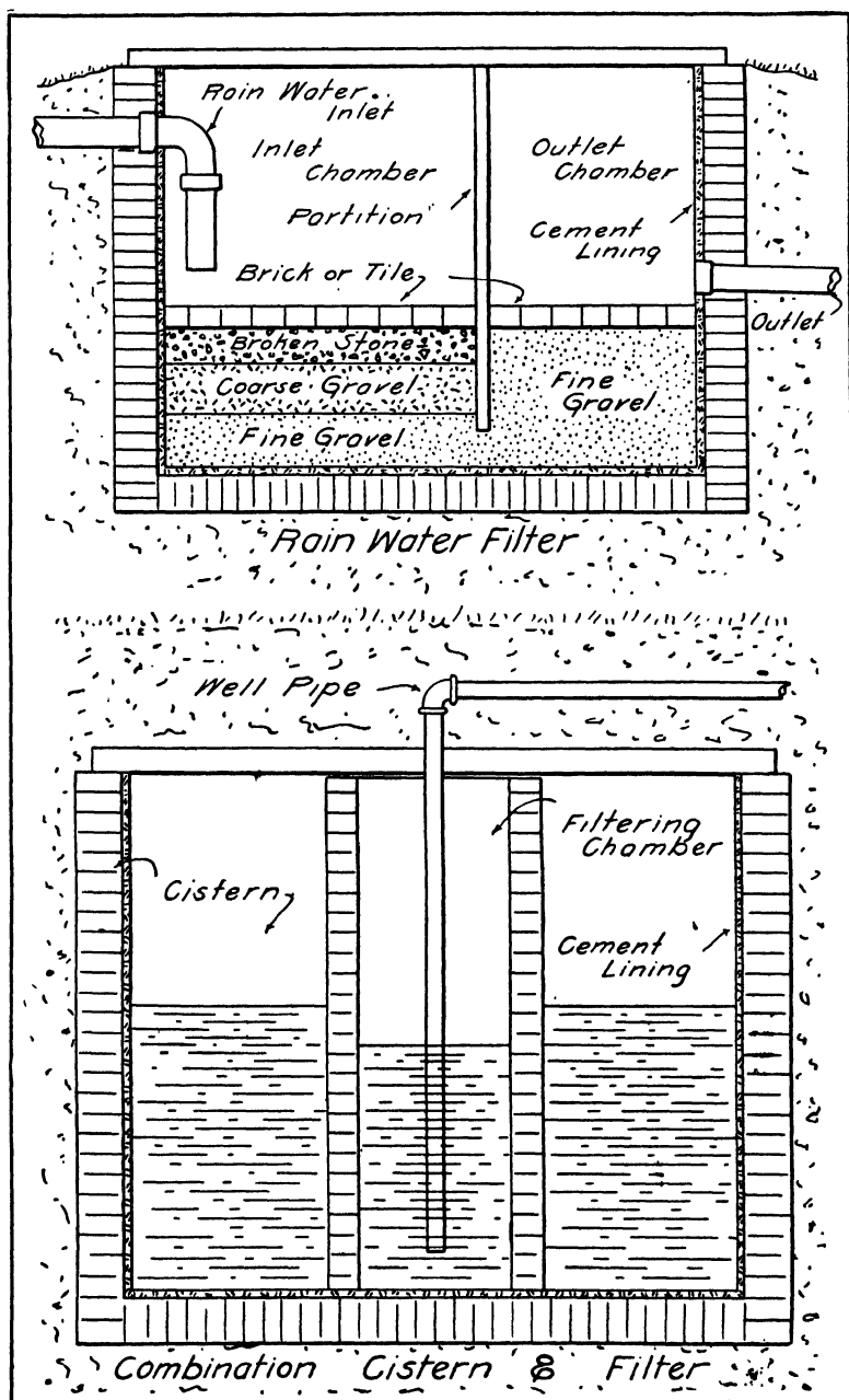
FIG. 245.—Cistern Filters.
