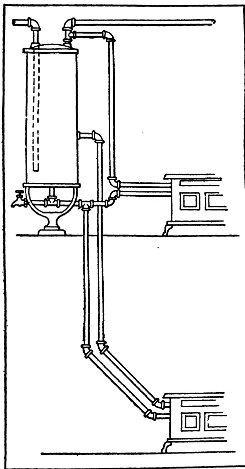
FIG. 306.—Range Boiler Heated by Two Ranges on Different Floors. Method No. 4.
