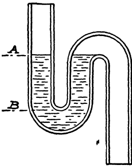
FIG. 32.—The Trap Seal.
