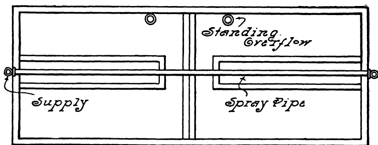
FIG. 207.—Plan View of Factory Wash Sink.
