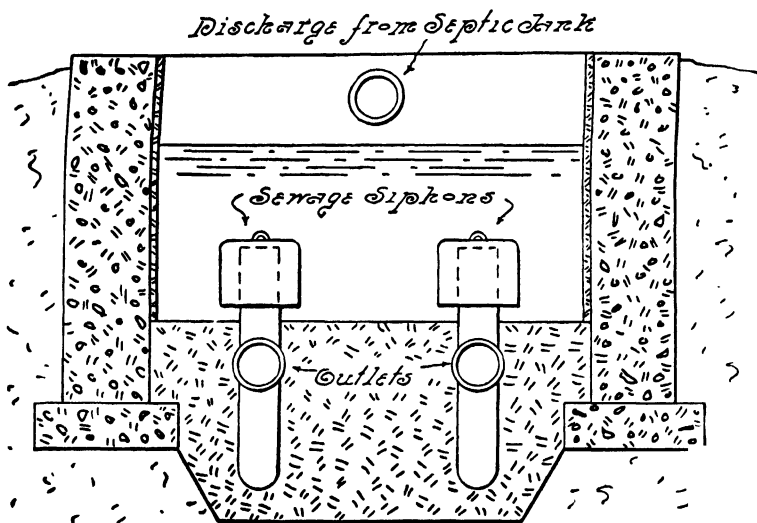
FIG. 224.—Sewage Siphons for Large Work.
