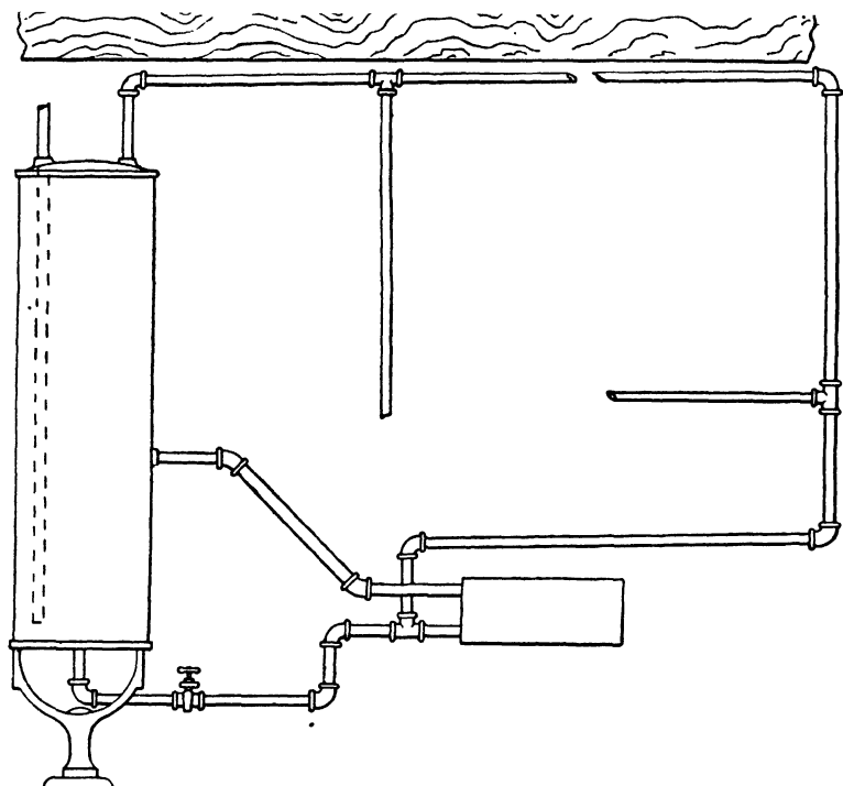
FIG. 288.—Use of Circulating Pipe.
