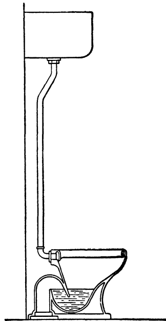
FIG. 131.—The Washdown Water-Closet.
