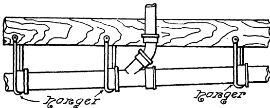
FIG. 104.—The Use of Hangers in Supporting Horizontal Pipe.
