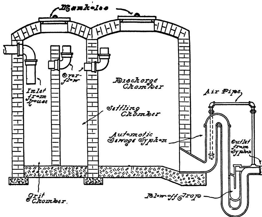
FIG. 222.—Septic Tank and Automatic Sewage Siphon.
