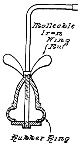
FIG. 84.—Testing Plug
