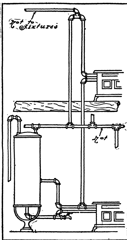
FIG. 308.—Boiler Heated by Range on Same Floor and Range on Floor Above.
