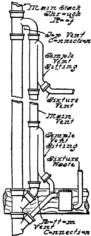
FIG. 55.—Showing Top and Bottom Vent Connections and Temple Vent Fittings.
