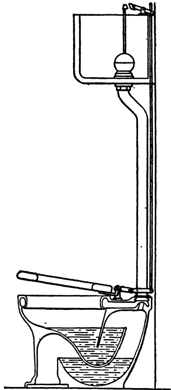
FIG. 133.—The Siphon Water-Closet.
