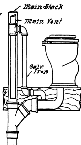
FIG. 149.—Venting of Water-Closet with Wrought Iron Pipe.
