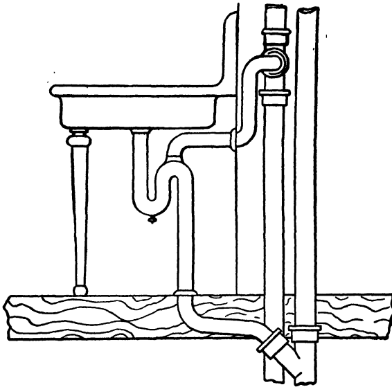
FIG. 41.—The Trap Vent.
