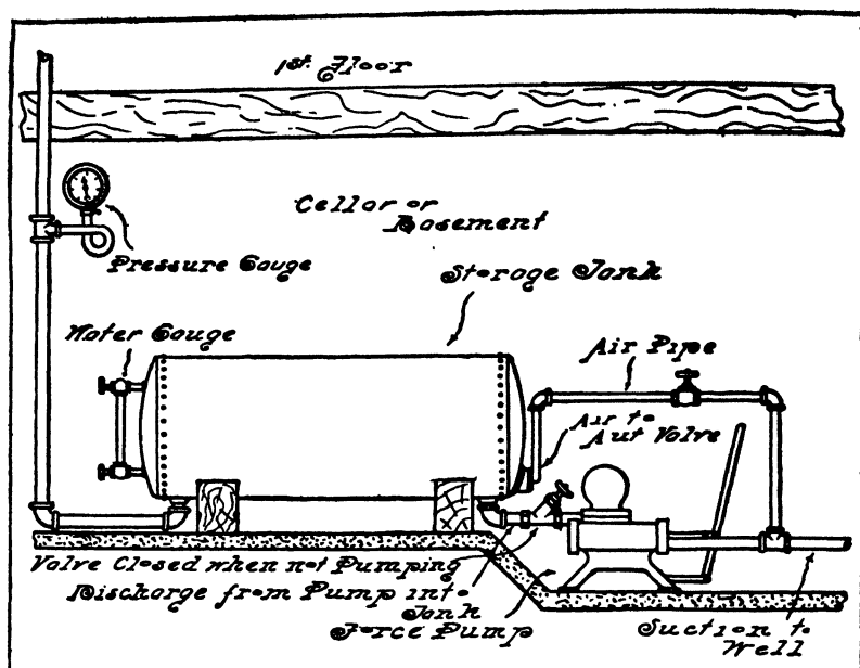
FIG. 226.—The Pneumatic System of Water Supply for Country Use.
