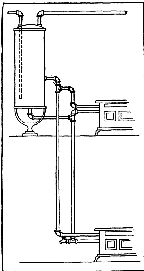
FIG. 303.—Range Boiler Heated by Two Ranges on Different Floors. Method No. 1.
