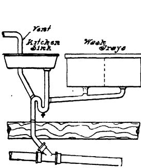
FIG. 119.—Kitchen Sink and Wash Trays Served by One Trap.—Poor Practice.
