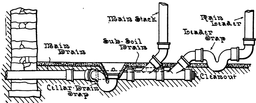
FIG. 81.—The House Drain and Its Connections.
