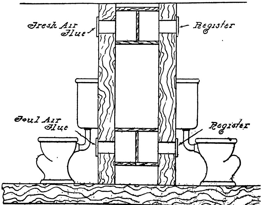
FIG. 164.—A Common Method of Ventilating Public Toilet Rooms.
