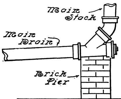
FIG. 107.—Vertical Line of Pipe Supported by Pier.
