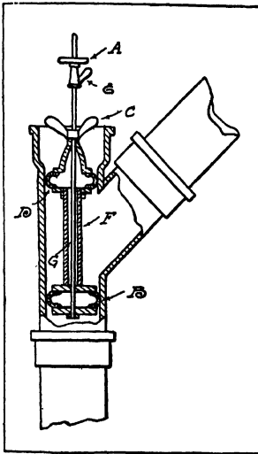
FIG. 85.—The Double Testing Plug.
