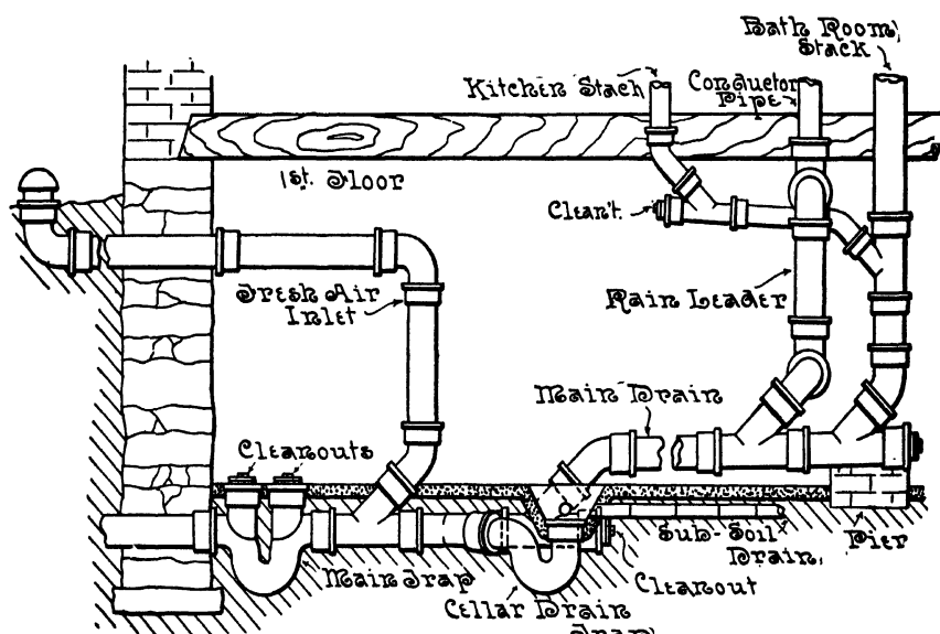
FIG. 80.—The House Drain and Its Connections.
