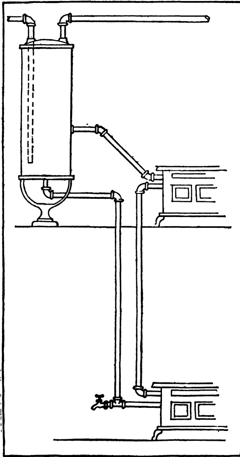
FIG. 305.—Range Boiler Heated by Two Ranges on Different Floors. Method No. 3.
