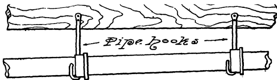
FIG. 105.—Poor Practice—Use of Pipe Hooks in Supporting Horizontal Pipe.
