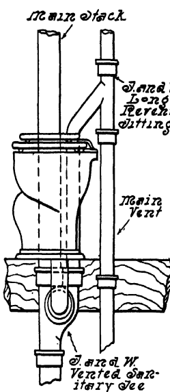
FIG. 148.—Use of Special Waste and Vent Fittings.
