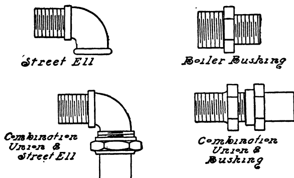
FIG. 281.—Malleable Iron Boiler Fittings.
