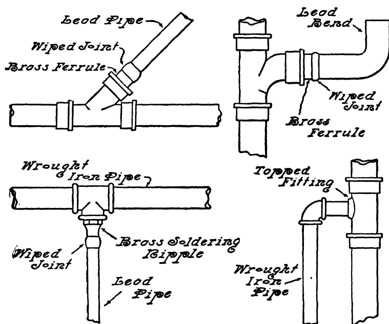
FIG. 101.—Connections between Lead-, Wrought- and Cast-Iron Pipes.
