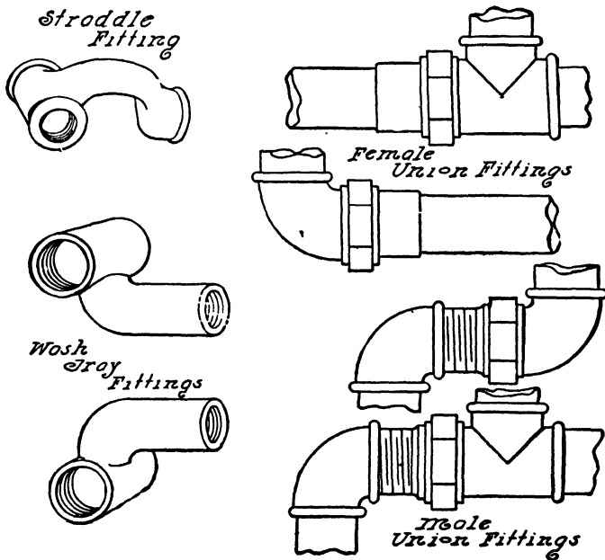
FIG. 264.—Special Supply Fittings.
