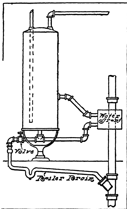
FIG. 272.—Drainage of Boiler into Drainage System—Poor Practice.
