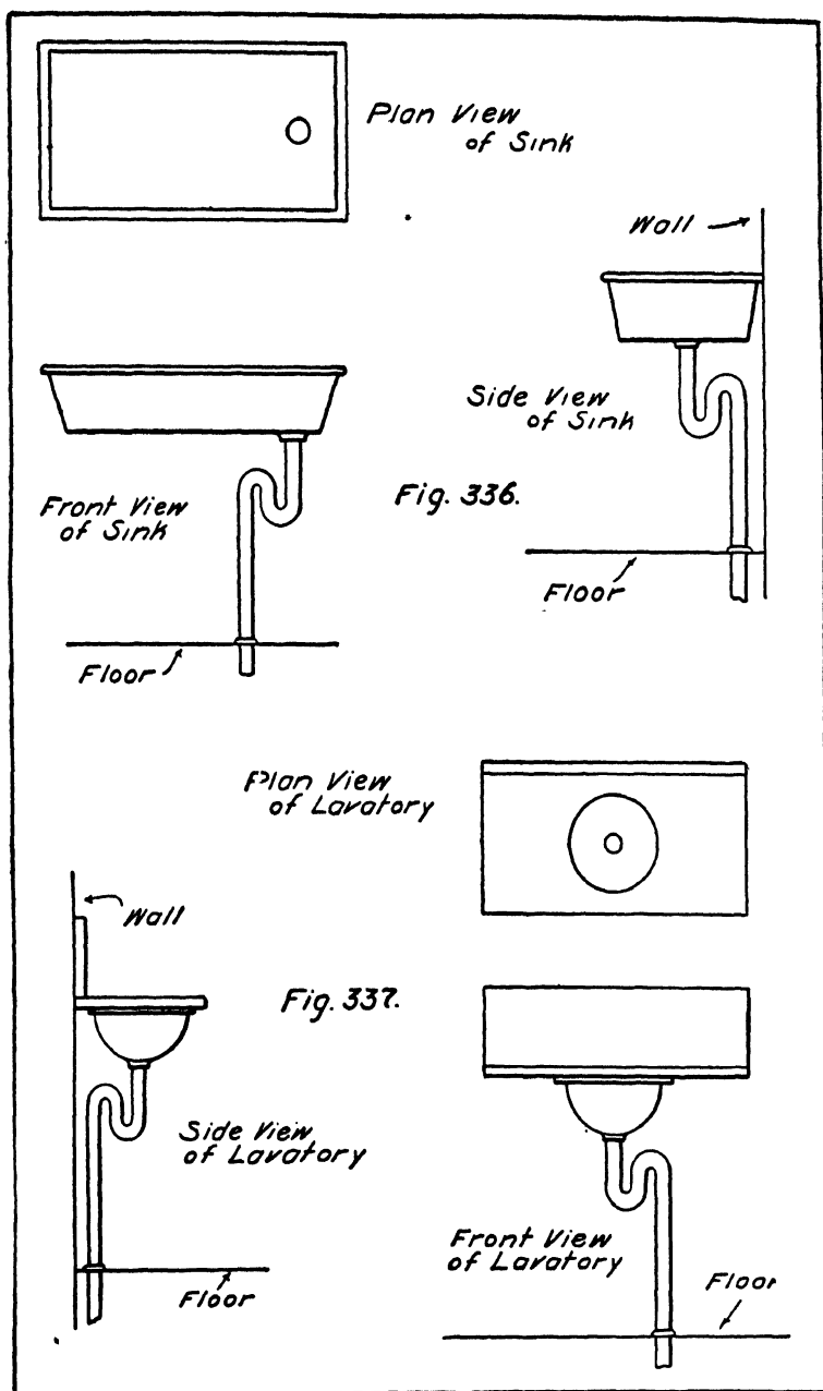
FIGS. 336-337.—Plan and Elevations of Common Fixtures.
