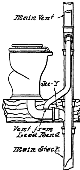
FIG. 141.—Ordinary Method of Venting Water-Closets.
