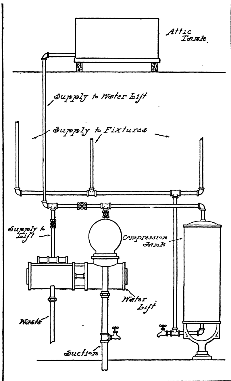
FIG. 231.—The Use of the Water Lift in Connection with the Country Plumbing System.
