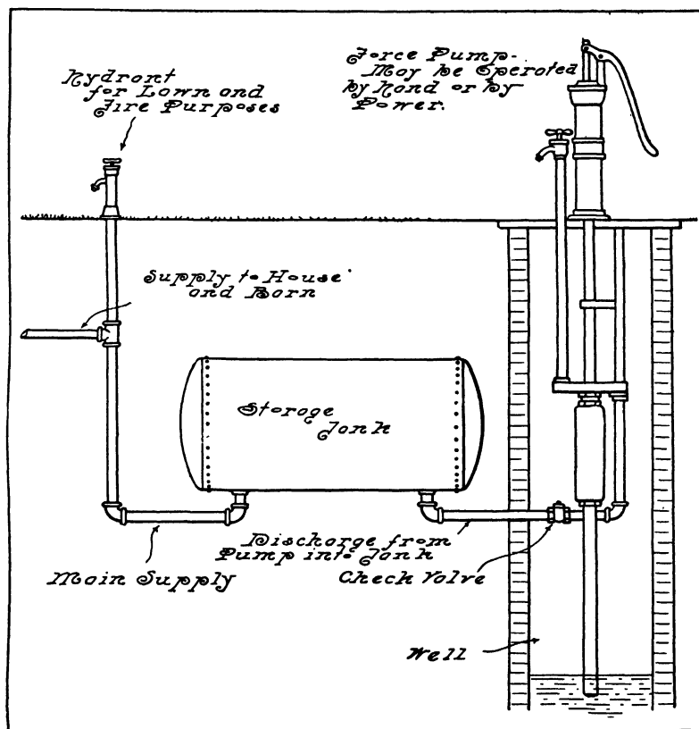
FIG. 225.—The Pneumatic System of Water Supply for Country Use.
