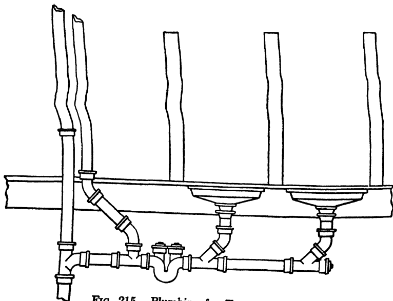
FIG. 215.—Plumbing for Two or More Horse Stalls.
