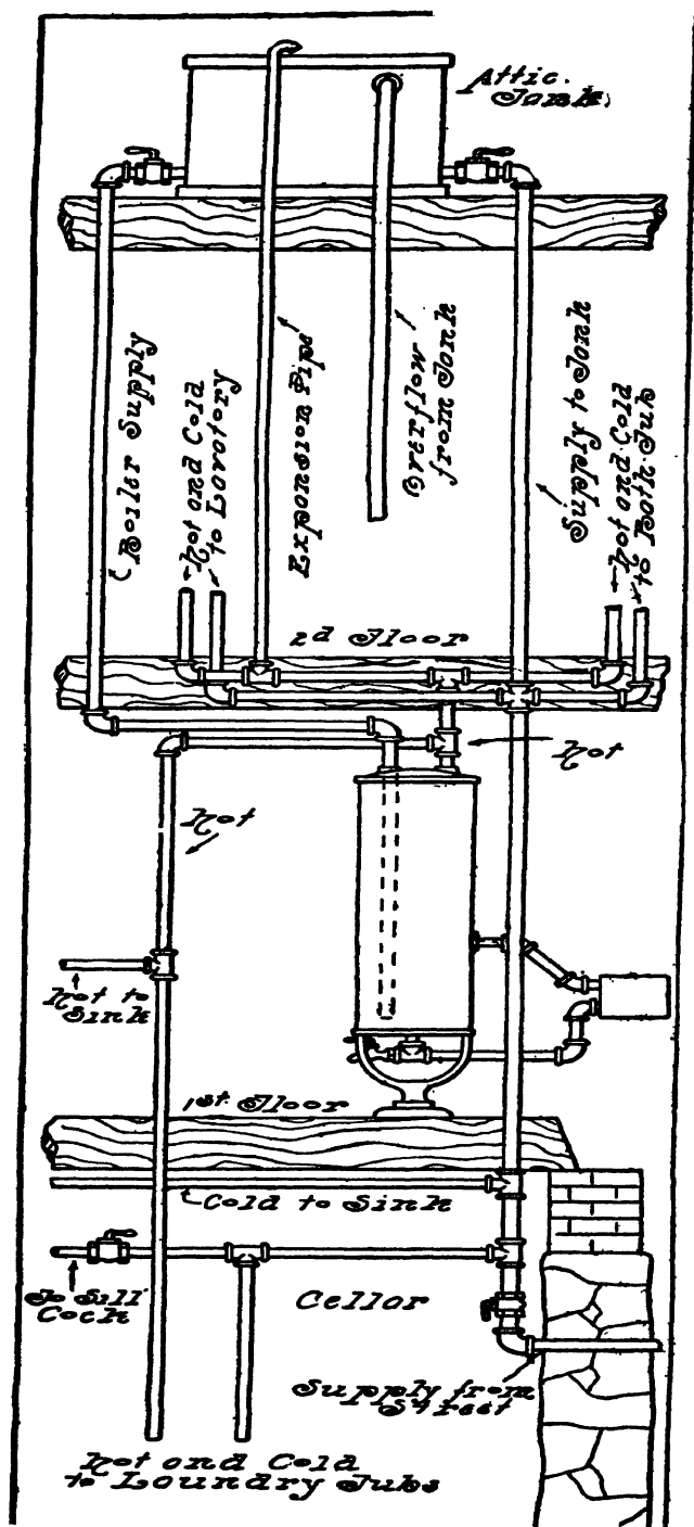
FIG. 293.—The Tank System of Hot Water Supply without Circulation.
