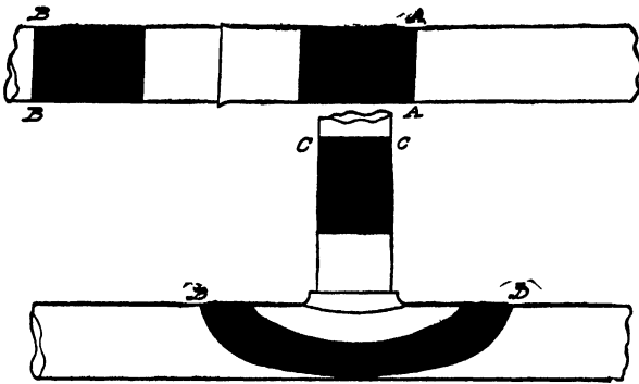
FIG. 11.—Joints Prepared with Soil, Ready to be Wiped.
