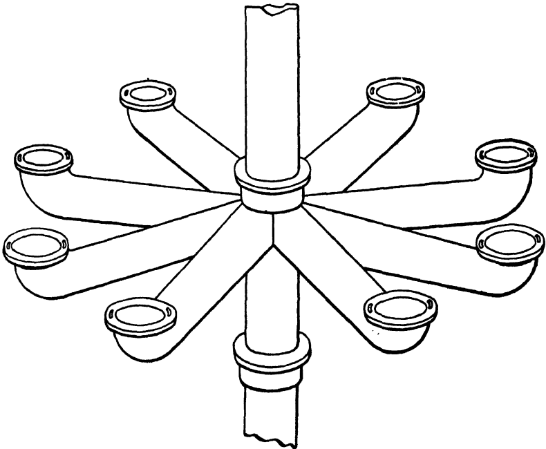
FIG. 182.—A Waste Fitting for Water-Closets Set in a Group at the Center of the Toilet Room.
