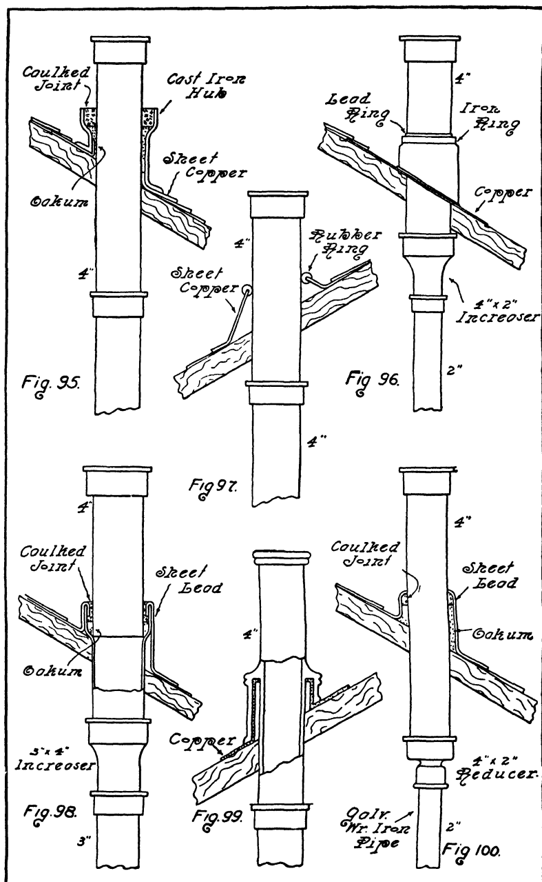
FIGS. 95-100.—Roof Connections.
