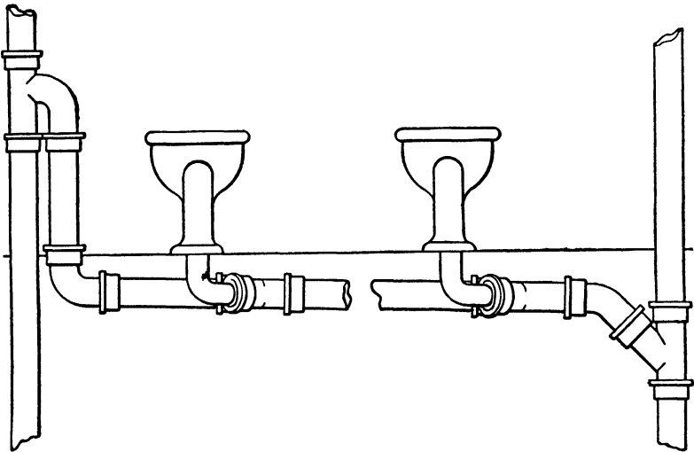
FIG. 67.—Continuous or Circuit Venting of Water-Closets.
