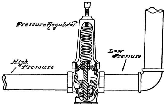
FIG. 263.—Use of Pressure Regulator.
