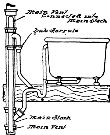
FIG. 185.—Connections for Foot Bath.
