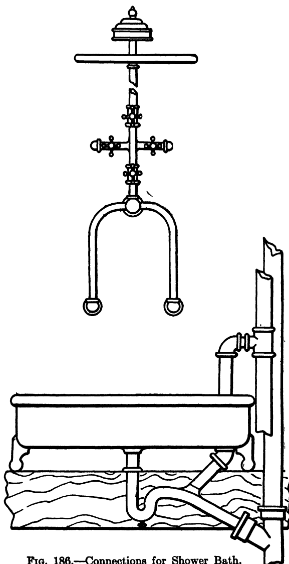
FIG. 186.—Connections for Shower Bath.
