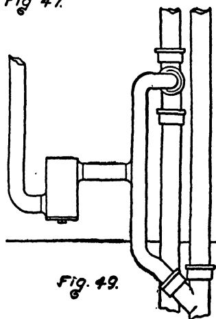
FIGS. 45-49.—Waste and Vent Connections of Drum Traps.
