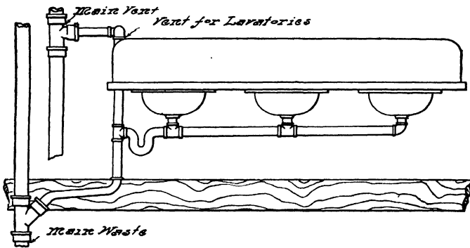
FIG. 195.—Poor Method of Connecting Line of Lavatories into One Trap.
