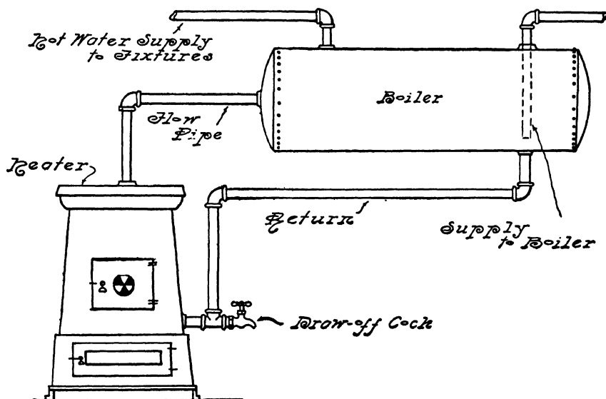
FIG. 309.—Connections for Horizontal Boiler and Tank Heater.
