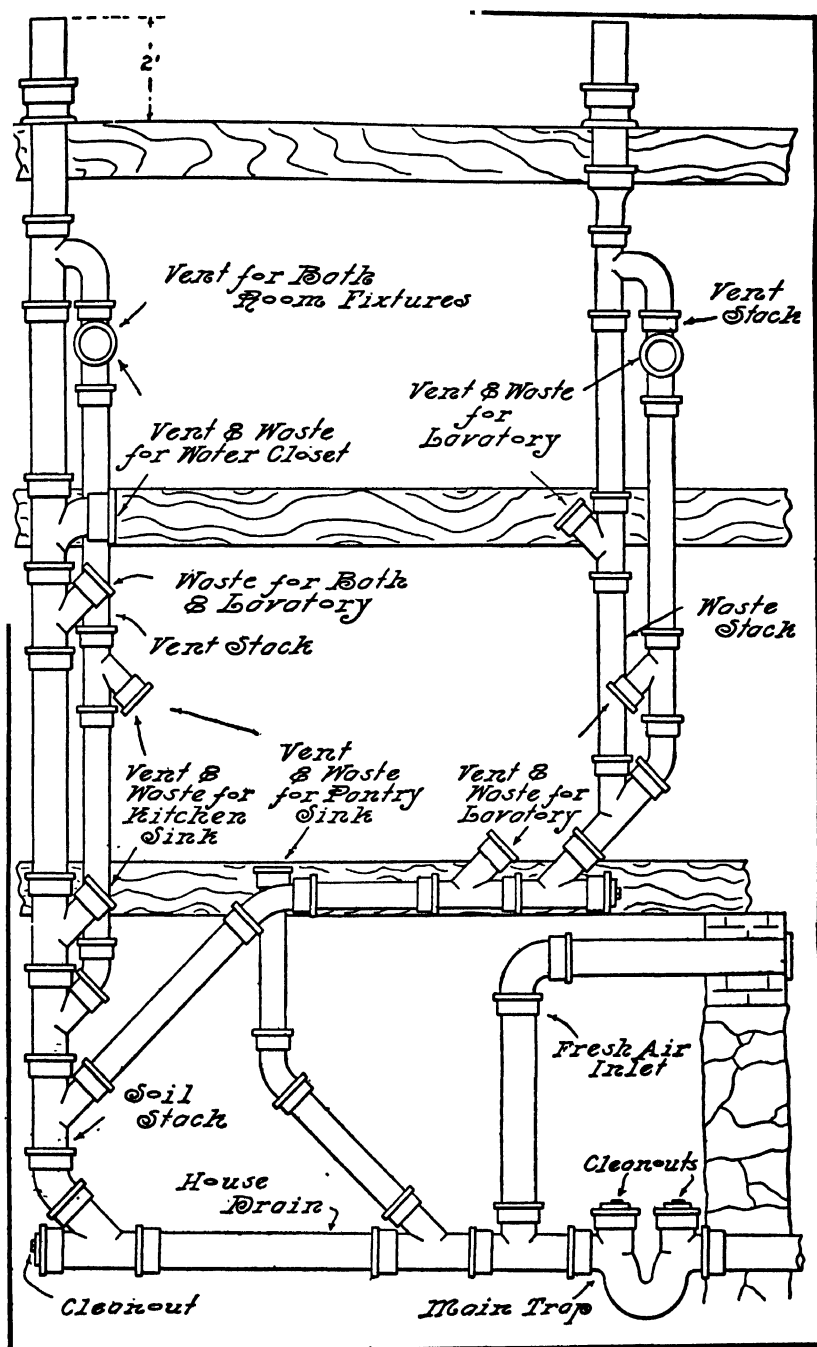
FIG. 89.—System of Soil Piping.
