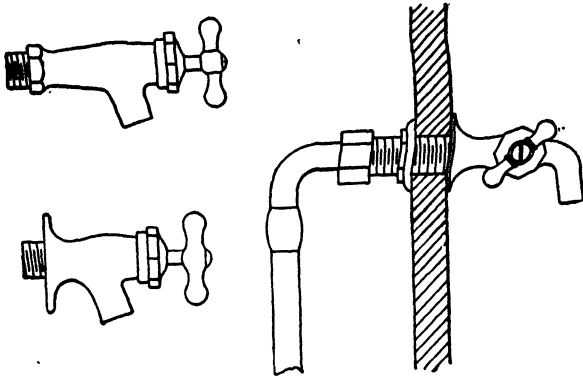
FIG. 266.—Wash-tray Bibbs.
