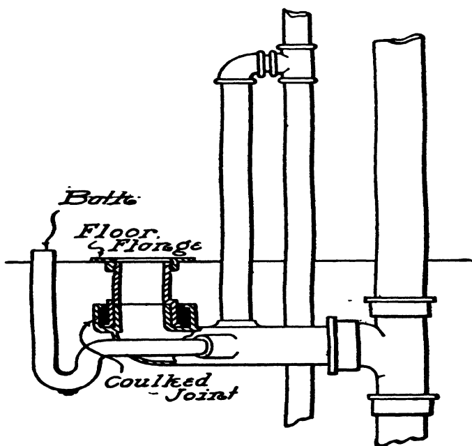
FIG. 179.—Another Modern Vented Waste Fitting.
