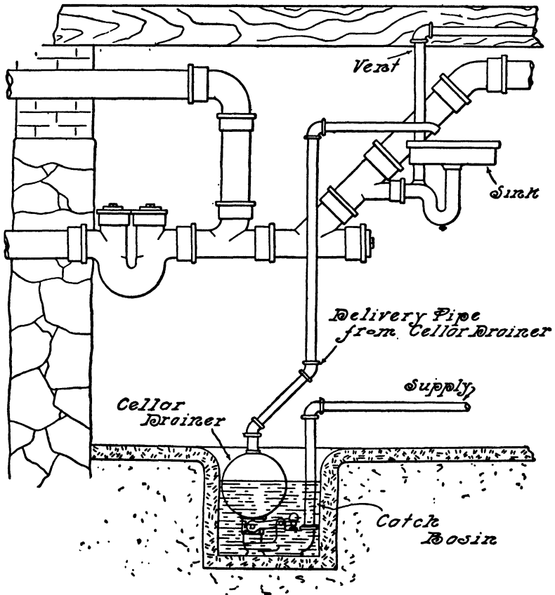
FIG. 116.—Connections for Cellar Drainer.
