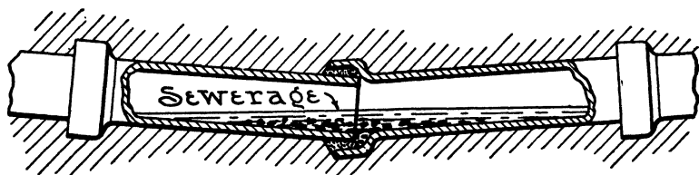
FIG. 71.—Settling and Breaking of Earthenware Pipes.
