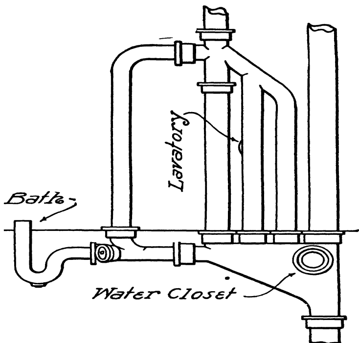
FIG. 179.—Another Modern Vented Waste Fitting.
