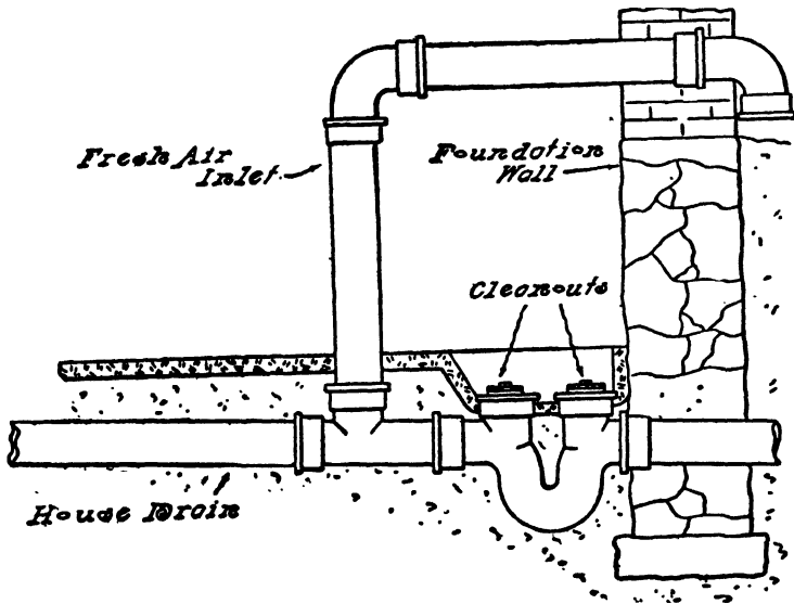
FIG. 111.—The Main Trap and Fresh-Air Inlet.
