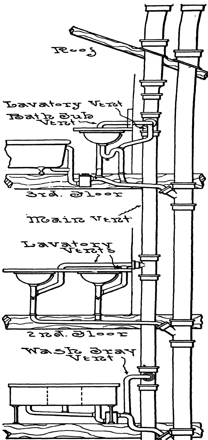
FIG. 26.—Traps and Connections for a Line of Fixtures.
