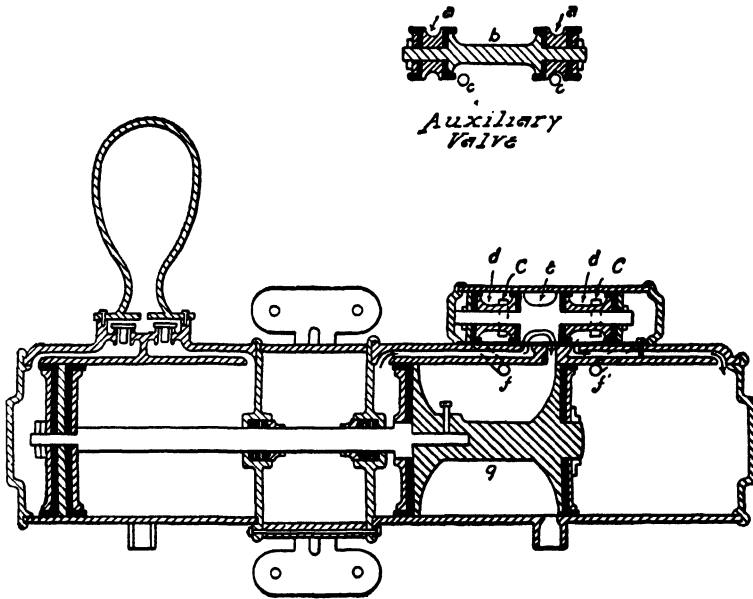
FIG. 322.—Sectional View of Water Lift and Auxiliary Valve.
