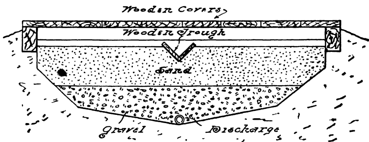
FIG. 244.—End View of Sewage Filter Bed.
