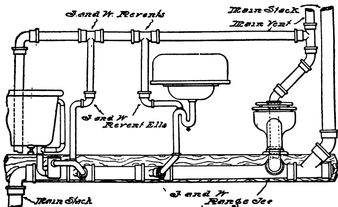
FIG. 126.—Separate Waste Entrances by Means of Special Fittings.
