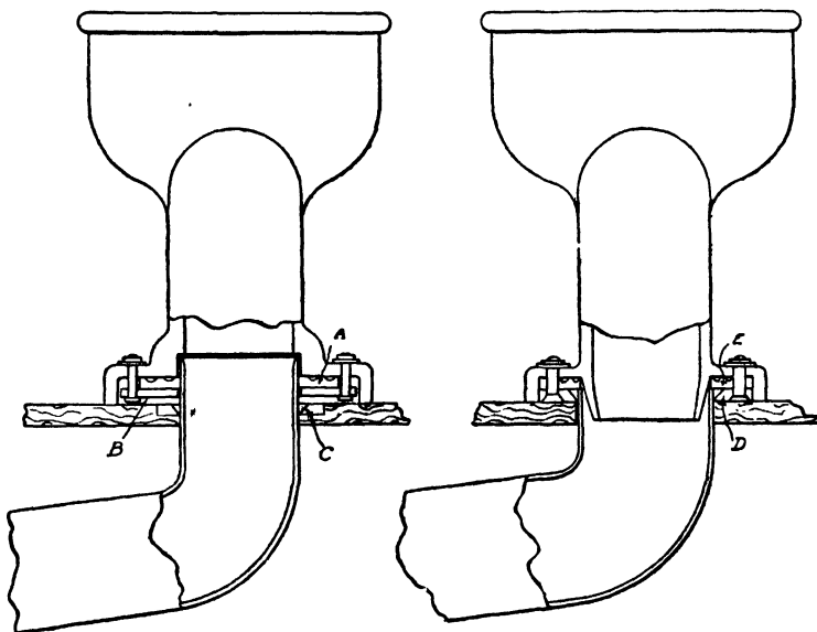
FIG. 136.—Water-Closet Floor Connections.
