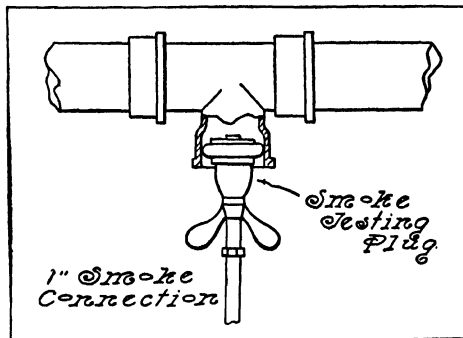
FIG. 87.—Smoke Testing Plug.
