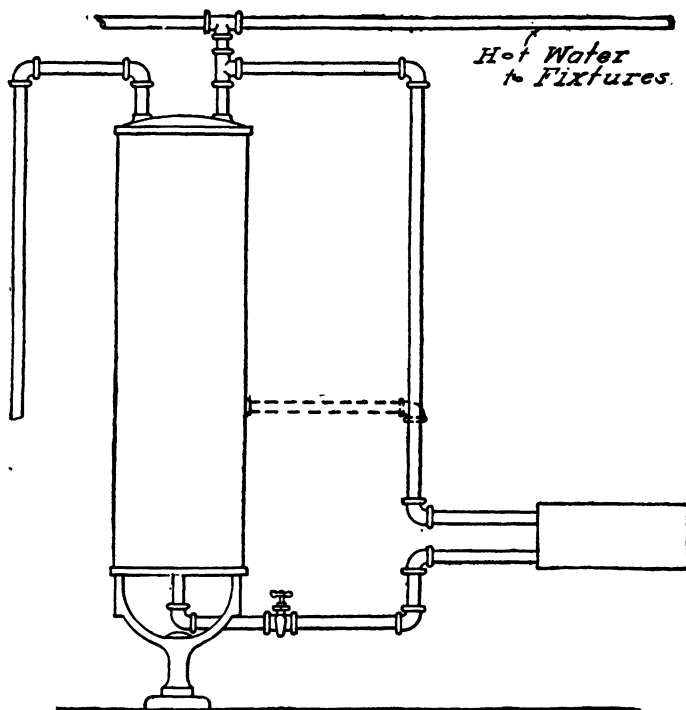
FIG. 295.—Quick-Heating Range Connection.
