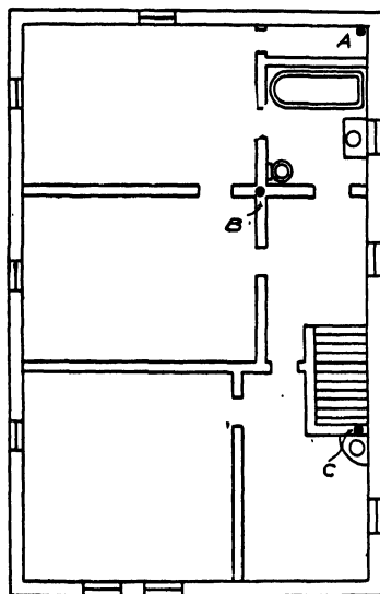
Second Floor Plan Fig. 345.
