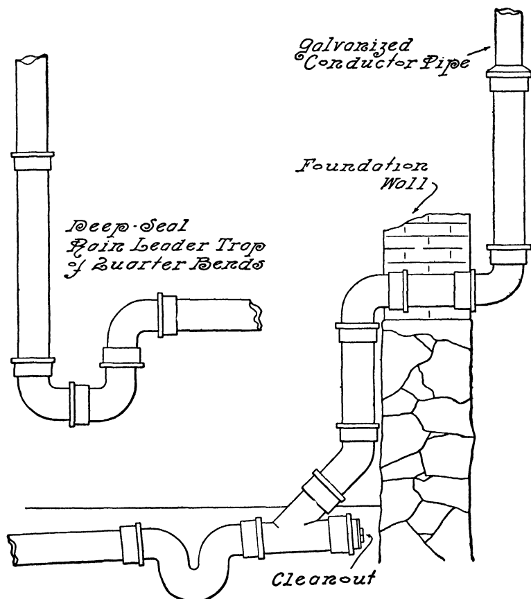
FIG. 115.—Rain Leader Connections.
