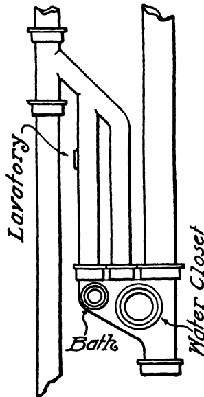
FIG. 174.—A Modern Vented Waste Fitting.
