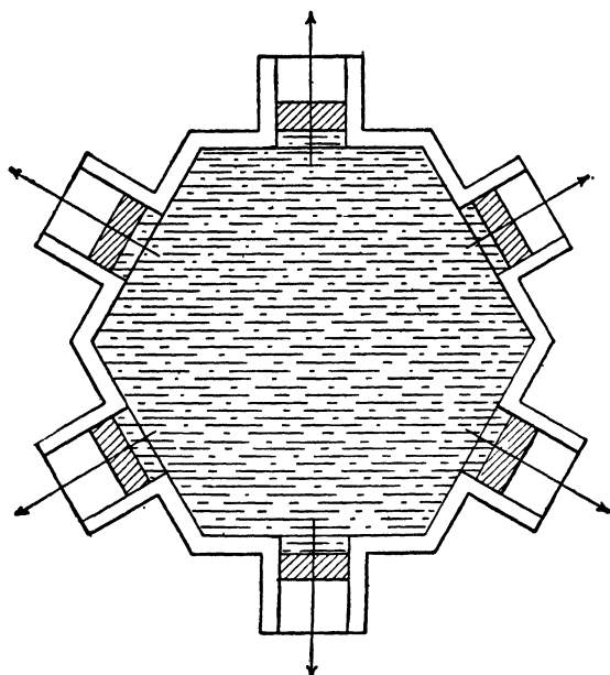
FIG. 332.—Direction of Pressure.
