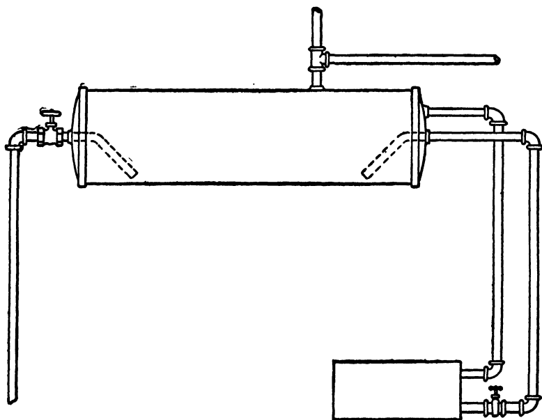
FIG. 275.—Connections for Horizontal Range Boiler.
