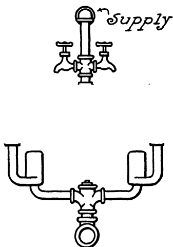
FIG. 204.—End View of Double Line of Wash Sinks.
