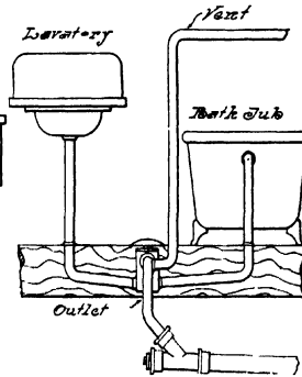
FIG. 120.—Lavatory and Bath Tub Connected into Drum Trap.—Poor Practice.
