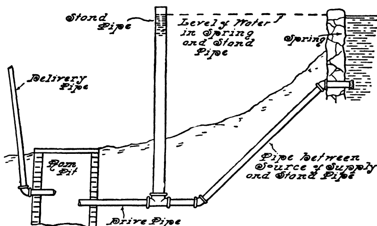
FIG. 229.—Method of Obtaining Direct Drive for Hydraulic Ram.
