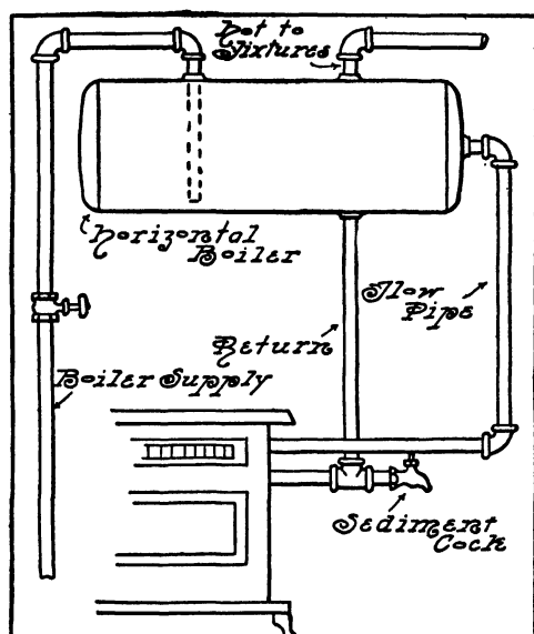
FIG. 276.—Connections for Horizontal Range Boiler.
