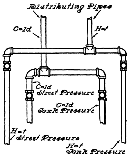
FIG. 318.—Simple Form of Cut-off.
