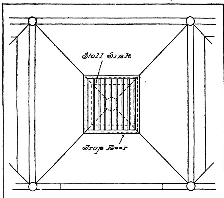
FIG. 218.—Plan of Box Stall, Showing Sink.
