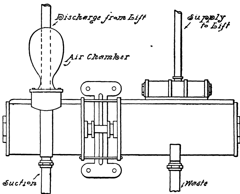
FIG. 323.—Connections for Water Lift.
