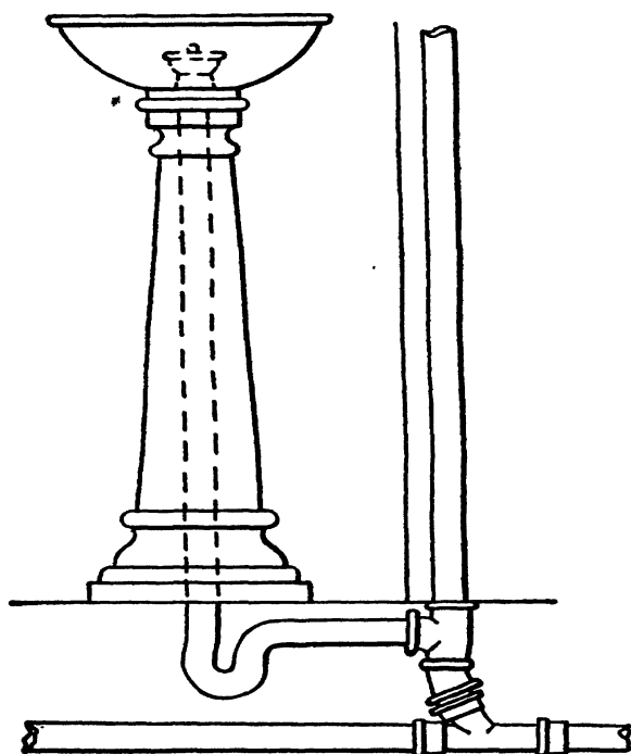
FIG. 211.—A Sanitary Pedestal Drinking Fountain.
