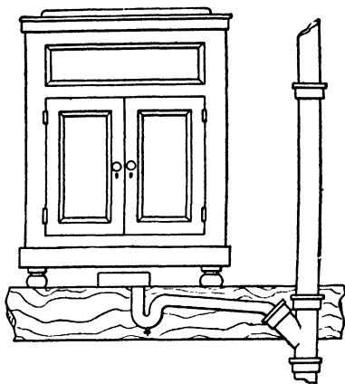
FIG. 191.—Wrong Connections for Refrigerator.
