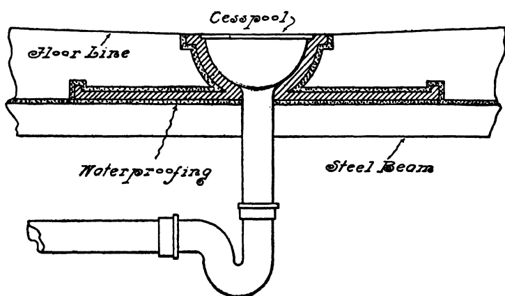
FIG. 219.—Watertight Drain.
