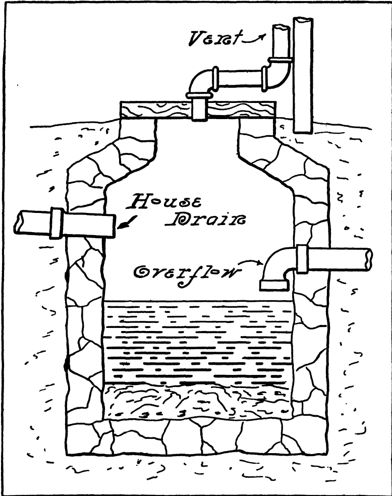
FIG. 240.—The Leeching Cesspool.
