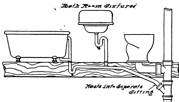
FIG. 123.—Connections Preferable to Those of Fig. 122.
