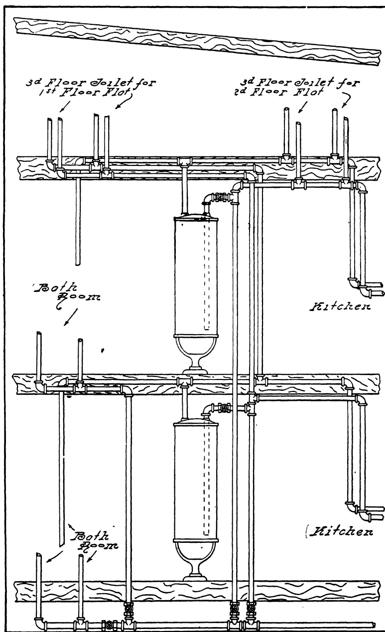
FIG. 256.—Pressure System for Two-Flat House.
