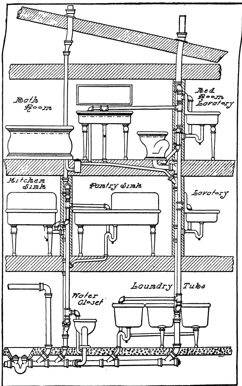
Plumbing for Residence.
