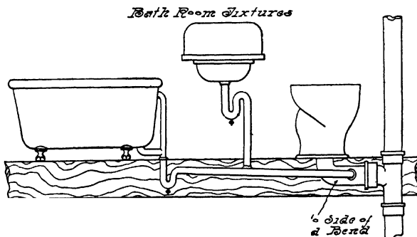
FIG. 122.—One Waste Entrance only for the Three Bath Room Fixtures.
