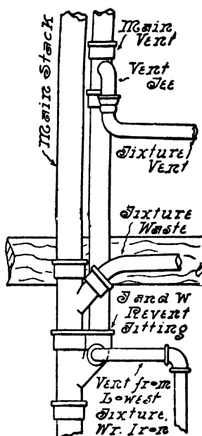
FIG. 58.—Special Main Vent Connection.
