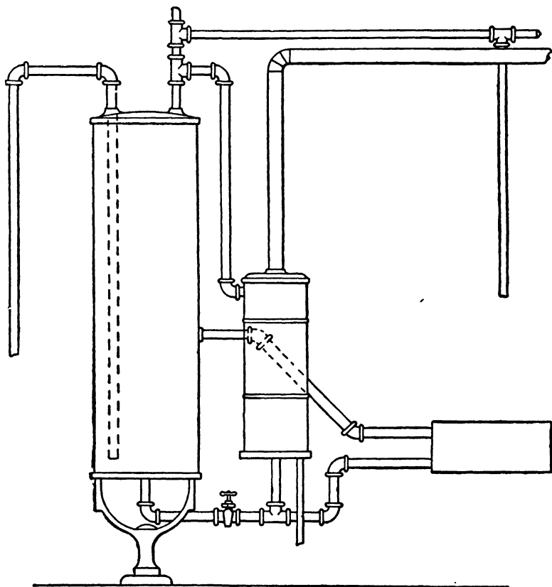
FIG. 298.—Range Boiler Heated by Kitchen Range and Auxiliary Heater.
