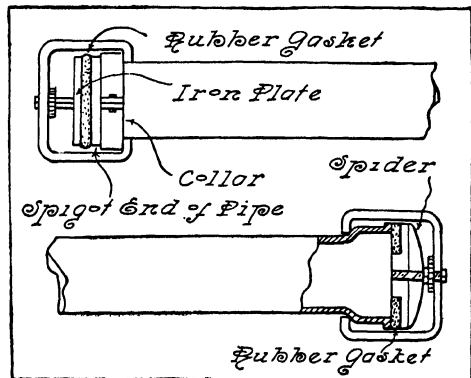
FIG. 86.—Special Testing Plugs.
