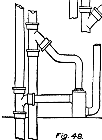
FIGS. 45-49.—Waste and Vent Connections of Drum Traps.
