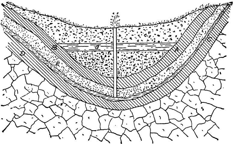
FIG. 333.—The Artesian Well.
