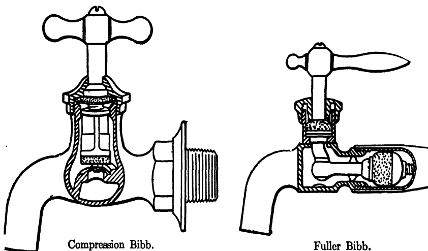
FIG. 259.—The Two Common Styles of Bibbs.
