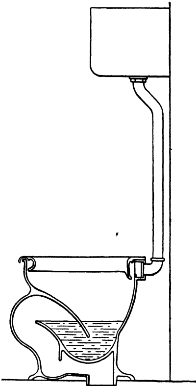
FIG. 132.—The Siphon Washdown Water-Closet
