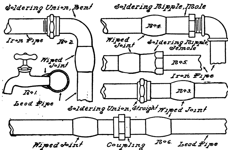
FIG. 16.—Wiping of Brass Work onto Lead Pipes.
