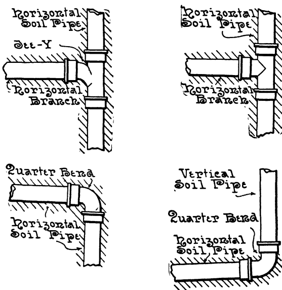
FIG. 78.—Wrong Methods of Making Changes in Direction in Soil Piping.
