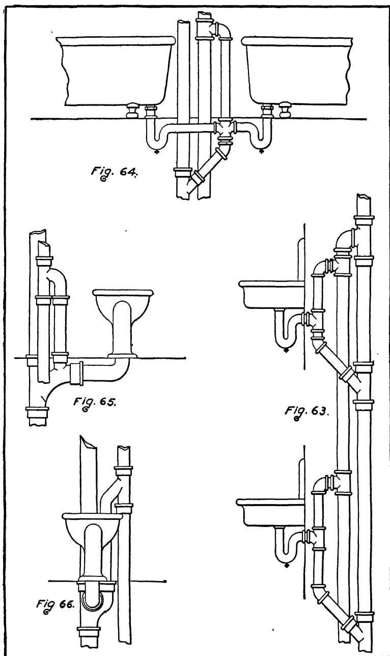
FIGS. 63-66.—Examples of Continuous Venting.
