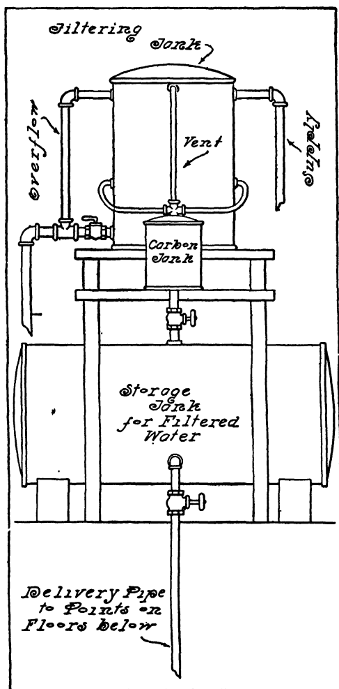
FIG. 239.—Gravity Filter for Hospitals, Hotels, Restaurants, etc.
