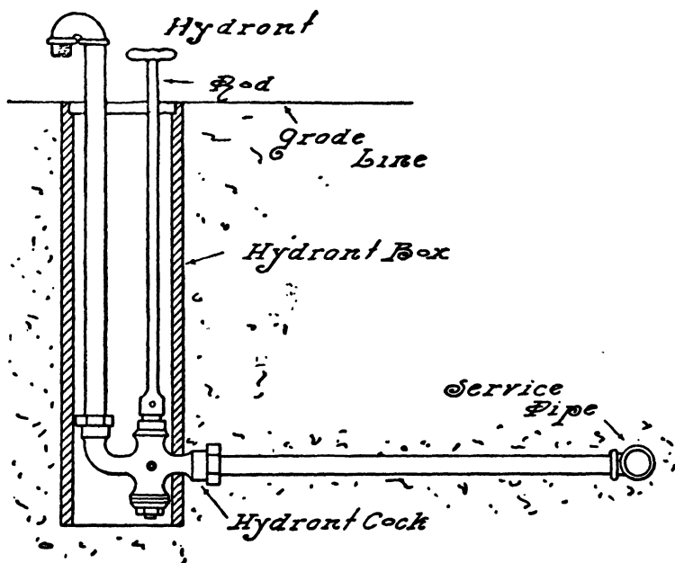
FIG. 252.—Hydrant Connections.
