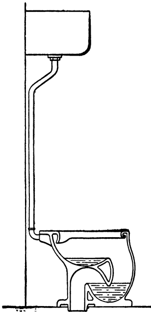
FIG. 130.—The Washout Water-Closet.
