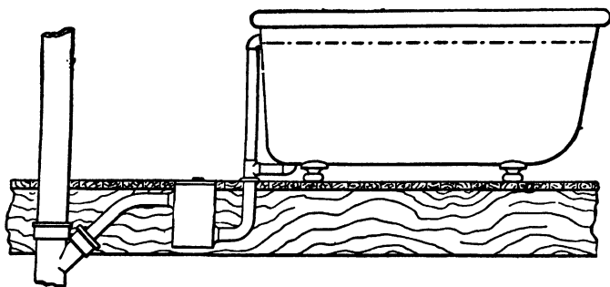
FIG. 28.—Use of Drum Trap under Floors.
