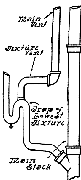
FIG. 56.—Wrong Method of Lower Connection of Main Vent.
