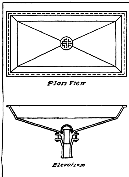
FIG. 216.—A Special Stall Drainage Sink.
