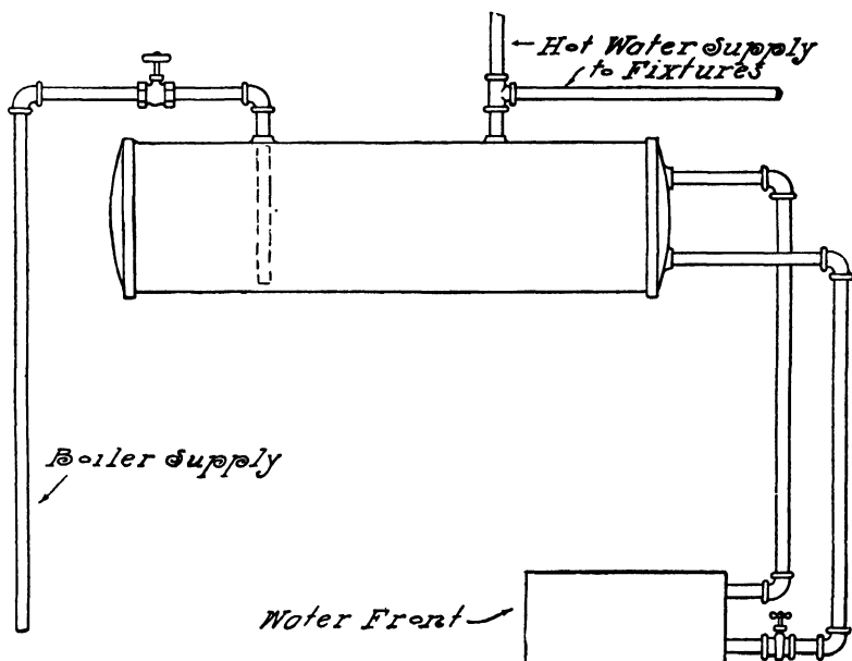
FIG. 274.—Connections for Horizontal Range Boiler.
