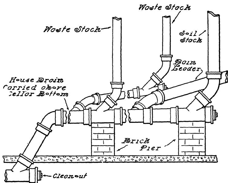
FIG. 76.—The House Drain and Pipes Discharging Into It.
