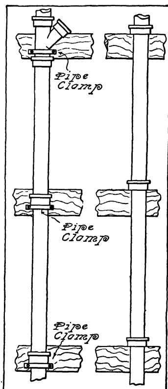
FIG. 109.—Supporting of Vertical Lines of Pipe.
