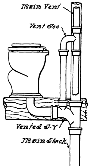
FIG. 142.—Water-Closet Vented from T-Y.
