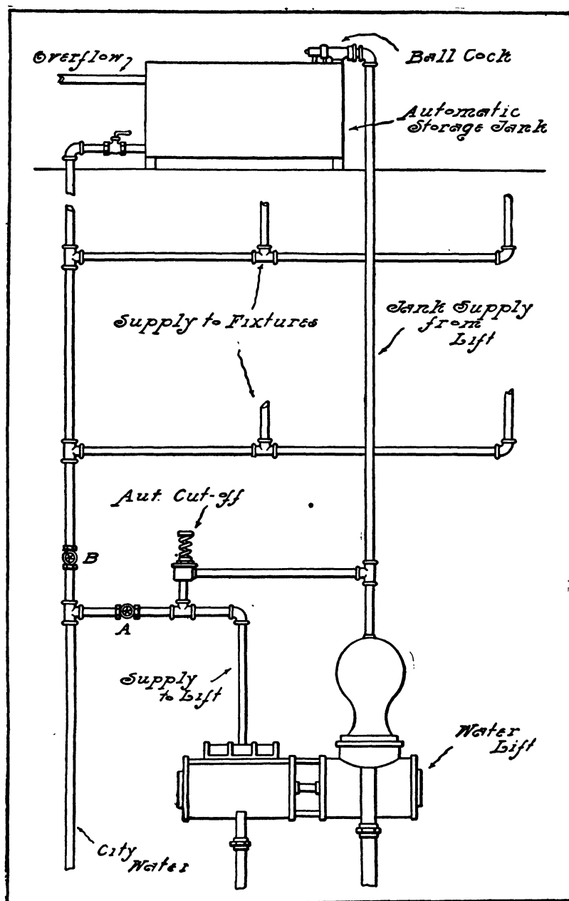
FIG. 326.—Water Lift Used on Automatic Storage Tank System.
