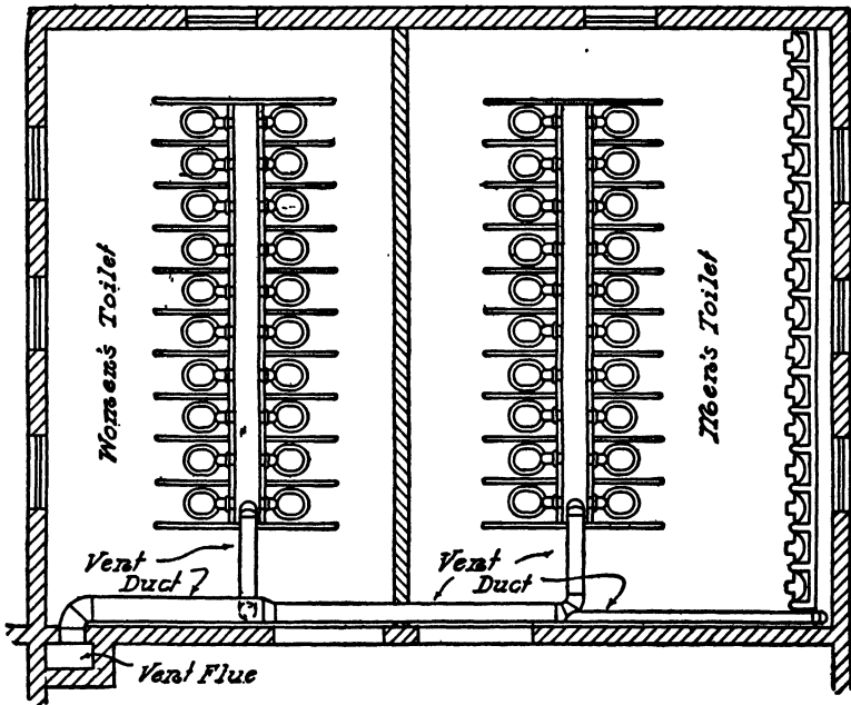
FIG. 173.—Local Ventilation for Toilet Rooms, Including Ventilation of Urinals.
