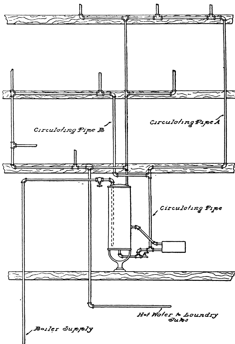
FIG. 289.—Hot-water Supply with Circulation.
