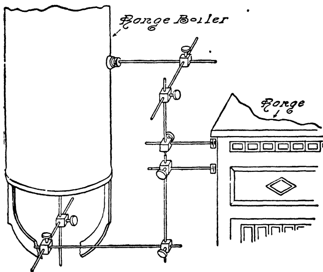
FIG 283.—Use of Center-Meter, a Device for Taking Range Connection Measurements.
