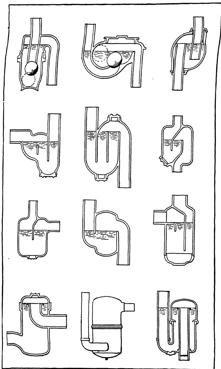
FIG. 29.—Various Patented Traps in More or Less Common Use.
