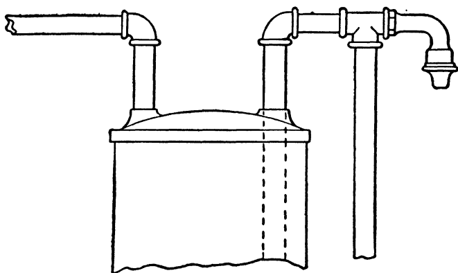
FIG. 257.—Use of the Vacuum Valve.
