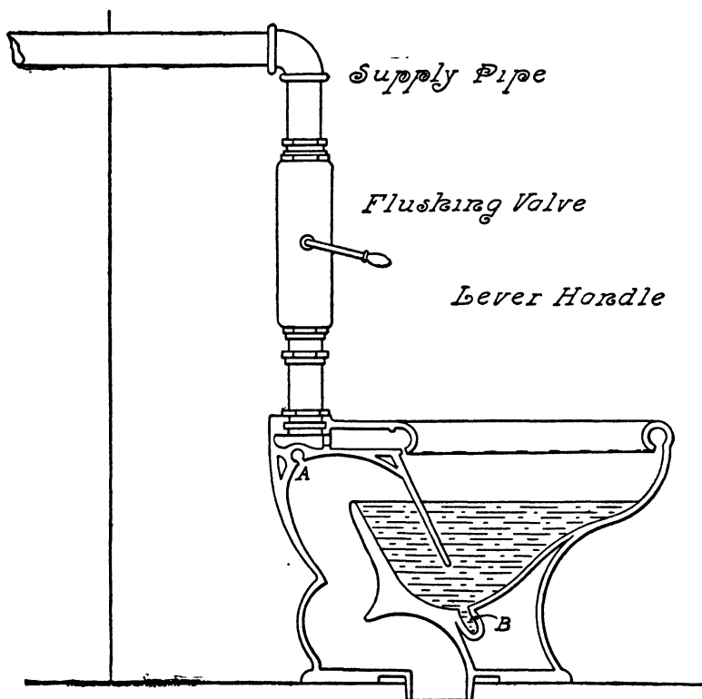
FIG. 158.—The Flushing Valve,—Double-Jet Siphon Water-Closet.
