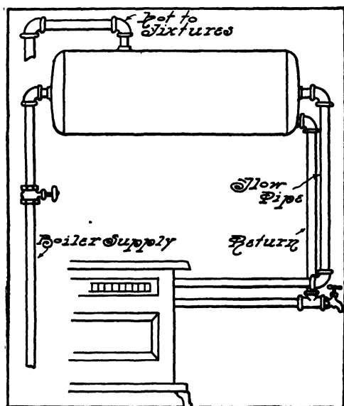
FIG. 278.—The Horizontal Range Boiler Improperly Connected.
