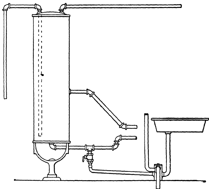
FIG. 271.—Drainage of Boiler into Sink Trap,—Poor Practice.
