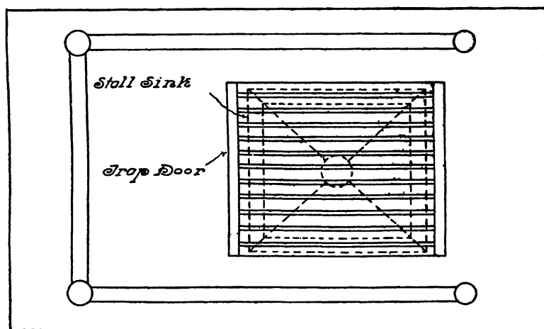
FIG. 217.—Plan of Horse Stall, Showing Sink.
