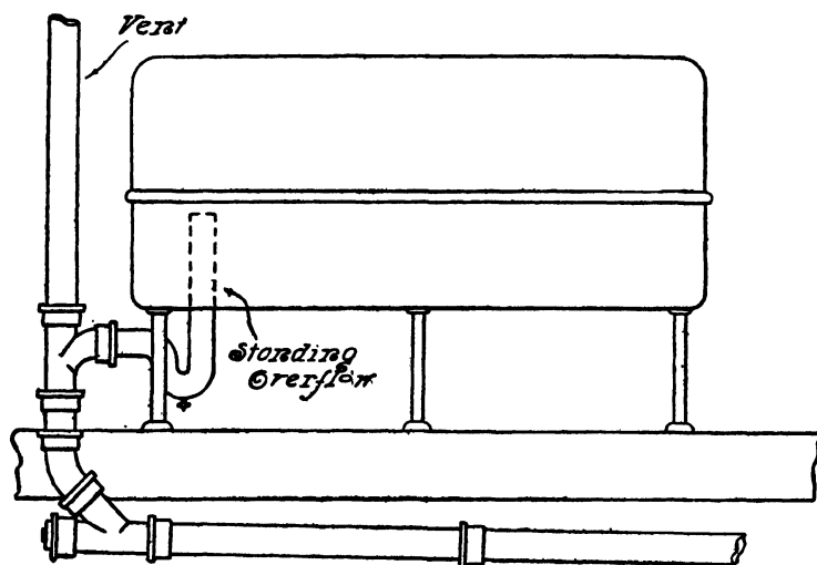
FIG. 220.—Connections for the Horse Trough.
