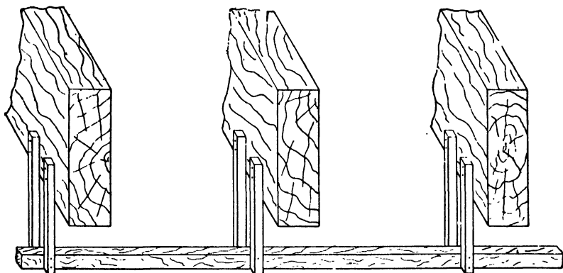
FIG. 22.—Support for Horizontal Line of Lead Pipe.
