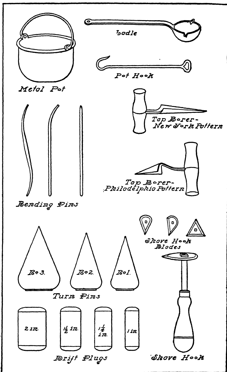
FIG. 1.—A Few of the Plumber's Tools.
