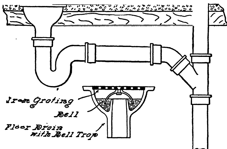
FIG. 114.—Floor Drain.
