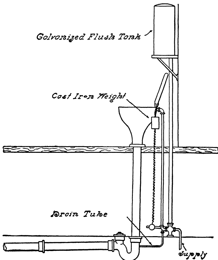
FIG. 159.—Frost-Proof Water-Closet.
