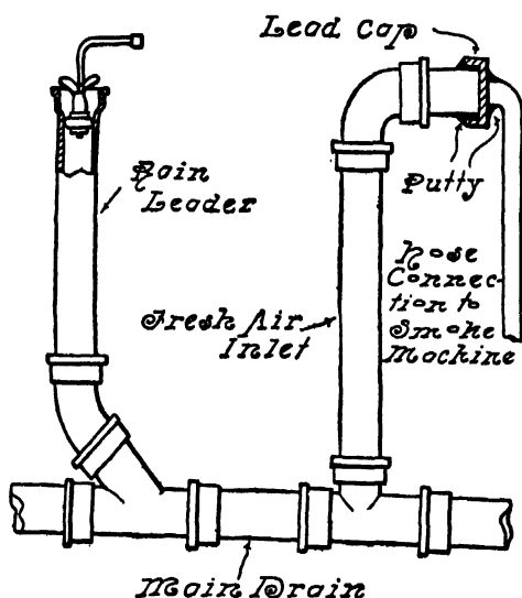
FIG. 88.—Plumbing under Smoke Test.
