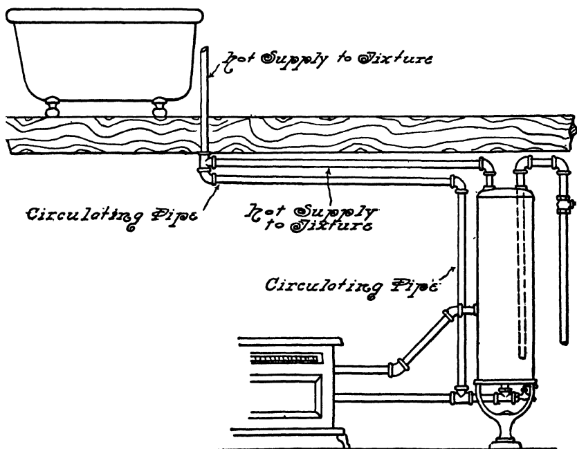
FIG. 286.—Circulation Applied to a Single Fixture.
