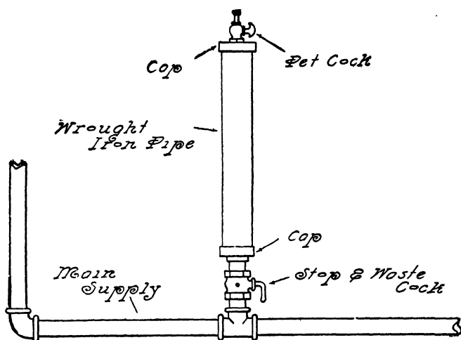
FIG. 262.—Air Chamber on Main Supply Pipe.
