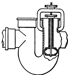
FIG. 83.—Testing Plug for Running Trap.
