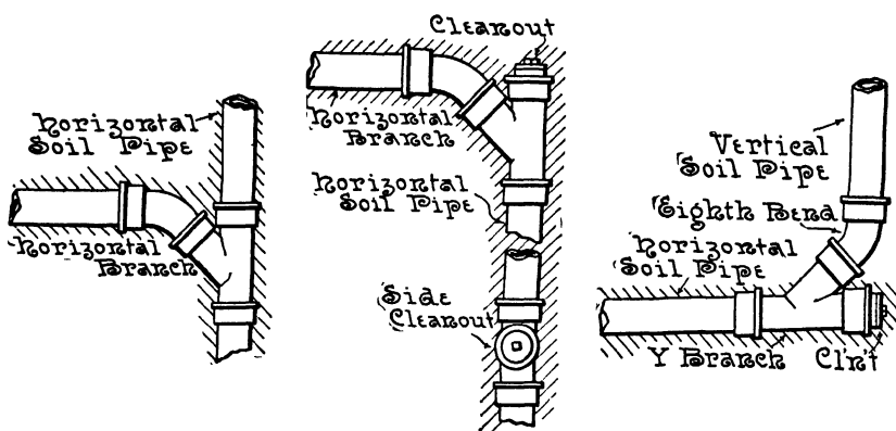
FIG. 77.—Correct Methods of Making Changes in Direction in Soil Piping.
