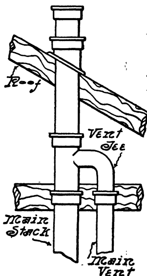
FIG. 53.—Upper Connection of Main Vent into Main Stack.
