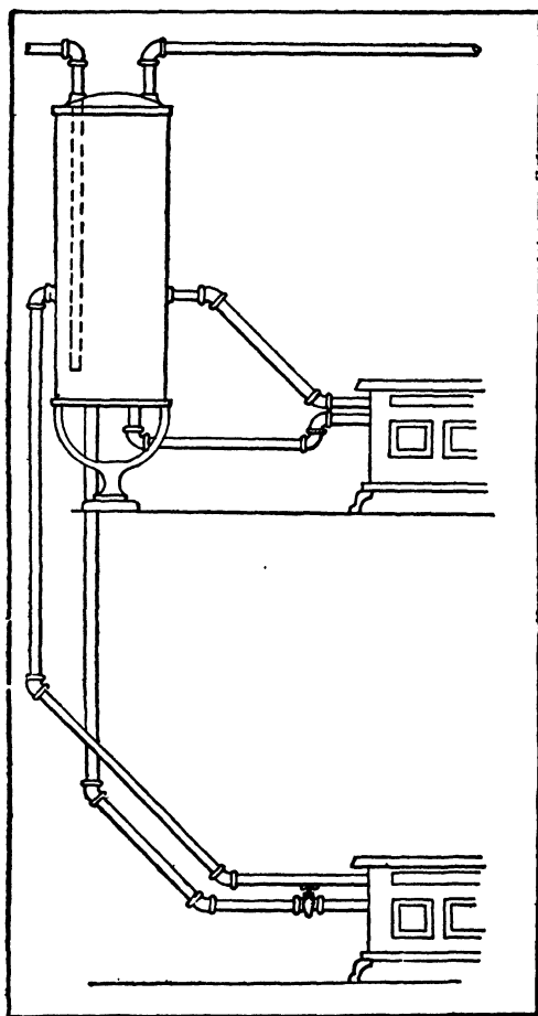
FIG. 304.—Range Boiler Heated by Two Ranges on Different Floors. Method No. 2.
