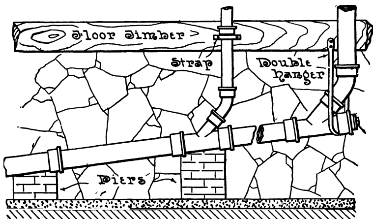
FIG. 75.—Running and Supporting of Exposed Cellar Piping.
