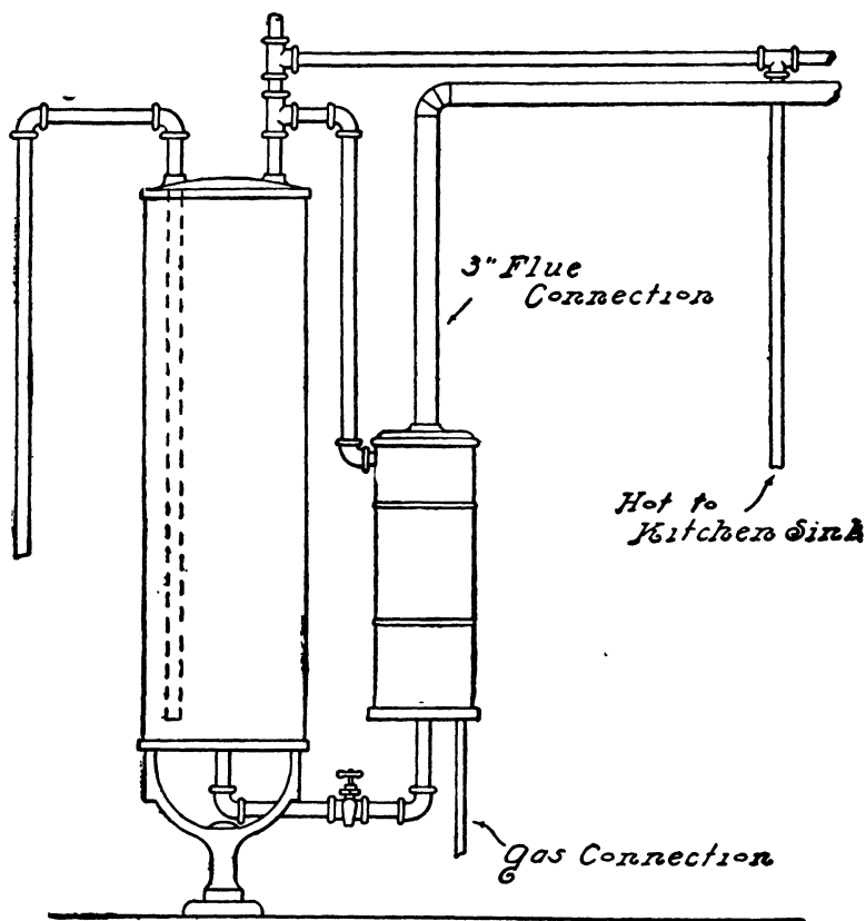
FIG. 297.—Connections for Auxiliary Gas Heater.
