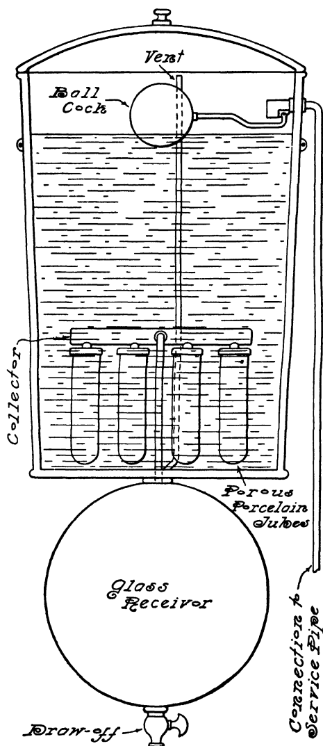
FIG. 238.—Domestic Gravity Filter.
