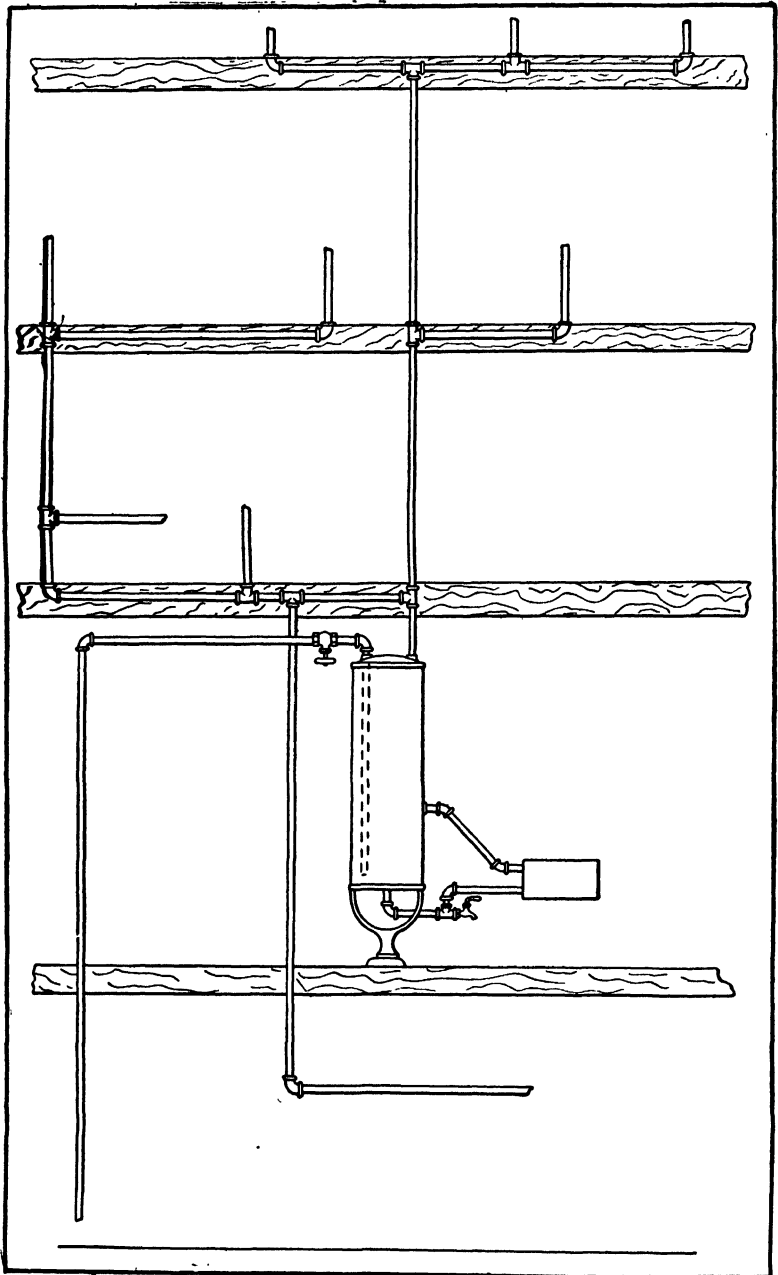
FIG 285.—System of Hot Water Supply without Circulation.
