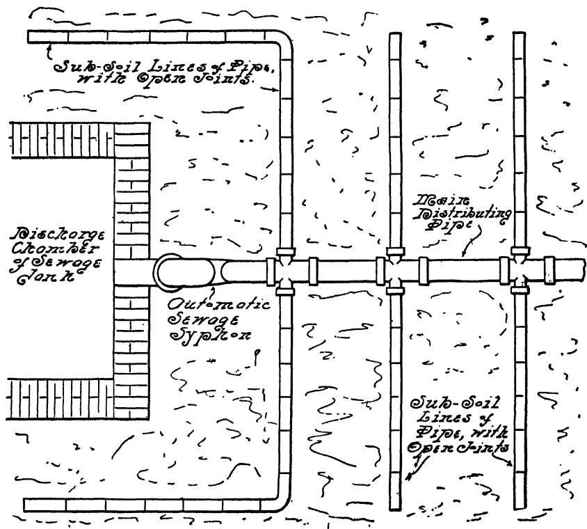
FIG. 242.—Sub-Soil System of Disposal of Sewage from Septic Tank.
