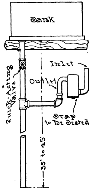
FIG. 31.—The Testing of Traps.
