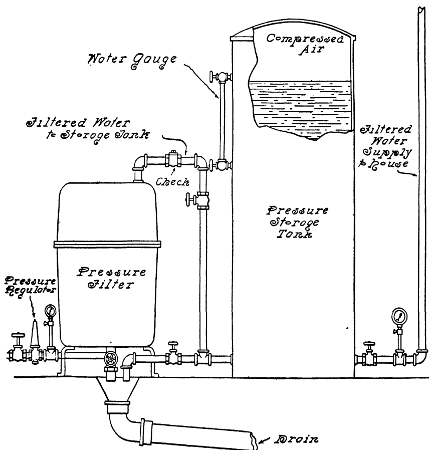
FIG. 235.—Pressure Filtering System for Residence Use, etc.
