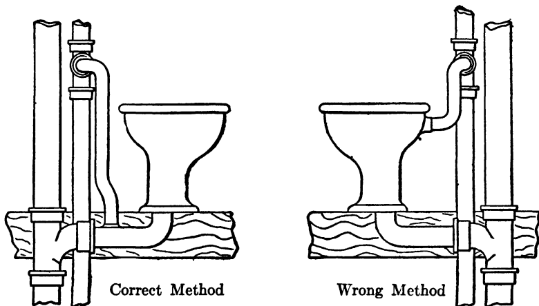
FIG. 50.—Venting of Water-Closets.
