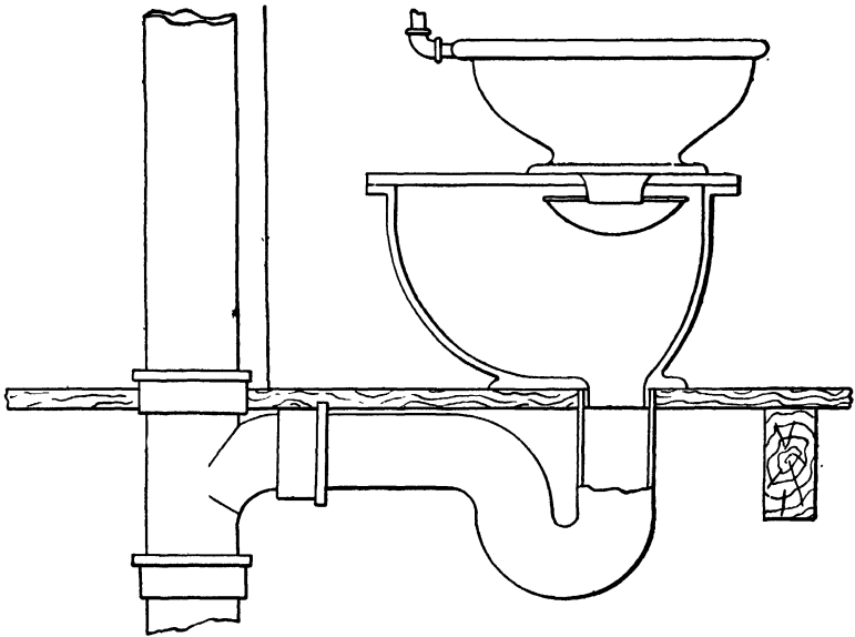
FIG. 127.—The Pan Water-Closet and Its Connections.
