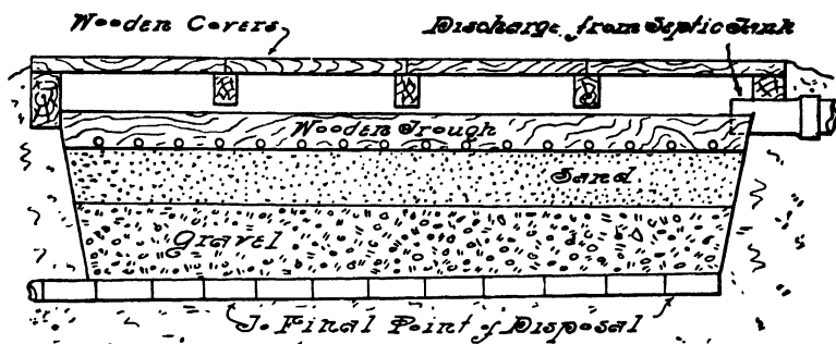
FIG. 243.—Side View of Sewage Filter Bed.
