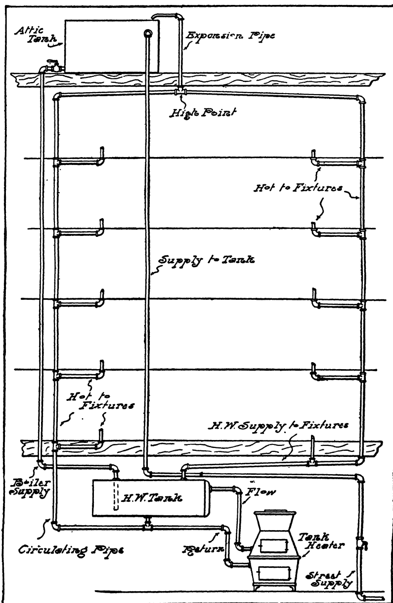
FIG. 313.—Hot Water Supply for Large Building Under Tank Pressure.
