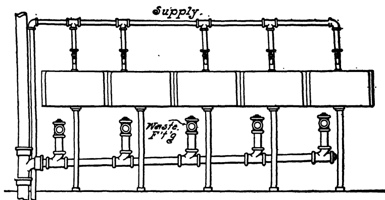
FIG. 203.—Wash Sinks for Schools, Factories, etc.
