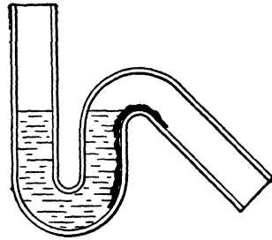
FIG. 33.—Trap Seal Broken by Capillary Action.
