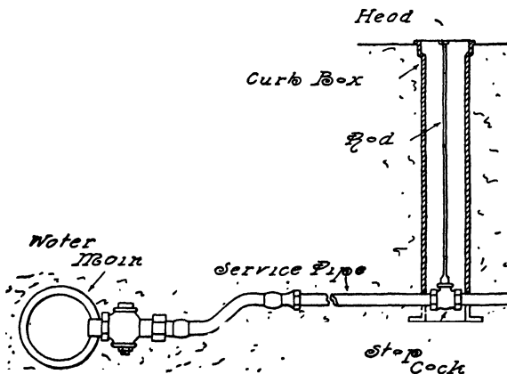
FIG. 249.—Shut-off on Service Pipe and Curb Box.
