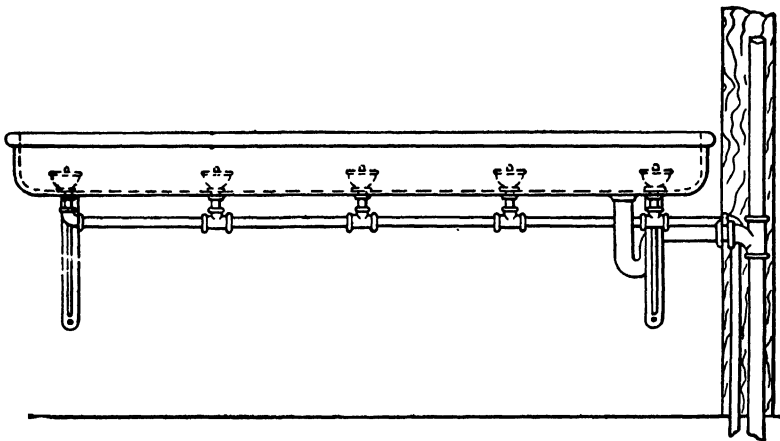
FIG. 212.—A Sanitary Drinking Fountain.
