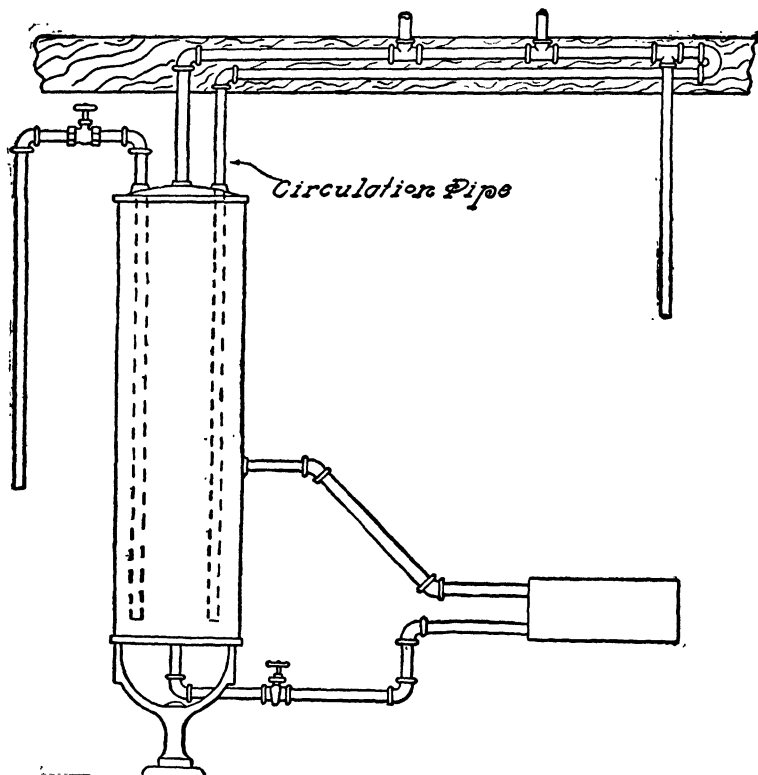
FIG. 290.—The Three-tube Boiler.
