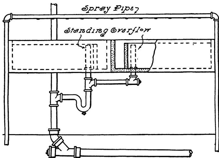
FIG. 206.—Factory Wash Sink.
