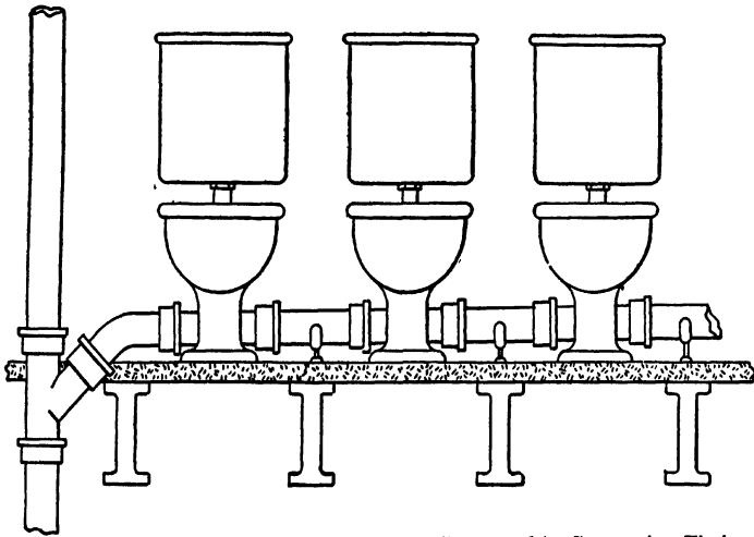
FIG. 139.—Soil Pipe for Line of Water-Closets Supported by Supporting Fittings.
