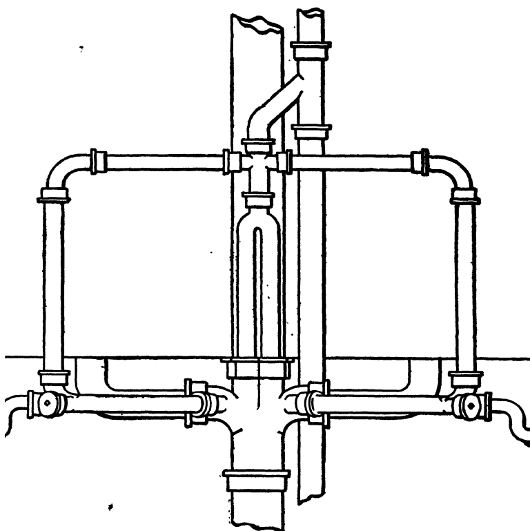
FIG. 176.—Fittings for Use in Installing Double Set of Fixtures.
