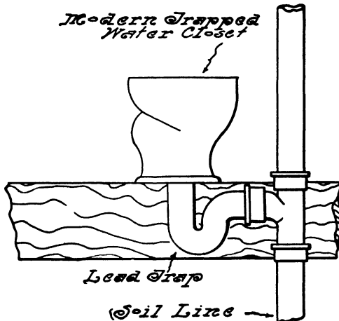
FIG. 157.—The Prohibited Offset Water-Closet.
