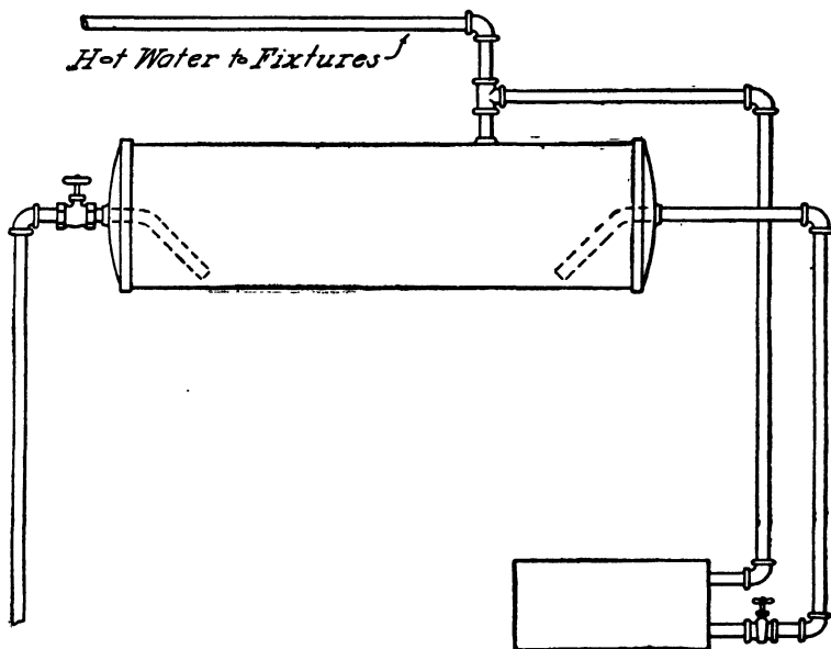
FIG. 296.—Quick-Heating Range Connection for Horizontal Boiler.
