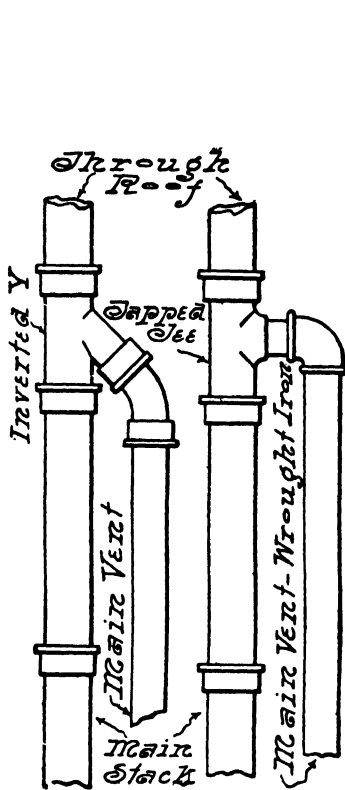
FIG. 54.—Two Methods of Upper Connection of Main Vent into Main Stack.
