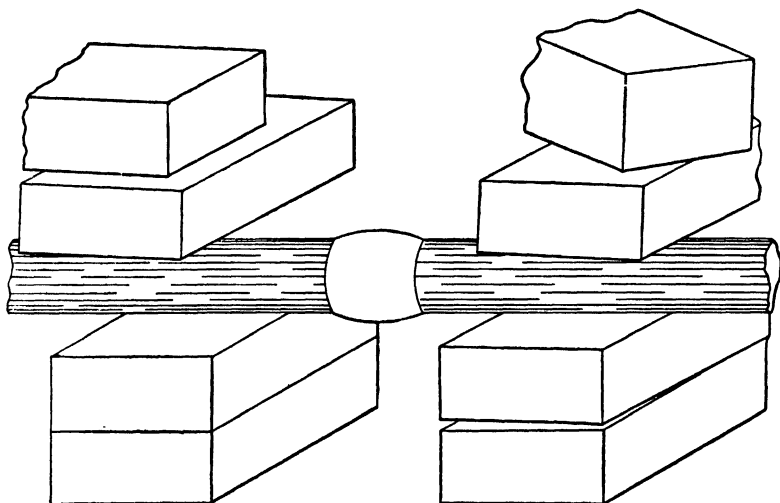
FIG. 12.—A Common Method of Holding Pipes for Wiping Joints.
