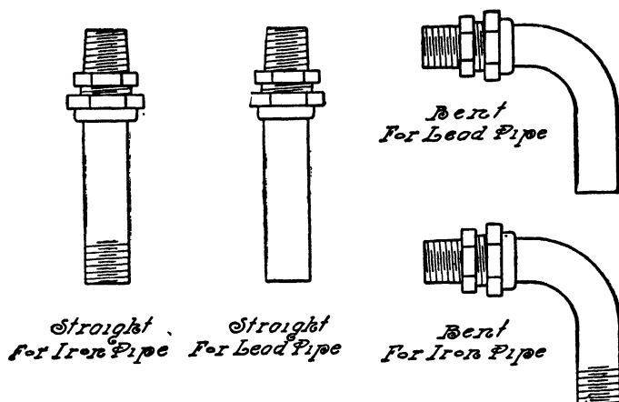
FIG. 280.—Boiler Couplings.
