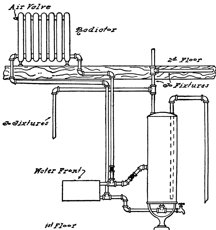
FIG. 328.—Radiator Heated from Range Boiler.
