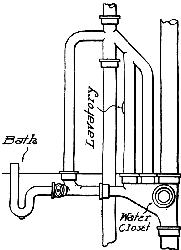
FIG. 178.—A Modern Vented Waste Fitting.
