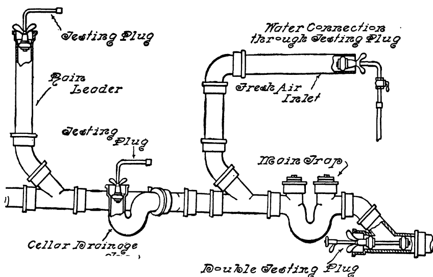
FIG. 82.—The Soil Piping in Readiness for the Water Test.
