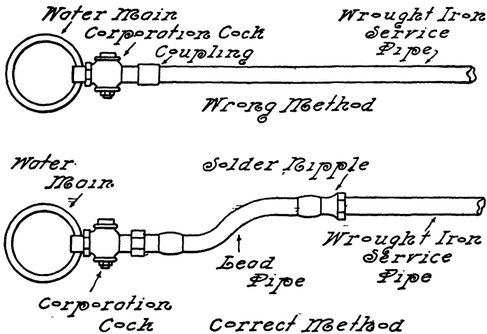
FIG. 248.—Service Connections.
