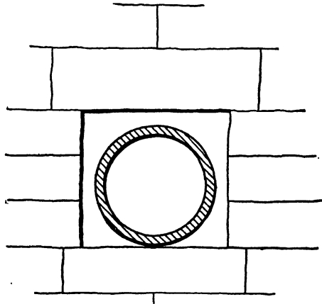
FIG. 73.—House Drain through Cellar Wall.
