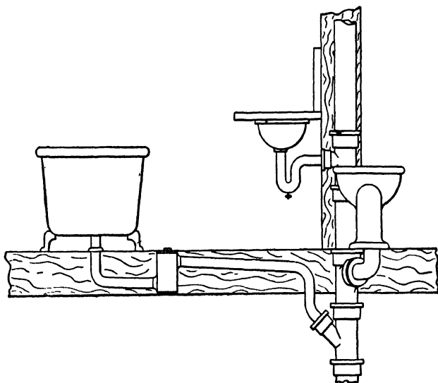
FIG. 92.—Separate Entrance of Each Fixture into Stack.
