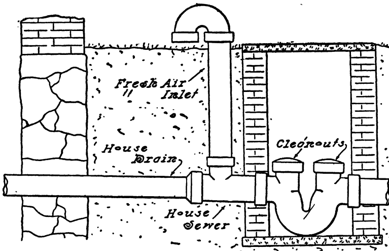
FIG. 112.—The Main Trap when Located on House Sewer.
