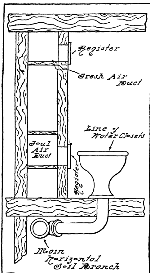
FIG. 202.—Ventilation of Line of Water-Closets in Public Toilet Room.
