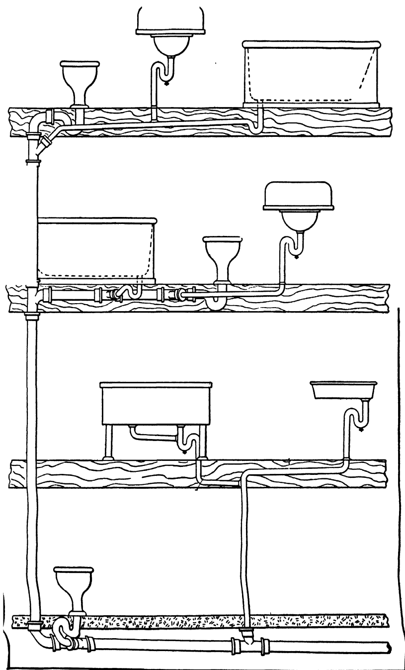
FIG. 36.—Siphonage of Traps in Old-Fashioned Unvented Plumbing System.
