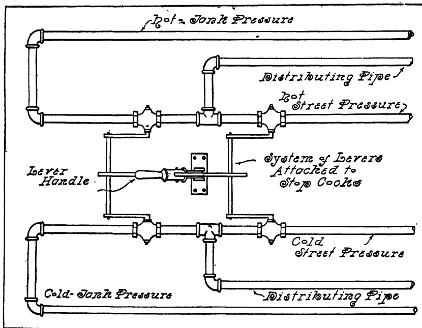
FIG. 319.—Automatic Cut-off.
