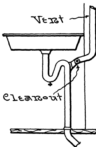
FIG. 60.—Cleanout on Trap Vent.
