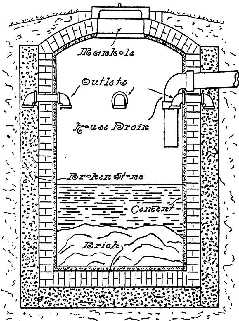
FIG. 241.—The Septic Cesspool.
