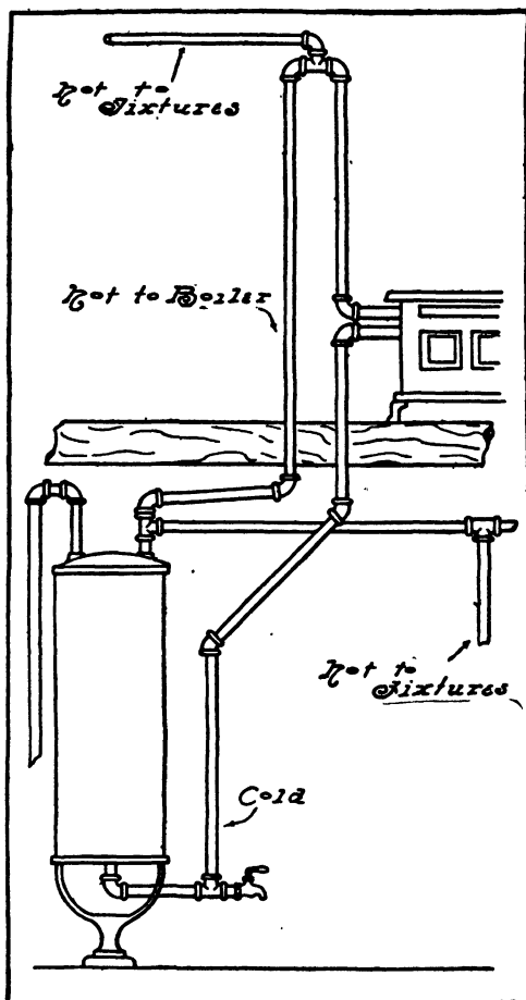
FIG. 307.—Heating of Range Boiler on Floor Below Range.
