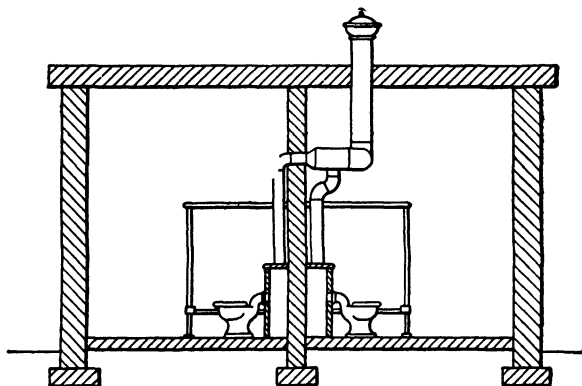
FIG. 172.—Local Ventilation for Comfort Station or Similar Toilet Building.
