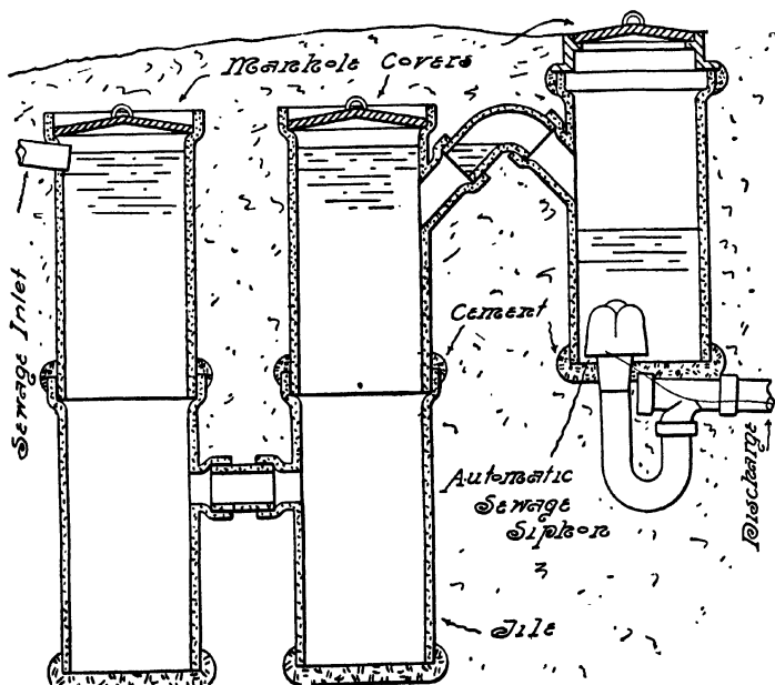
FIG. 222.—Septic Tank and Automatic Sewage Siphon.
