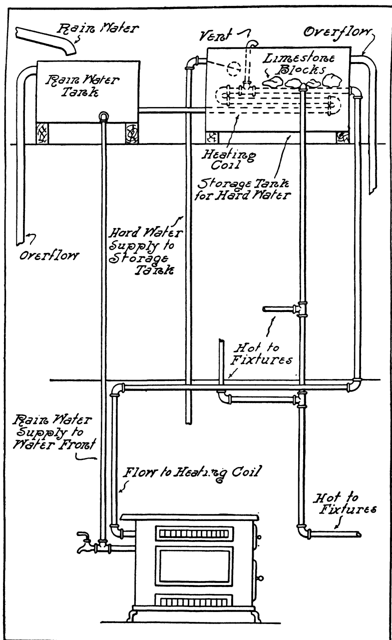
FIG. 321.—Method of Preventing Deposit of Lime in Range Connections.
