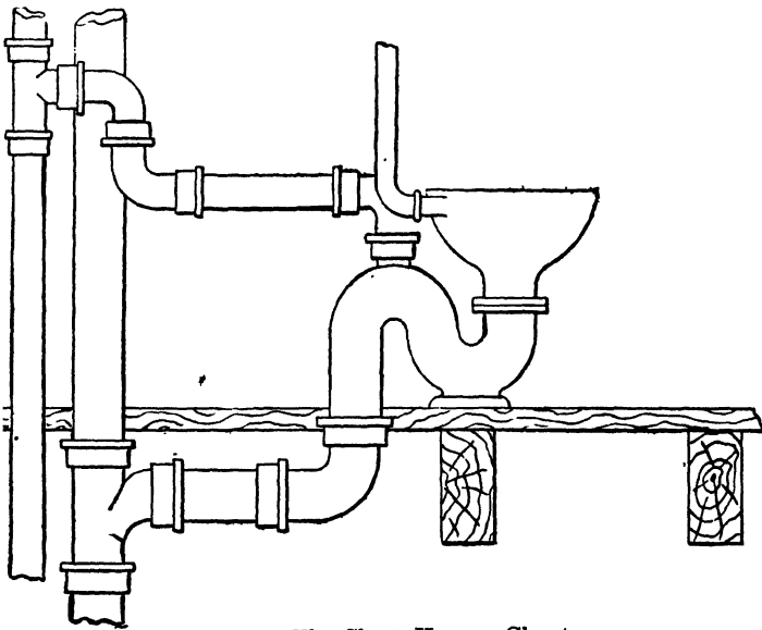
FIG. 129.—The Short Hopper Closet.
