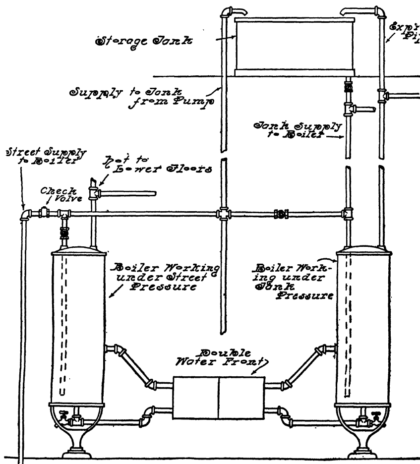
FIG. 320.—Two Single Boilers Doing Work of Double Boiler.
