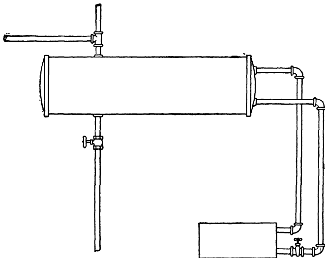
FIG. 277.—Wrong Connections for Horizontal Range Boiler.
