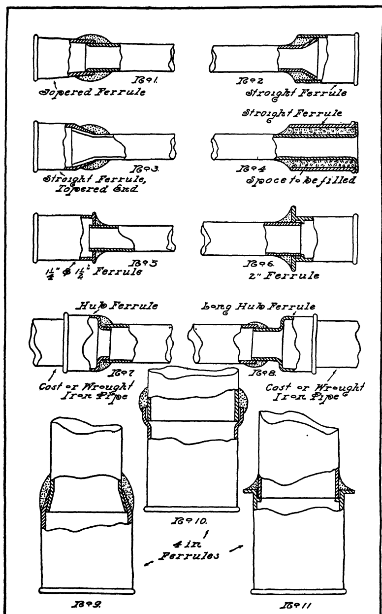
FIG. 18.—Wiping Brass Ferrules.
