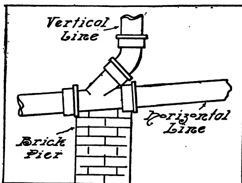
FIG. 106.—Horizontal Line of Pipe Supported by Pier
