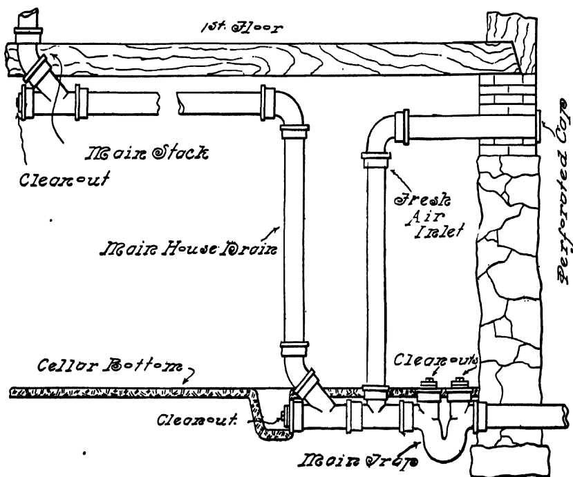
FIG. 103.—Line of House Drain Run Overhead.
