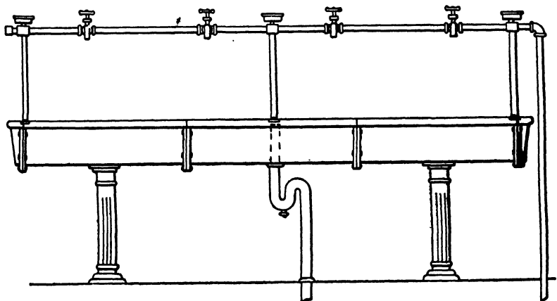
FIG. 208.—Sectional Wash Sink.
