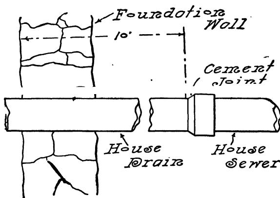
FIG. 74.—House Drain through Cellar Wall.
