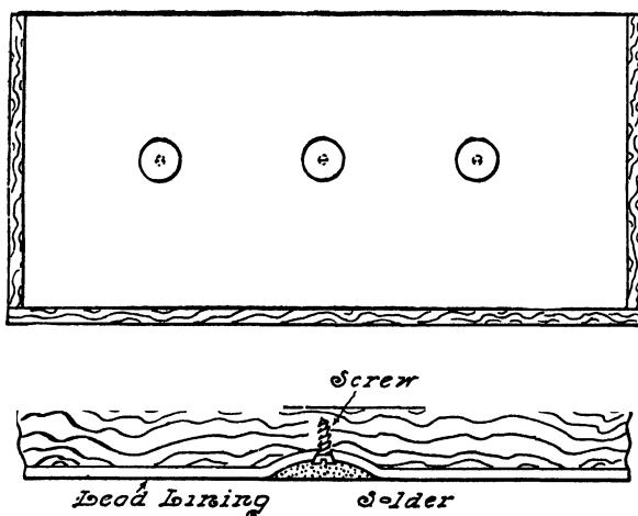
FIG. 21.—Supporting of Lead Lining on Sides of Tank.
