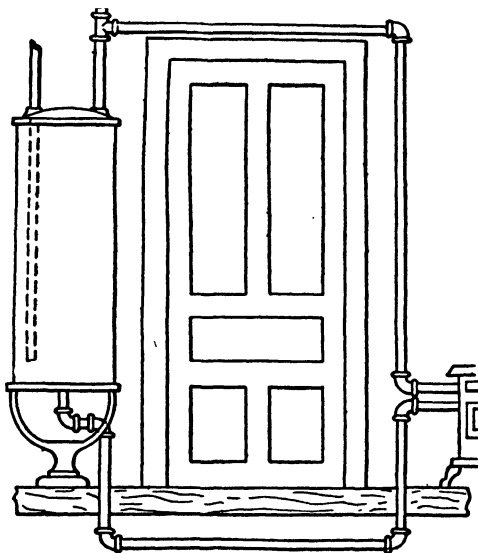
FIG. 299.—Boiler Heated by Range with Door Between. Correct Method.
