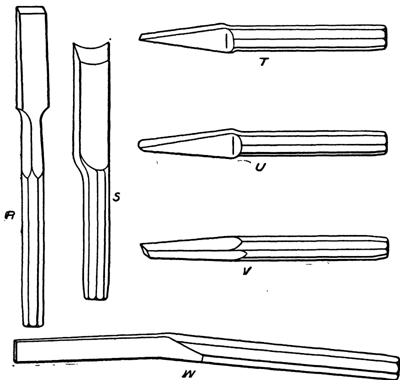
FIG. 6.—Special Plumbers' Chisels.
