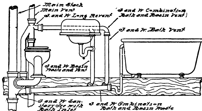
FIG. 125.—Separate Waste Entrances by Means of Special Fittings.
