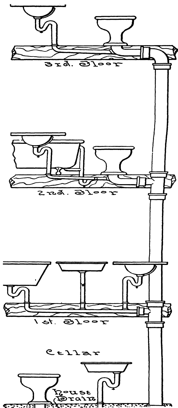
FIG. 37.—Siphonage in Unventilated Plumbing System.
