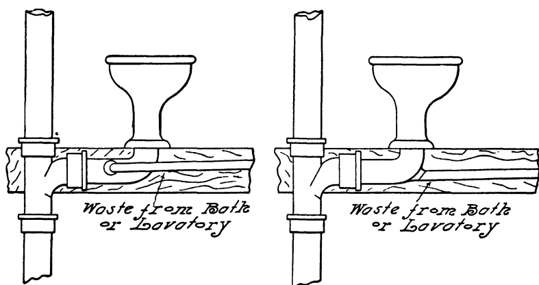
FIG. 93.—Connection of Waste Pipe into Lead Bend.
