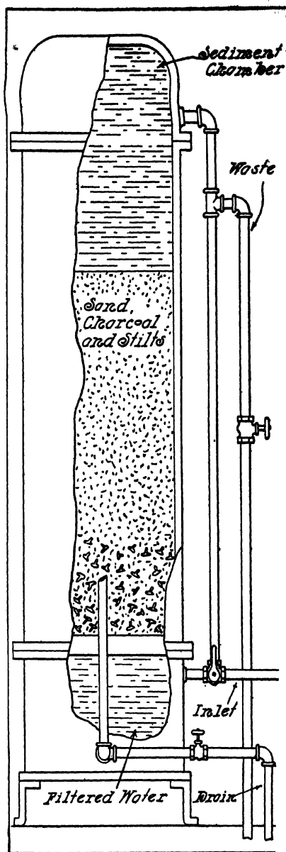
FIG. 234.—Filter for Domestic or Commercial Use.
