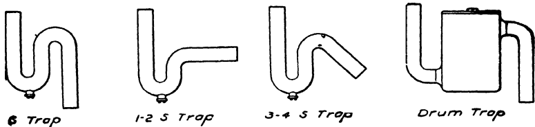
FIG. 27.—Fundamental Types of Traps.
