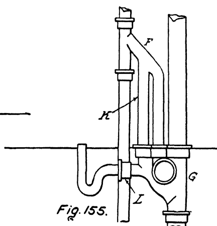
FIGS. 152-155.—The Use of Special Water-Closet Waste and Vent Fittings.
