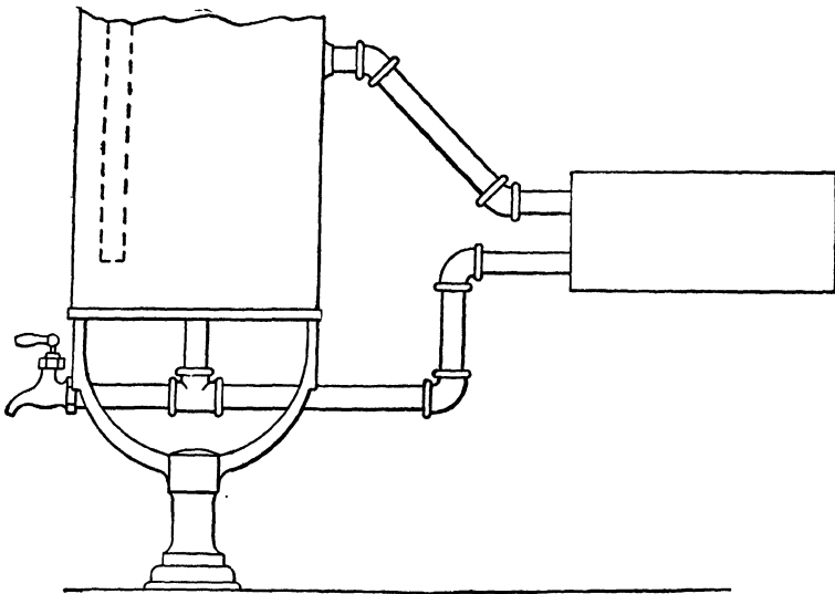
FIG. 270.—Use of 45 Degree Elbows on Range Connections.
