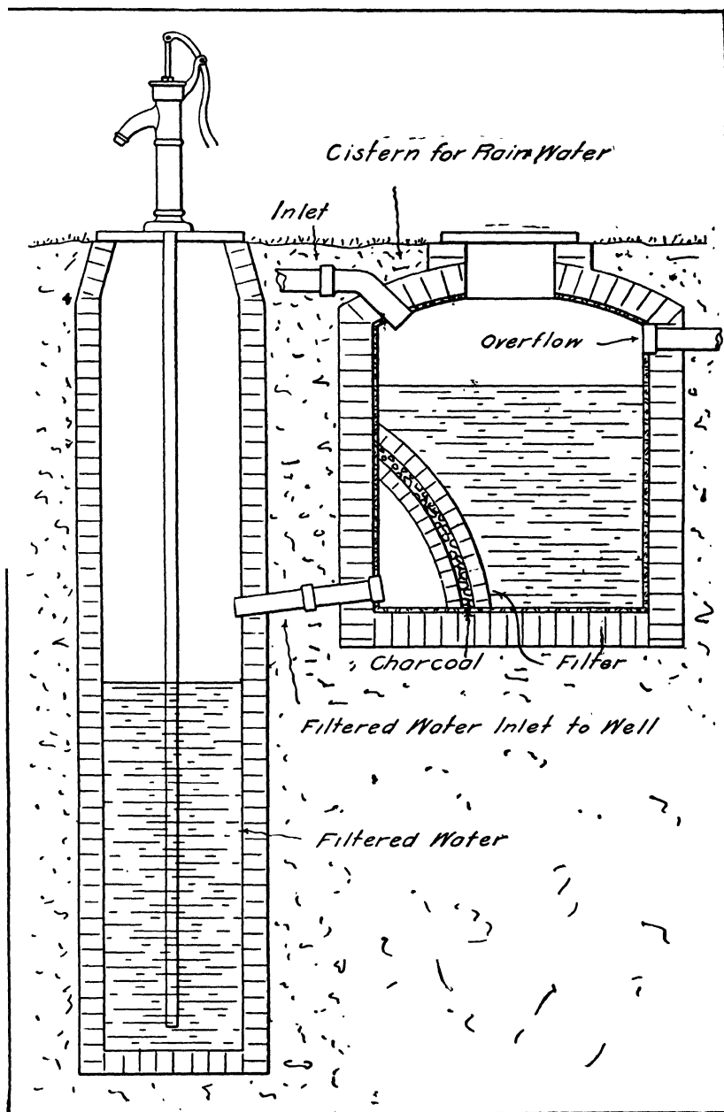
FIG. 247.—Filtered Rain Water from Well.
