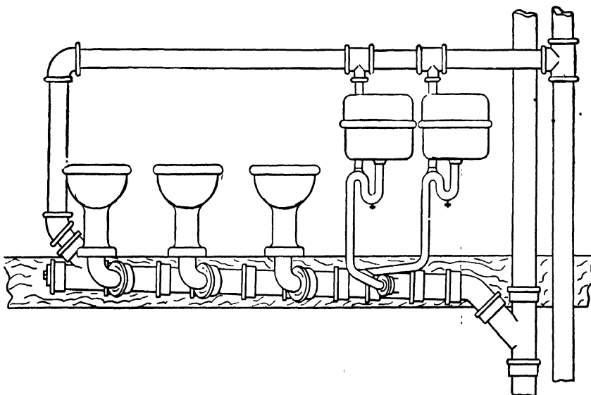
FIG. 200.—The Loop Vent.
