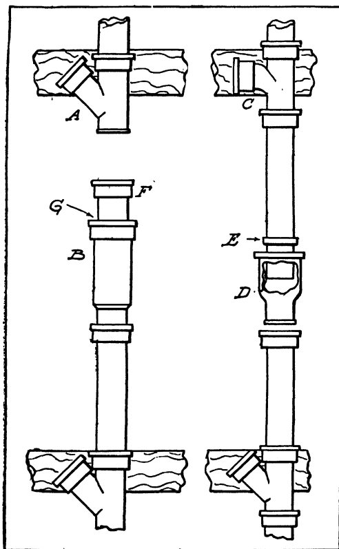
FIG. 94.—The Use of Insertable Fittings.
