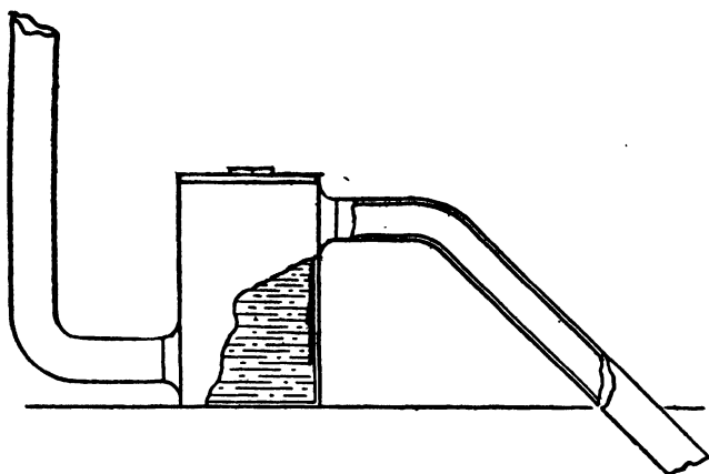
FIG. 334.—Destruction of Trap Seal by Capillary Action.
