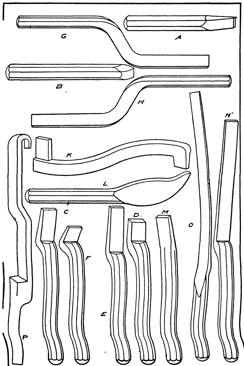
FIG. 5.—Various Styles of Calking Tools
