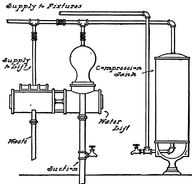
FIG. 324.—Water Lift Used on Direct Pressure System.
