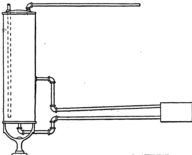
FIG. 269.—Flow Pipe of Range Connection Pitching in Wrong Direction.
