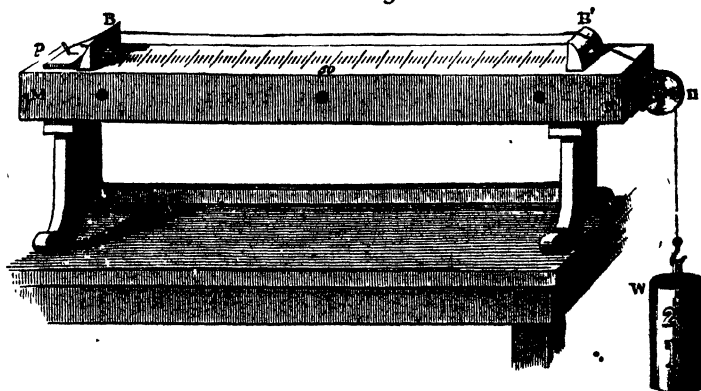
THE MONOCHORD.
