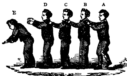
TYNDALL'S ILLUSTRATION
