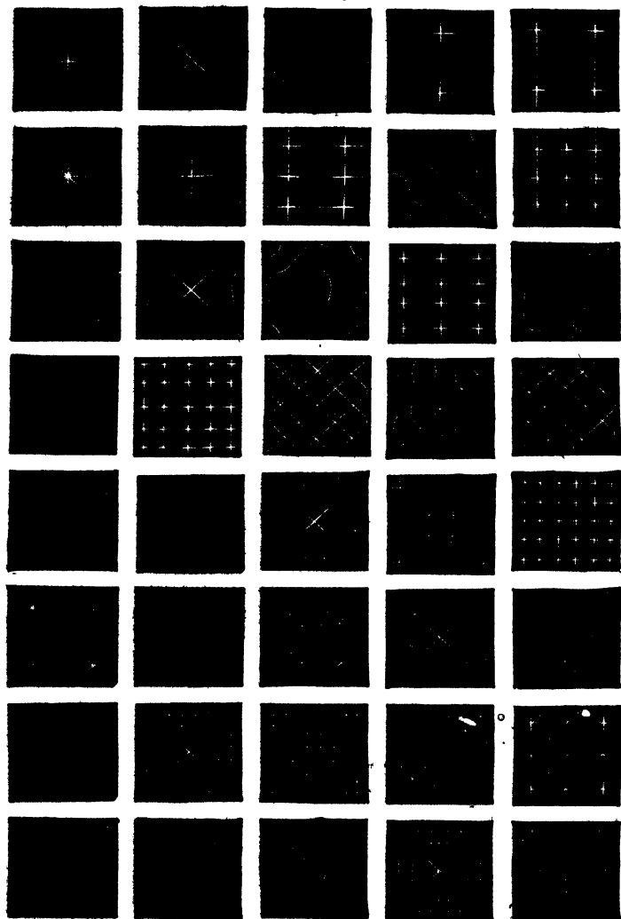
CHLADNI'S VIBRATIONS OF SQUARE PLATES.
