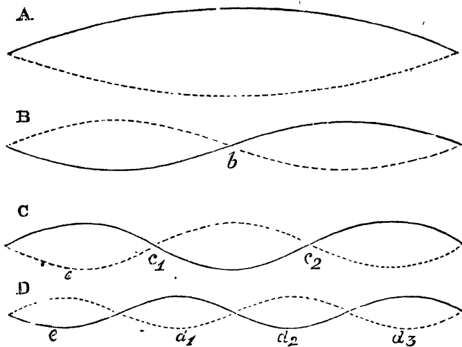
VIBRATIONS OF STRINGS.
