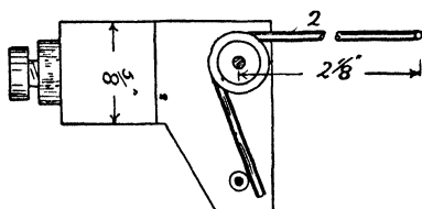
Fig. 149.—Elevation of Pendulum Fitting
