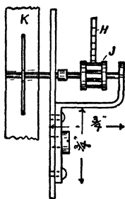
Fig. 195. — Enlarged Detail showing Mounting of Fly
