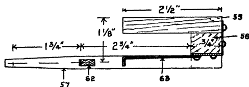
Fig. 103.—Plan of Contact Board
