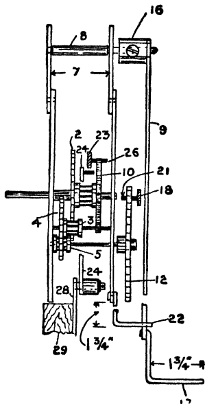
Fig. 77. Side View showing Position of Wheels for Clock with Chime
