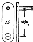
Figs. 145 and 146.—Adjustable Support for Pawl
