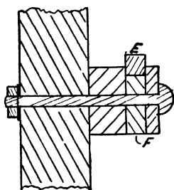
Fig. 118.—Vertical Section
