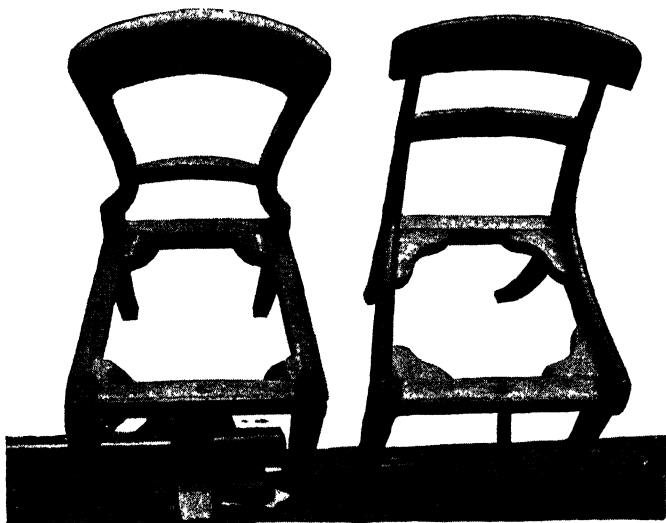
Fig. 47.—Chairs strengthened with Corner Blocks
