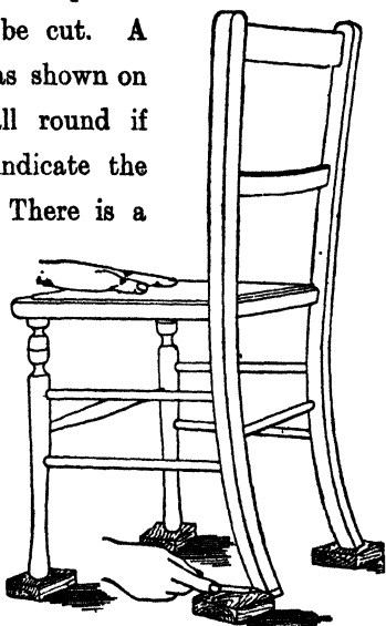
Fig. 79.—Method of Levelling Legs
