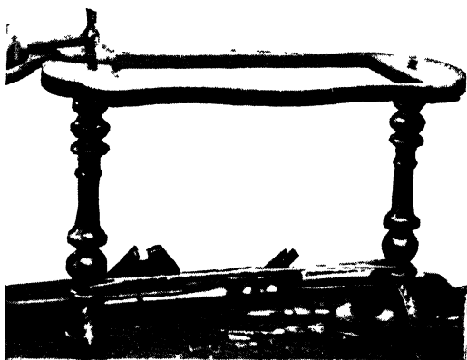
Fig. 102.—Method of Wedging Pillar and Frame Joints and Cramping Rail Joints
