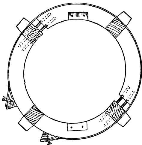
Fig. 164.—Method of Cramping Desk Chair Seat
