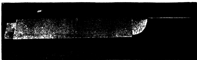
Fig. 133.—Repaired Corner Post Ready for Fixing in Position
