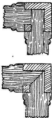
Figs. 85 and 86.— Incorrect and Correct Methods of Joining Rails
