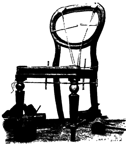
Fig. 33.—Joints Cramped up with Strings and Winders
