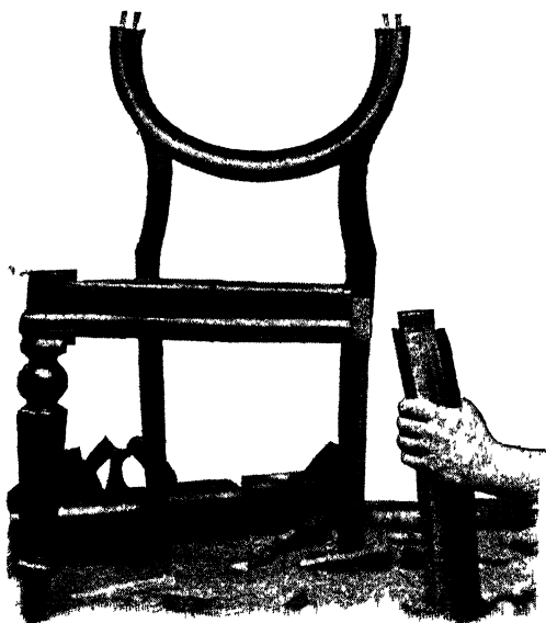
Fig. 32.—"Blind Wedging" of Mortice-and-tenon Joints
