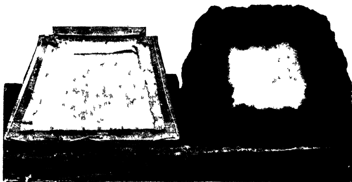
Figs. 51 and 52.—One Seat Frame Webbed and Canvased, Another with Hair Stuffed under Strings
