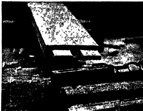
Fig. 99. — Mor- tice-and-tenon Joint ready for Gluing up
