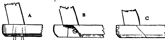
Fig. 14.—Parts of Back Uprights and Chair Seat
