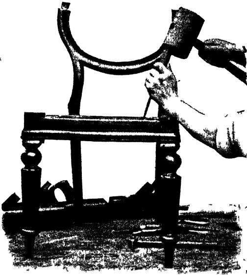
Fig. 30.—Marking Chair Braces and Rails with Chisel
