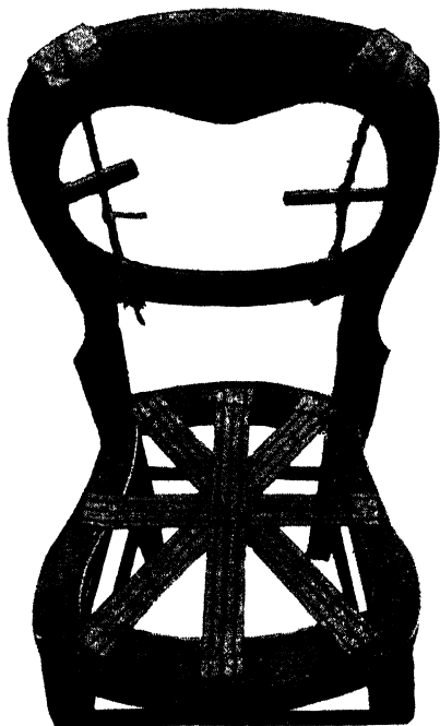
Fig. 22.—Cramping Rail Joints
