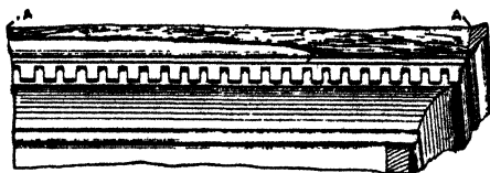
Fig. 136.—Portion of Side Cornice Moulding with Piece Broken Out (A to A)
