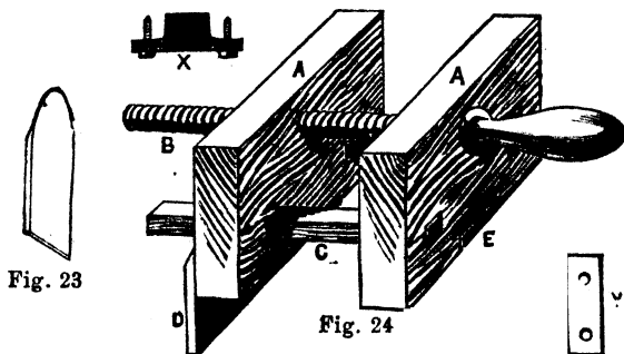
Fig. 23.—Plough Knife. Fig. 24.—Plough.
