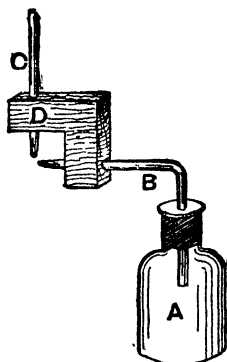
Fig. 48.—Sprayer for Colouring Book Edges.
