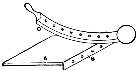
Fig. 25.—Strawboard Cutter.
