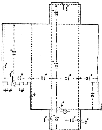
Fig. 96.—Pattern for Picnic Teapot.
