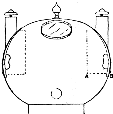
Fig. 277.—Front Elevation of Lamp for Binnacle Cover.
