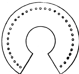
Fig. 270.—Pattern for Parts G and H (Fig. 265).
