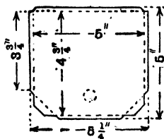
Fig. 245.—Top and Bottom of Wall Lamp Body.
