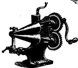
Fig. 55.—Cone Rollers.
