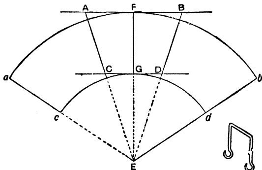
Fig. 138.—Setting out Body for Nose-tin.
