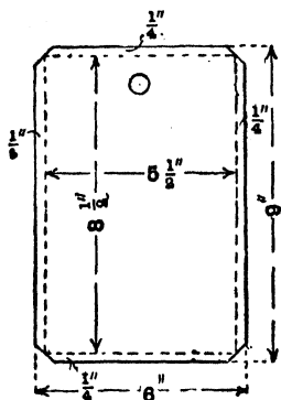
Fig. 243.—Back of Wall Lamp.
