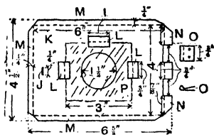
Fig. 86.—Door of Letter-box.
