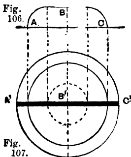
Figs. 106 and 107.—Section and Plan of Hollowed Circle.
