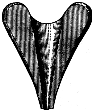
Fig. 161.—Finished Boss of Saucepan.
