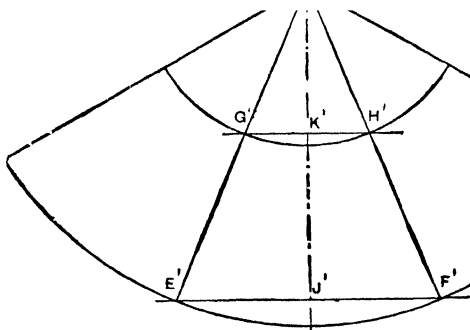
Fig. 169.—Bottom Part of Inner Saucepan.
