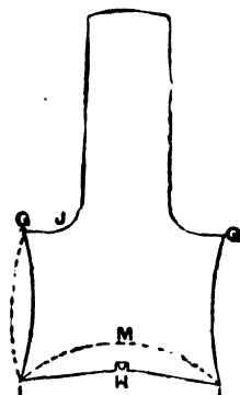
Fig. 205.—Spout Pattern for Oval Kettle.
