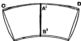
Fig. 121.—Pattern of Frustum of Curved Cone.
