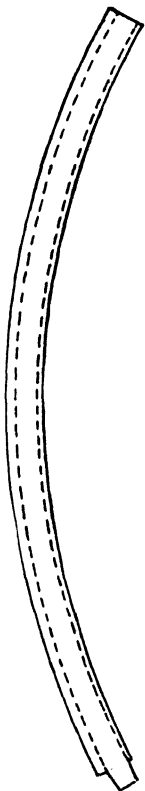
Fig. 176.—Rim Pattern for Saucepan Cover.
