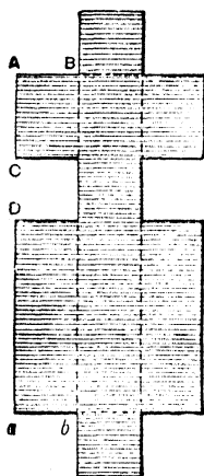
Fig. 73.—Part Pattern for Cross Flower Tray.
