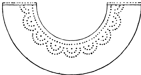
Fig. 126.—Tin Colander. Fig. 127.—Pattern for Colander Body.
