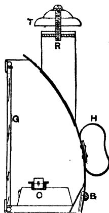
Fig. 278.—Enlarged Section of Lamp for Binnacle Cover.
