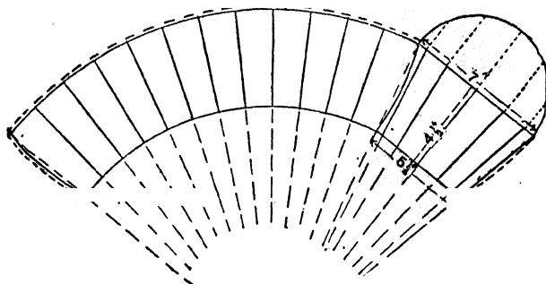
Fig. 146.—Pattern for Tea-urn.
