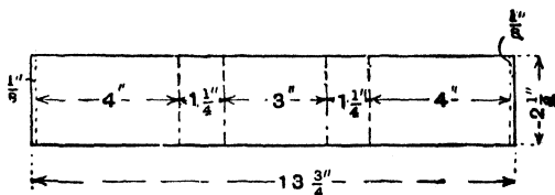
Fig. 244.—Body of Wall Lamp.
