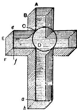
Fig. 72.—Plain Cross Flower Tray.
