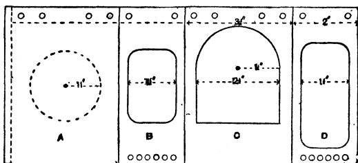
Fig. 257.—Body Pattern of Hand Lamp.
