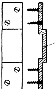
Fig. 248. Fig. 249. Figs. 248 and 249.— Elevation and Section of Socket or Staple.
