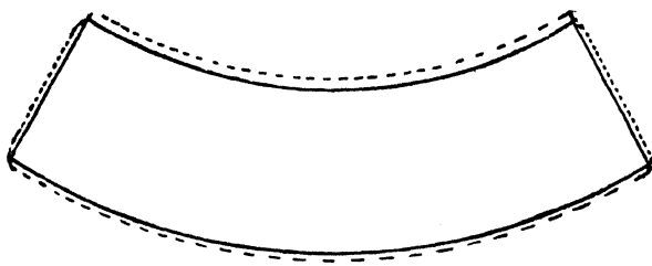
Fig. 171.—Pattern for Saucepan with Tapering Sides.
