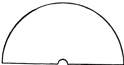
Fig. 182.—Pattern for Steam Spreader for Bronchitis Kettle.
