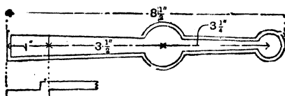
Fig. 221.—Latch of Oven Door.
