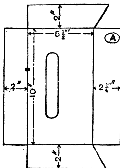
Fig. 214.—Oil Stove Reservoir Pattern.
