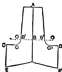
Fig. 192.—Kettle Spout Pattern.
