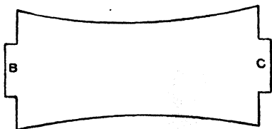
Fig. 253.—Pattern for Wind-guard for Cart Lamp.
