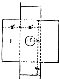
Fig. 262.—Reservoir Pattern for Hand Lamp.
