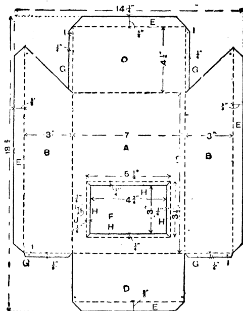
Fig. 85.—Letter Box Pattern.
