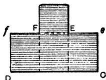
Fig. 74.—Part Pattern for Cross Flower Tray.
