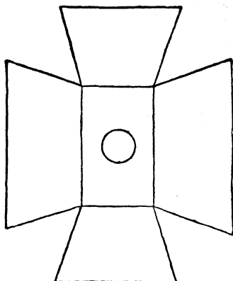
Fig. 255.—Pattern for Oil Container for Cart Lamp.
