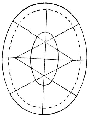
Fig. 203.—Pattern for Oval Kettle Top.
