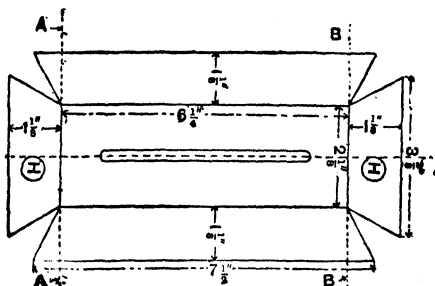
Fig. 209.—Base of Oil Stove Burner.
