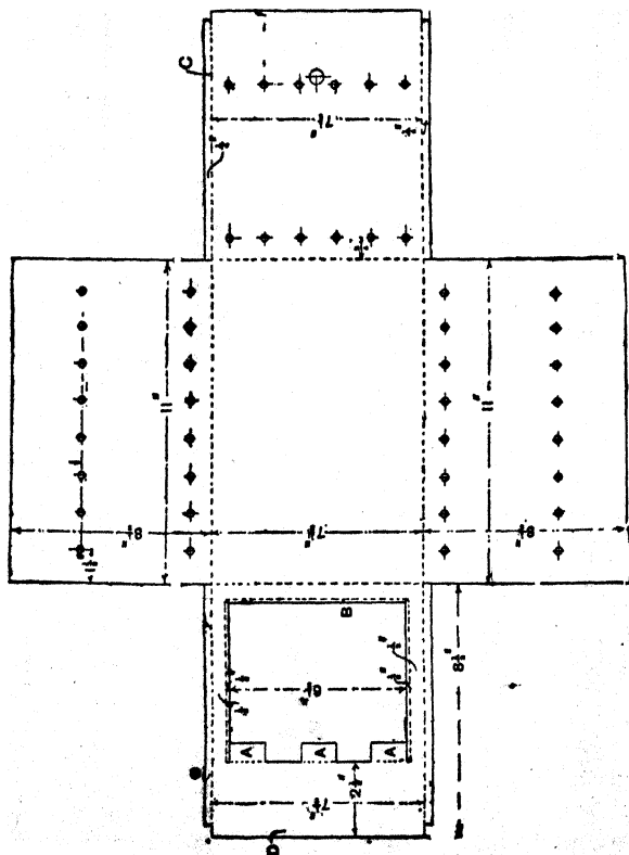
Fig. 88.—Pattern for Body of Picnic Outfit.
