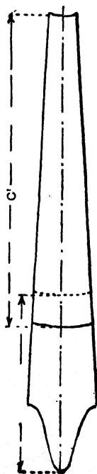
Fig. 180.—Spout Pattern for Bronchitis Kettle.
