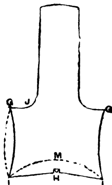
Fig. 205.—Spout Pattern for Oval Kettle.
