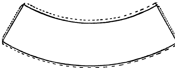
Fig. 171.—Pattern for Saucepan with Tapering Sides.
