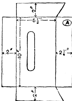
Fig. 214.—Oil Stove Reservoir Pattern.
