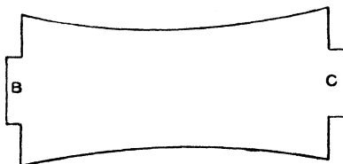
Fig. 253.—Pattern for Wind-guard for Cart Lamp.
