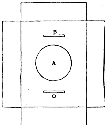
Fig. 252.—Pattern for Top of Cart Lamp.
