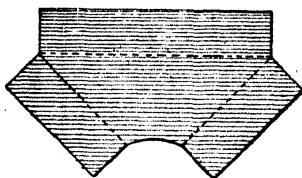
Fig. 78.—Pattern for Maltese Cross.
