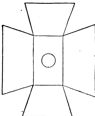
Fig. 255.—Pattern for Oil Container for Cart Lamp.
