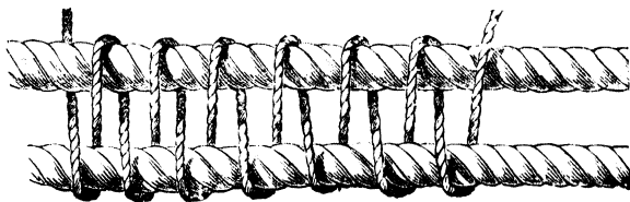
Fig. 78.—Nippering.
