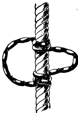
Fig. 125.—Selvagee fastening Block to Rope.
