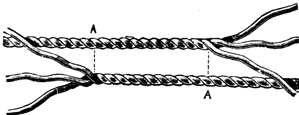
Fig. 118.—Beginning Cut Splice.
