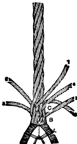
Fig. 185.—Left-handed Splice, all Ends Tucked Onoa.
