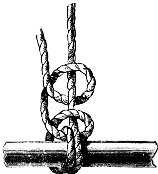
Fig. 29.—Fisherman's Bend.
