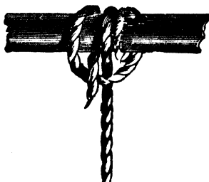
Fig. 28.—Magnus Hitch.
