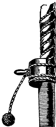
Fig. 127.—Serving.
