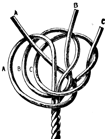
Fig. 90.—Beginning Matthew Walker Knot.
