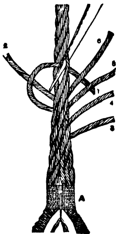
Fig. 180.—Partly-finished Splice.
