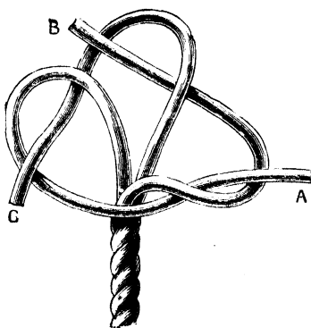
Fig. 83.—Wall Knot.
