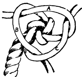
Fig. 144.—Crown.
