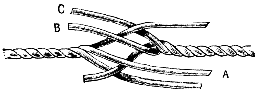
Fig. 113.—Beginning Short Splice.
