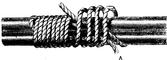
Fig. 76.—Finishing off Whipping.
