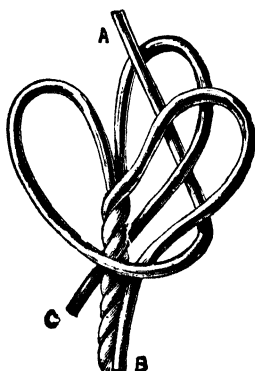
Fig. 92.—Beginning Diamond Knot.
