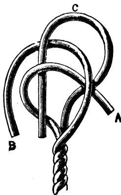
Fig. 85.—Beginning Crowning.
