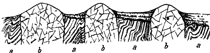
FIG. 70.—Section across the three Dirrington Laws, Berwickshire
