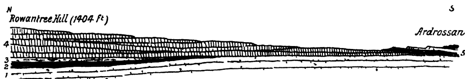
FIG. 121.—Diagram illustrating the thinning away southwards of the lavas of the Clyde Plateau between Largs and Ardrossan. Length about 10 miles.
