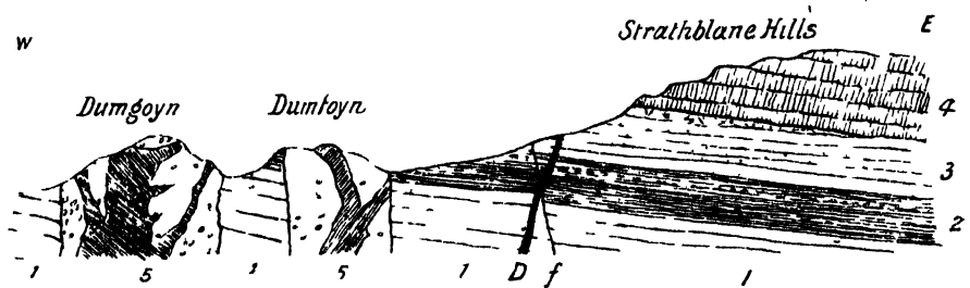
FIG 127 —Section across the vents Dumgoyne and Dumfryn, and the edge of the Clyde plateau above Strathblane, Stirlingshire
