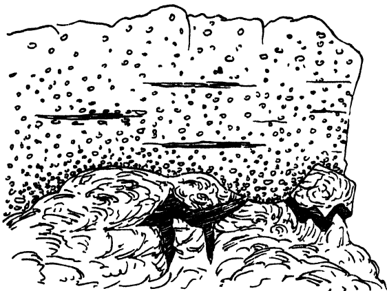
FIG 76 — Andesite with sand-tone veinings and overlying conglomerate Todhead, south of Caterline, coast of Kincardineshire
