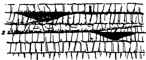
FIG. 21.—Diagram illustrating volcanic eruptions on a land surface.
