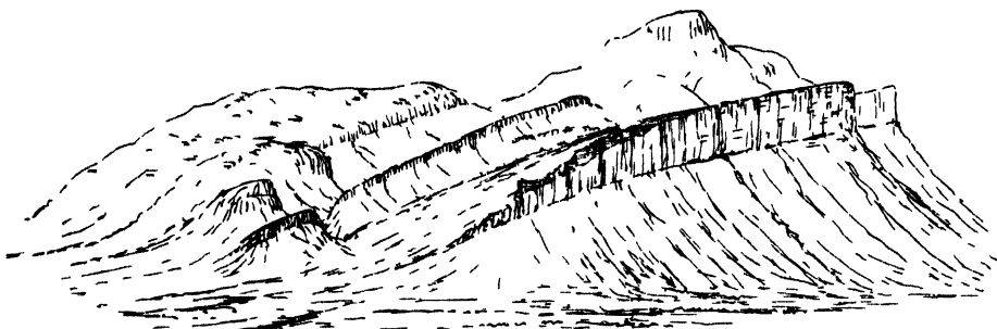
FIG 112.—View of Arthur Seat from Calton Hill to the north
