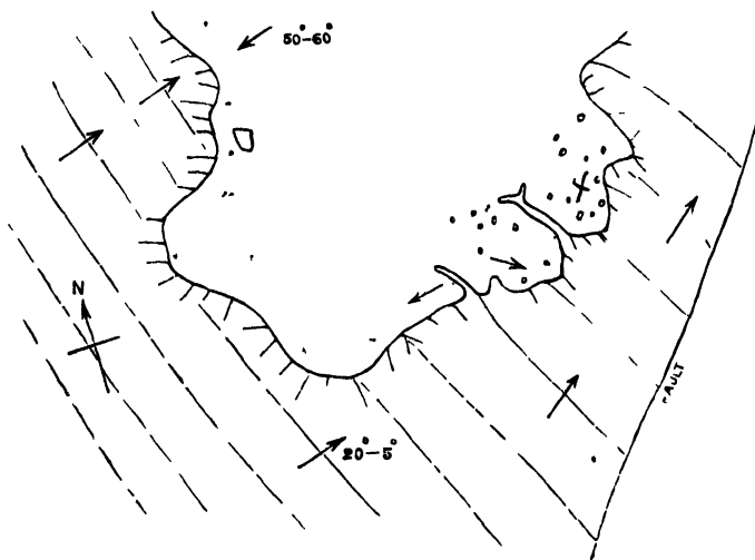
FIG. 126.—Ground-plan of tuff neck, shore east of Dunbar
