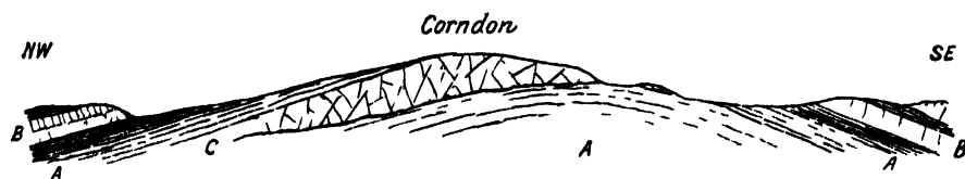
FIG. 50.—Section across the anticline of Corndon. 1
