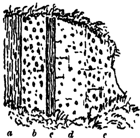
a. 41 —Section showing the interstratification of tuff and conglomerate above Lower Mill, St. David's
