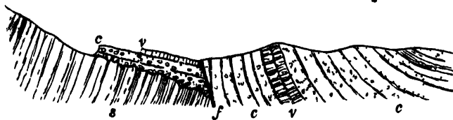
FIG 77 —Section across the Boundary fault of the Highlands at Glen Turril, Perthshire s, Crystalline schists of the Highlands, c c, conglomerates and sandstones (Lower Old Red Sandstone) with interstratified volcanic rocks (v r), f, fault
