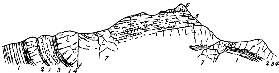
FIG 56 —Section of Snowdon 4
