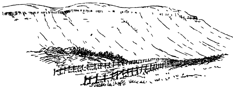
FIG. 111.—Corston Hill—a fragment of the Midlothian Plateau, seen from the north. The volcanic rocks form a cake on the top, the slopes lying across the edges of the Calcareous Sandstones.
