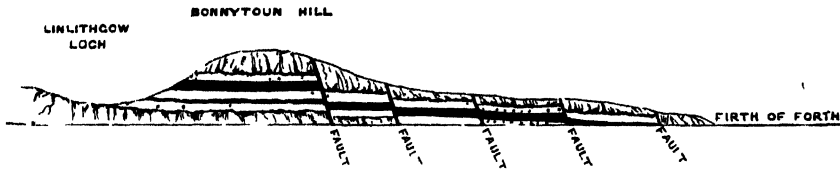
FIG 157 —Section from Linlithgow Loch to the Firth of Forth
