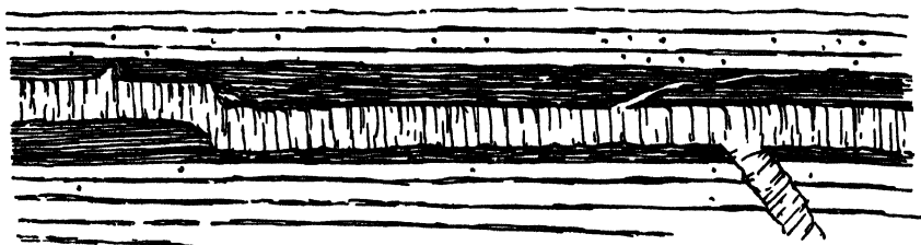
FIG 33 —Section of Sill or Intrusive Sheet
