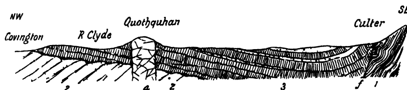
FIG. 92 — Section across the southern part of the Biggar volcanic group from Covington to Culter
