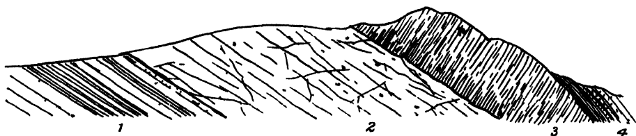
FIG 115 —Section of Craiglockhart Hill, Edinburgh
