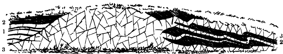
FIG. 167.—Boss of diabase cutting the Burleighhouse Limestone and sending sills and veins into the overlying shales. Railway cutting, West Quarry, East Calder, Midlothian.
