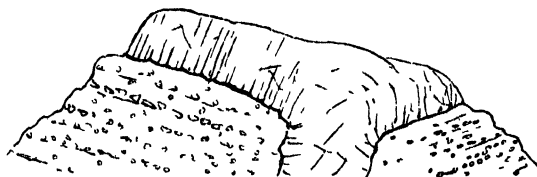
FIG 131.—Section of south end of Dumbuck Hill East of Dumbarton
