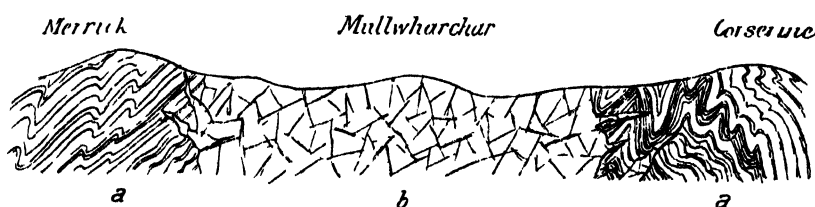
FIG 69 —Section of the granite core between Merrick and Corsevine a, Silurian greywackes, gills and shales, b, granite
