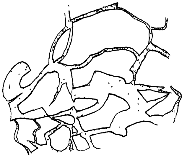
FIG 66 —Ground plan of reticulated cracks in the upper surface of an Old Red Sandstone lava filled in with sandstone Red Head, Forfarshire
