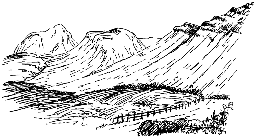
FIG 123 View of the two necks Dumgoyn and Dumfoyn, Stirlingshire, taken from the south. These two necks form a conspicuous feature in front of and below the lava plateau, a portion of which is shown on the right hand. The ground plan of the same necks is shown in Fig 124.
