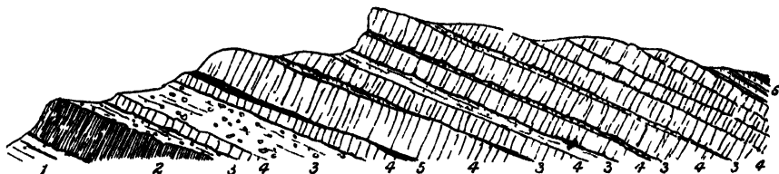
FIG. 118.—Section of Calton Hill, Edinburgh
