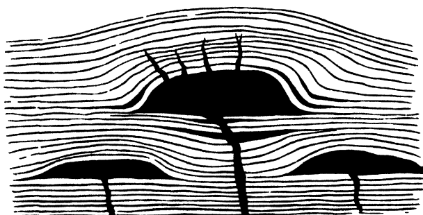
FIG. 34 — Ideal section of three Laccolites (After Mr. Gilbert.)
