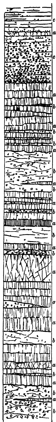
FIG. 81.—Diagram of the volcanic series of the Western Oehl Hills
