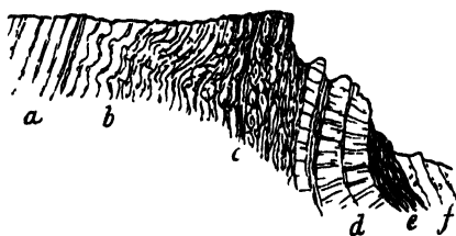
FIG 54—Section of part of the Arenig volcanic group, stream south of Bennane Head, Ayrshire
