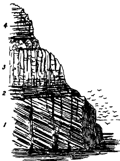
FIG 103—Section of the volcanic zone in the Upper Old Red Sandstone, Cam of Hoy, Orkney
