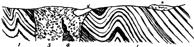
FIG 175 —Diagram to show the position of a mass of Upper Old Red Sandstone which has fallen into the great vent near Tudhope Hill, east of Mossburn
