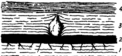
FIG. 151.—Ejected volcanic block in Carboniferous strata, Burntisland
