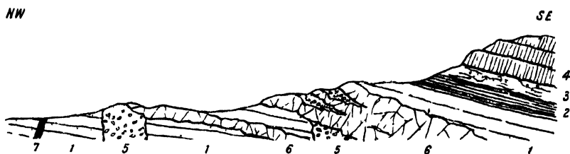
Fig 136 —Trachytic sills, Knockvadie, Kilpatrick Hills
