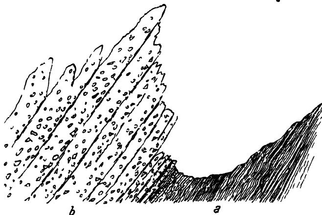
FIG 61 —Blue shale or slate passing into volcanic breccia east of Porth Padrig, near Carmel Point, Anglesey
