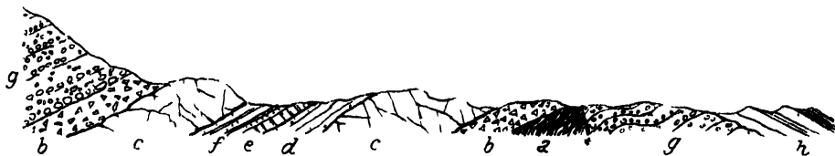
FIG 64.—Diagram of the general relations of the different groups of rock in the Lower Silurian volcanic district along the western shore of Lough Mask
