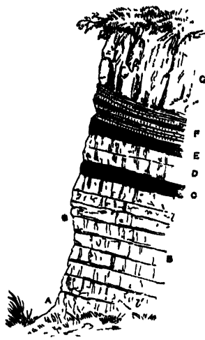
FIG 156 — Section in Wardlaw Quarry, Lamlithgowshire
