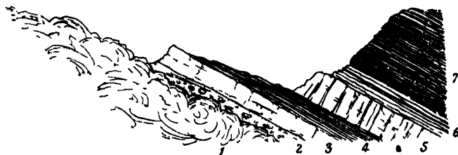
FIG. 154.—Section of the upper surface of a diabase ("leekstone") sheet, Skolhe Burn, south east of Bathgate.
