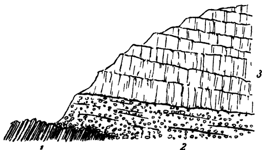
FIG 100.—Section of lava escarpment at Benn Lora, north side of mouth of Loch Etive, Argyllshire.
