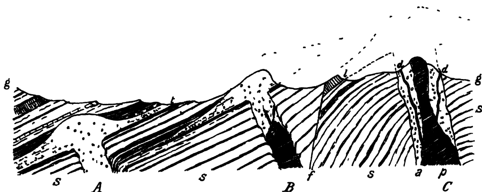
FIG 31.—Diagram illustrating the gradual emergence of buried volcanic cones through the influence of prolonged denudation
