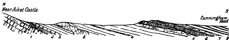
FIG 173 —Section across the Upper Volcanic Band of north Ayrshire. Length about four miles.
