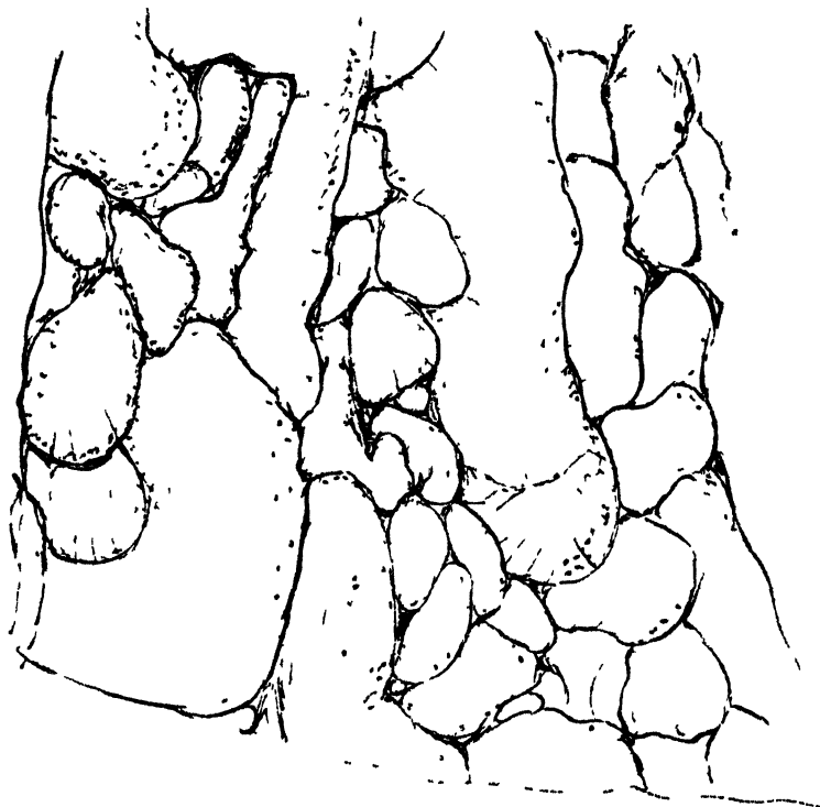
FIG 51 —Structure in finely amygdaloidal diabase lava, south of mouth of Stinchar River, Ayrshire The fine dots and circles mark the lines of amygdaloides
