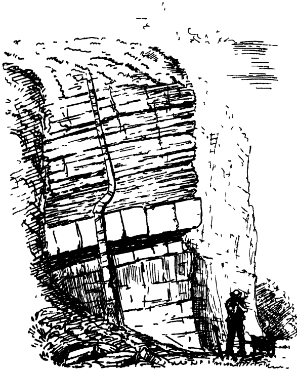
FIG 169 — Dyke rising through the Hurlet Limestone and its overlying shales. Silvermine Quarry, Lanlithgowshire
