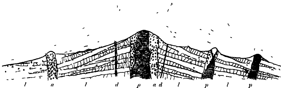
FIG 16 —Effects of denudation on a Vesuvian cone
