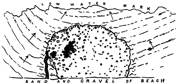
FIG 106 —Ground plan of volcanic neck piercing the Carthness Flagstone series on the beach near John o' Groat's House
