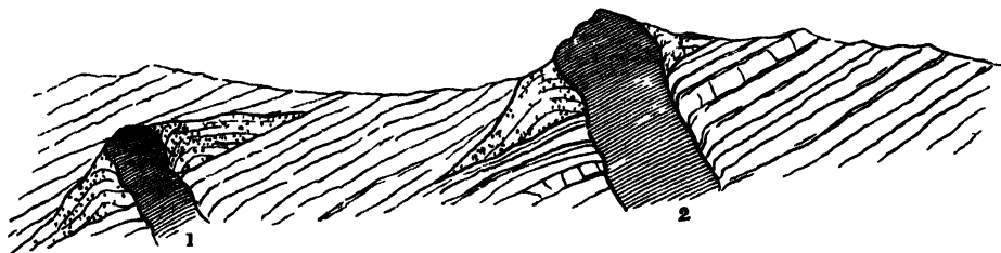
FIG 147.—Diagram to illustrate how Volcanic Necks may be concealed and exposed.
