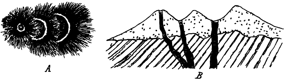
FIG 29 —Successive shiftings of vents giving rise to double or triple cones
