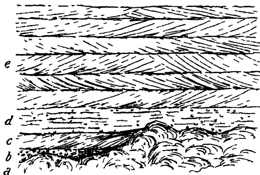
FIG. 75.—Section showing the top of the volcanic series at the foot of the precipice of the Red Head, Forfarshire
