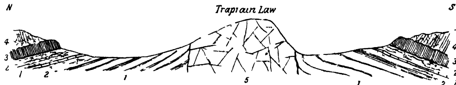
FIG 132 —Section across the East Lothian plateau to show the relative position of one of the necks
