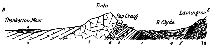
FIG. 93 — Section from Thankerton Moor across Tinto to Lamington
