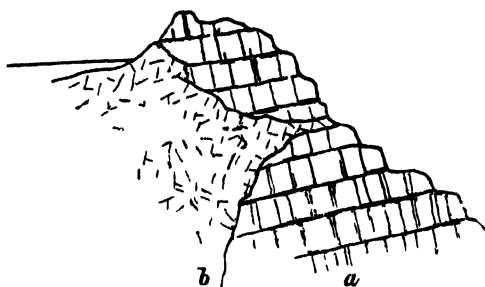
FIG 354 —Section at head of Allt na Searmoin, Mull a, basalts and dolerites with slaggy upper surfaces b felsite
