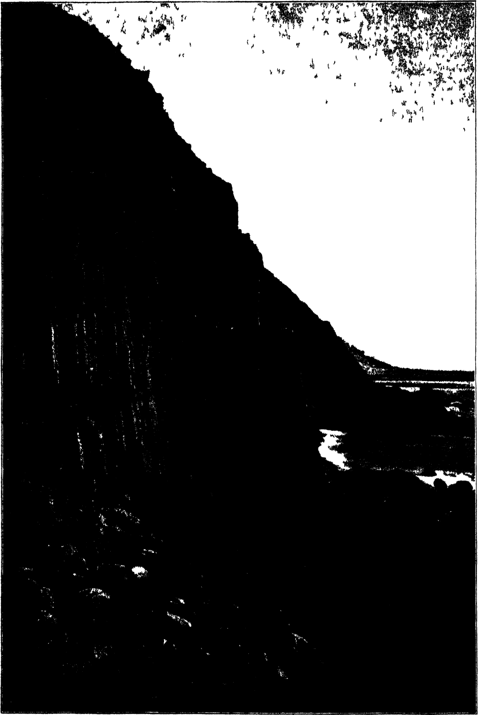
FIG 225 —Columnar basalt in the neck of Kinraig, Elie, seen from the west
