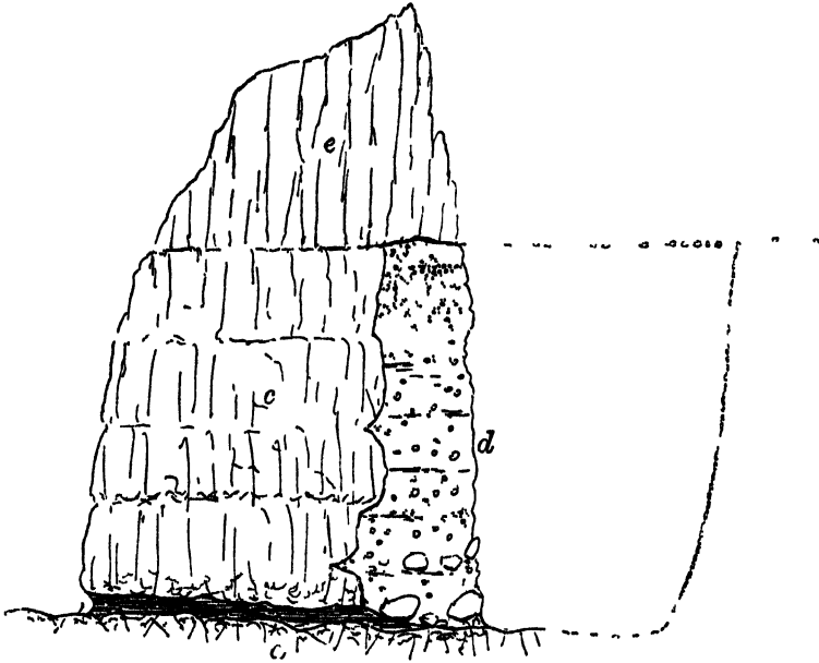
FIG 274 —Section of eastern front of Dun Beag
