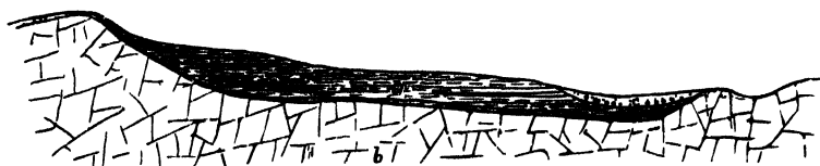
FIG 241 —Section along the line of the Cleveland Dyke at Cliff Ridge, Guisbrough (G. Barrow) Scale, 12 inches to 1 mile
