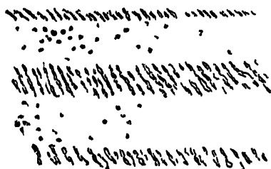
FIG 260 —Banded amygdaloidal basalt showing layers of elongated and steeply inclined vesicles, Macleod's Maidens Skye
