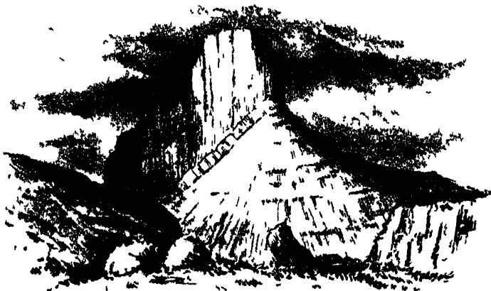
FIG 278 —View of the Scur of Eigg from the east
