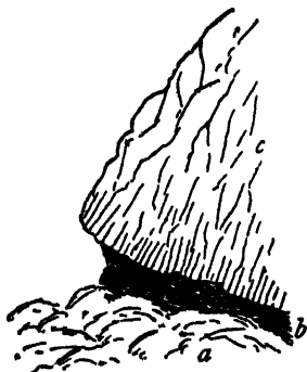
FIG 305 —Section of the Volcanic Series at Ach na Han nait, south of Portree, Skye
