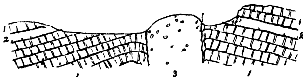
FIG 180 —Section across the smaller volcanic neck and the stratified tuff in Carboniferous Limestone Grange Mill
