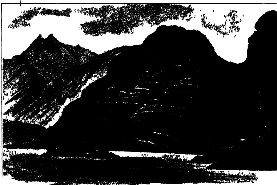
FIG 338 —Sketch of Banded Structure in the Gabbros of the hills at the head of Loch Scavaig
