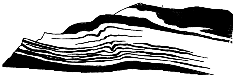
FIG 335 —Banded and puckerred gabbro, Drumm an Eithne Glen Sligachan, Skye
