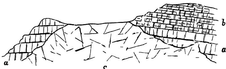
FIG. 355.—Section on south side of Beinn Fhada, Mull. a bedded basalts and dolerites b pale group of Ben More c granophyre
