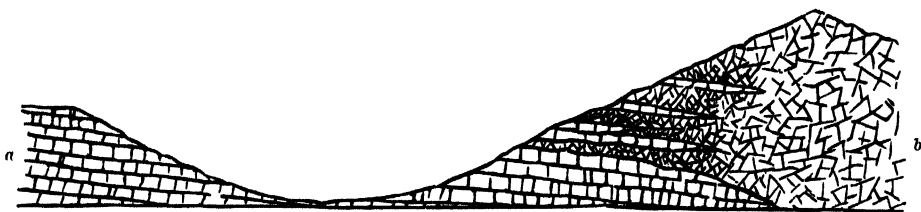
FIG 332—Section across Glen Brittle, to show the general relations of the Bedded Basalts (a) and the Gabbros (b)
