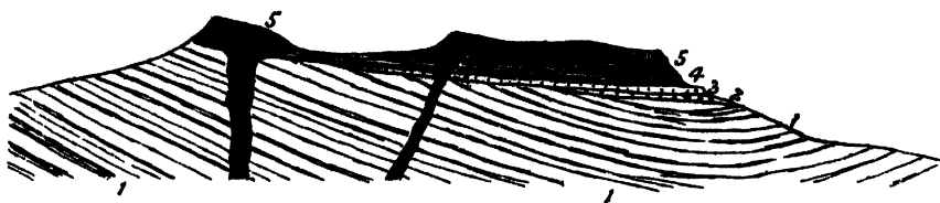
FIG. 232.—Diagrammatic section across Titterstone Cleve Hill
