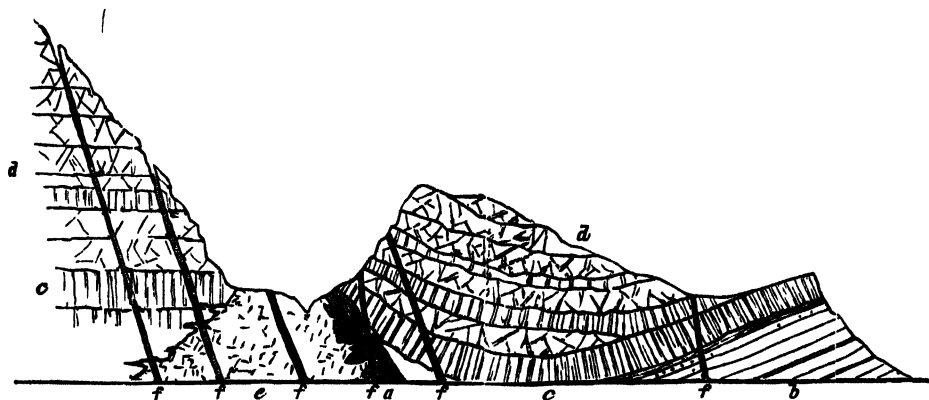
FIG 334.—Section across the Cuillin Hills, Skye
