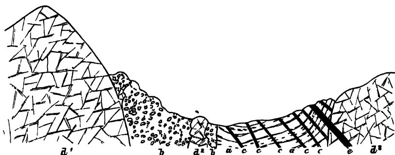
FIG 348 —Section from Beinn Dearg to Beinn an Dubhaich, Skye
