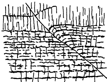
FIG 383 — Reversed fault on the north-east headland of Sando Faroe Isle
