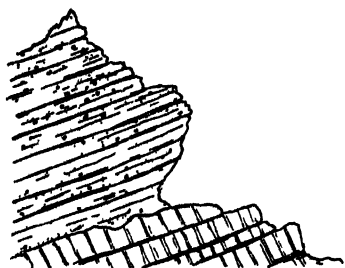
FIG 184 — Limestones passing under stratified tuffs, Poyll Vaaish, Isle of Man
