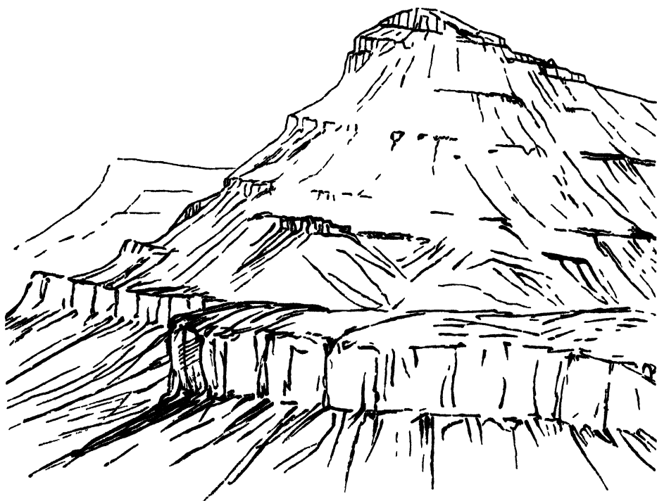
FIG 340 —View of Allival, Rum, sketched from the base of the north east side of the cone
