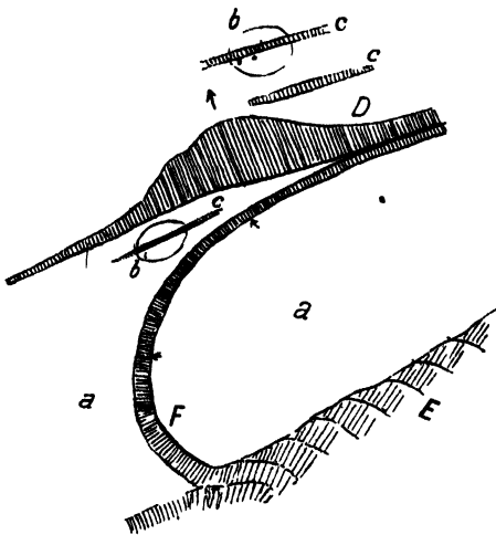
FIG 326 —Ground plan of Sills at Ben Hiant, Ardnamurchan
