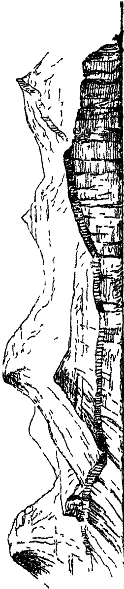
FIG 329.—View of the same Sill seen from the channel opposite the island of Kolter
