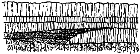
FIG 288 —Dying out of Lava beds, east side of Sando Faroe Isles
