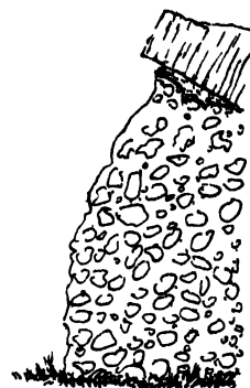
FIG. 231.—Section of agglomerate overlain with sandstone and andesite, Posbury, Crediton
