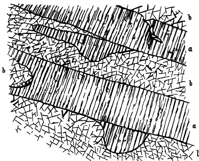
FIG 380.—Section of intruded veins of various acid rocks above River Clachan, Mull
