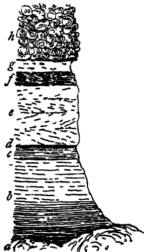
FIG 291 —Section at Frod bonyp, Sudero, Faroe
