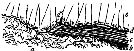
FIG 270 —Section of shales and tuffs, with a coniferous stump lying between two basalt sheets, Cul nam Marbh, Canna
