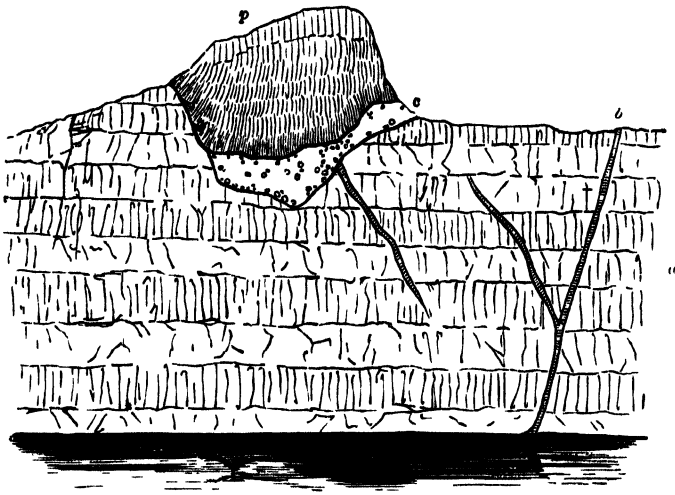
FIG. 279.—Natural Section at the Cliff of Bideann Boidheach, north west end of the Scur of Eigg
