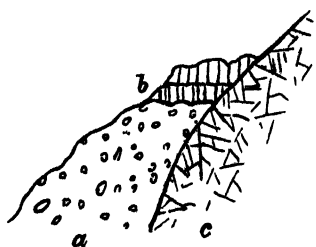
FIG 303.—Diagram to show the probable relations of the rocks on the southern flank of Beinn Dearg Bheag
