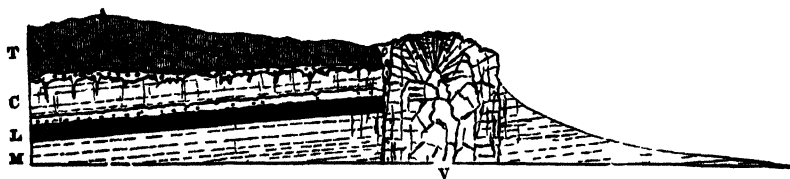
FIG 295 —Section of Volcanic Vent at Carnmony Hill (E. Hull) T, Lower basalt, C, Cretaceous strata, L, Lower Lias, M, Triassic marls, V, Vent
