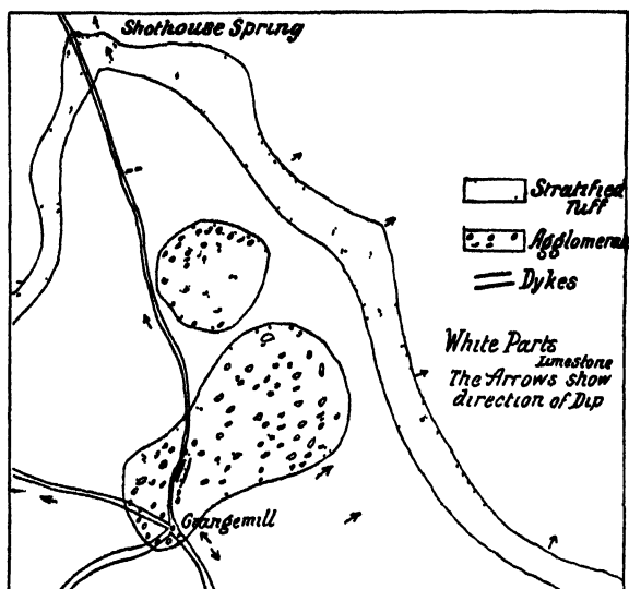
FIG 179 —Plan of necks and bedded tuff at Grange Mill, five miles west of Matlock Bath
