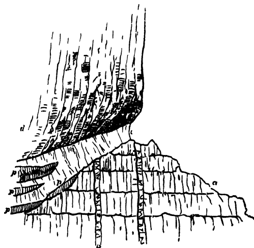
FIG 282 —Section at the base of the Scur of Egg (east end)
