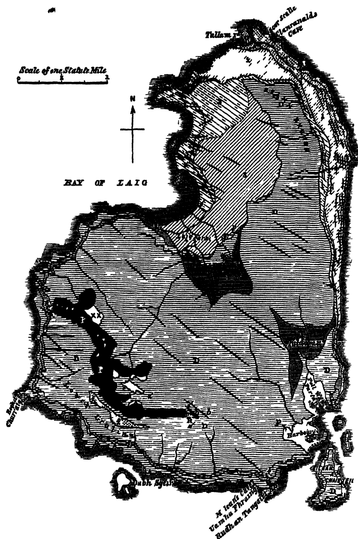
FIG 276 —Geological Map of the Island of Eigg
