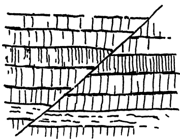
FIG 382 — Reversed fault on the eastern side of Svino, Faroe Isles
