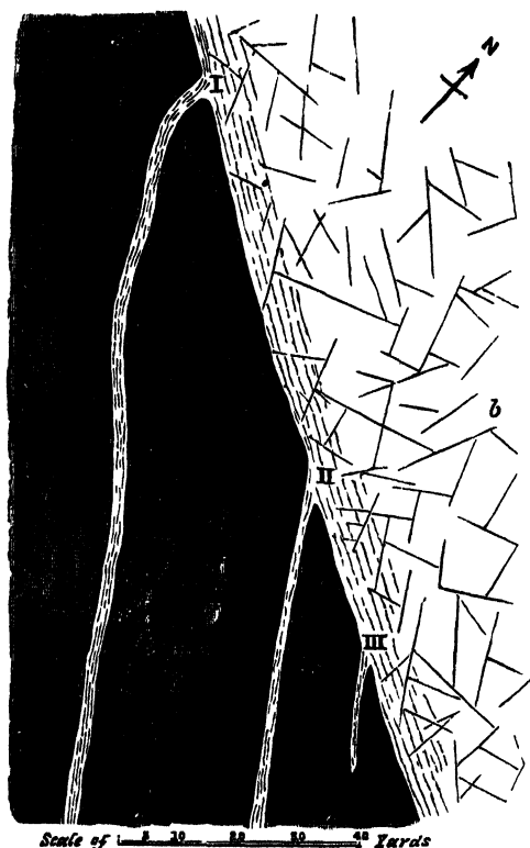
FIG 376.—Plan of portion of the ridge north of Drumnaghnan, Glen Sligachan, Skye, showing three dykes issuing from a mass of granophyre.
