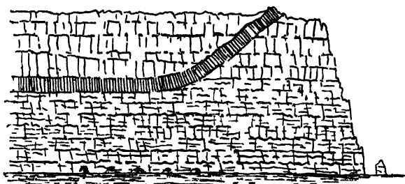
FIG 328 —Sill traversing bedded Basalts cliffs of Stromo at entrance of Vaagofjord
