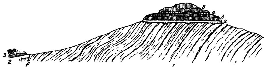
FIG 263 —Section of Knocklayd, an outlier of the Antrim basalt plateau lying on Chalk
