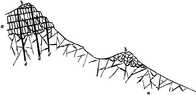
FIG. 359 — Section at Creag na h Iolaire, Glen More, Mull, showing basalts and gabbros resting on and pierced by granophyre
