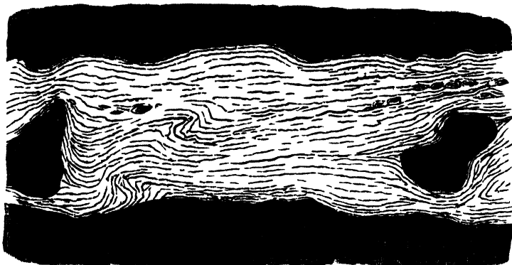
FIG 378 —Plan of pale granophyric dyke, with spherulitic and flow structure, cutting and enclosing dark gabbro, Drumm an Eidhne
