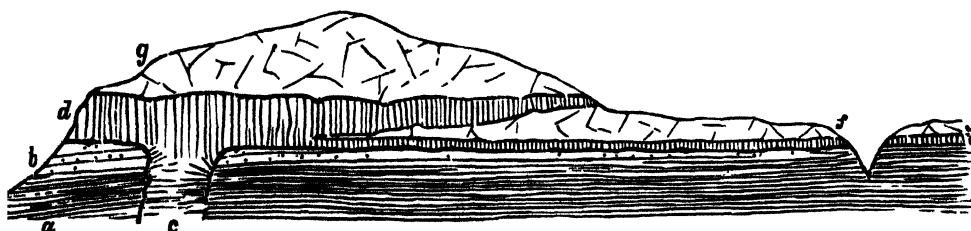
FIG 249.—Section showing the connection of a Dyke with an Intrusive Sheet, Point of Suishnish, Skye
