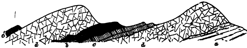
FIG 372.—Section across the Granophyre Sills at Loch a Mhullaich, above Skulamus, Skye
