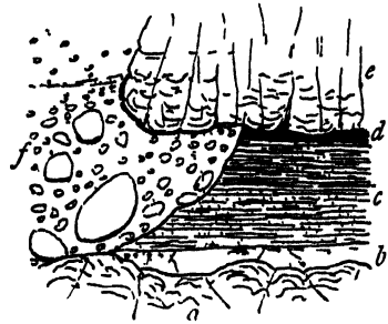
FIG 275 —Enlarged Section on the western side of Dun Beag
