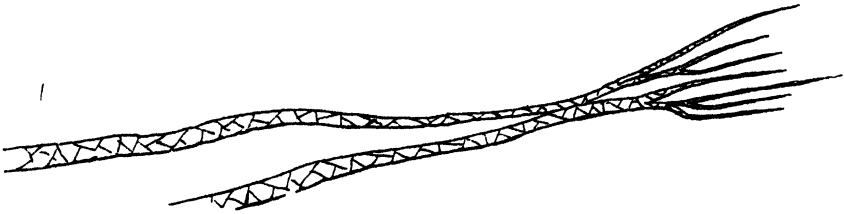
FIG 363 — Veins of granophyre traversing gabbro and splitting up into thin threads, north side of St Kilda
