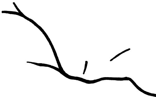
FIG 246 —Branching portion of the great Dyke near Hawick (length about one mile)
