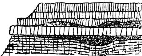
FIG 289 —Lenticular lavas western front of Hesto, Faroe Isles
