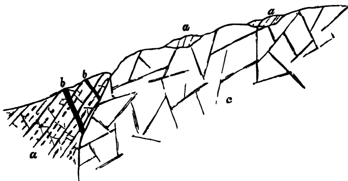
FIG. 347.—Section across the north slope of Beinn an Dubhaich, Skye. a a Cambrian limestone b b basalt dykes c granite
