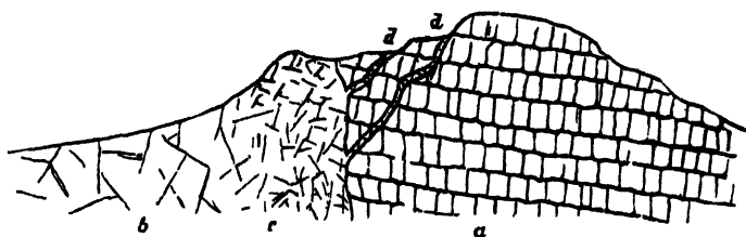
FIG 353 —Section on south side of Cruach Torr an Lochain, Mull
