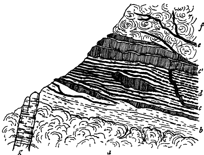
FIG 321 — Section of thin Intrusive Sheets and Veins in carbonaceous shales lying among the Plateau-basalts cliffs north of Ach na Hannait, between Portree Bay and Loch Sligachan
