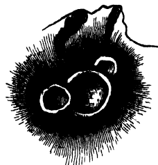
Fig 214 —Plan of the craters in Volcanello, Lipari Islands
