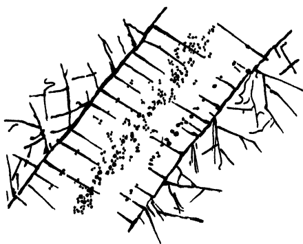
FIG 236 —Arrangement of lines of amygdaloid in a dyke, Strathmore, Skye
