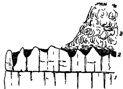
FIG 181 —Section of vesicular and amygdaloidal diabase resting on Carboniferous limestone, Peak Forest Limestone Works, Great Rocks Quarry
