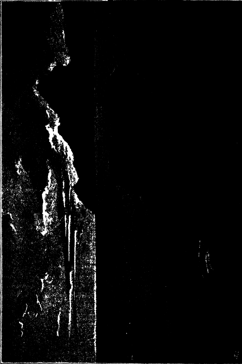
FIG. 364 —Pale granophyre injected into dark basalt, South Bay, St Kilda The crags on the further side of the bay are the gabbro sheets of the Dune (From a photograph by Colonel Evans)
