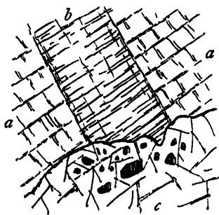
FIG 350 —Ground plan of basic dyke in Cambrian Limestone truncated by granophyre which encloses large blocks of the dyke, Torrìn, Skye
