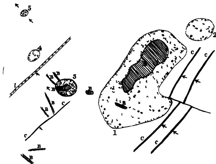
Fig 213 —Plan of volcanic necks at Kellie Law, east of Fife on the scale of three inches to one mile
