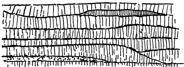
FIG 290 —Lenticular lavas east side of Svino, Faroe Isles
