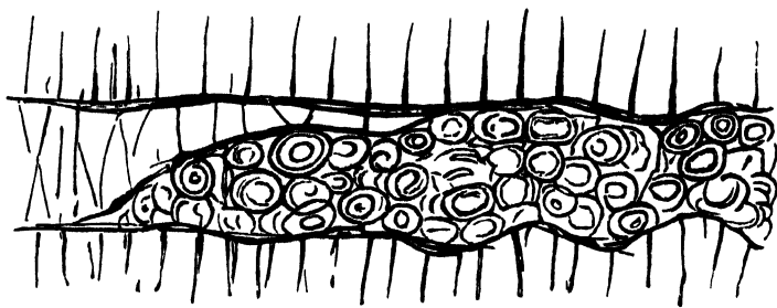
FIG. 261.—Termination of Basalt beds, Carsug, Mull
