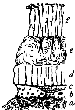
FIG 200—Section of lavas east side of Mauchline Hill
