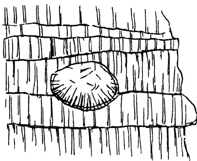
FIG 238 —Section of cylindrical vein or dyke, cutting the bedded lavas, east side of Fuglo, Faroe Islands
