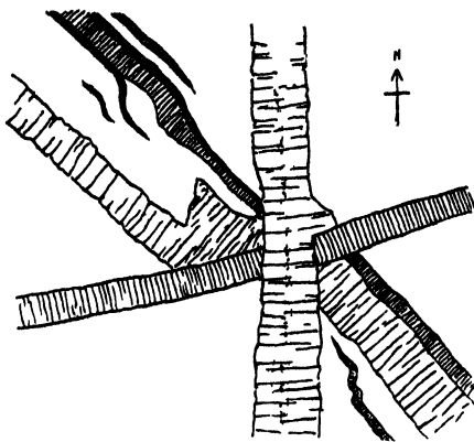
FIG 253 —Ground plan of intersecting Dykes in Lias limestone, Shore, Harribol East of Broadford, Skye
