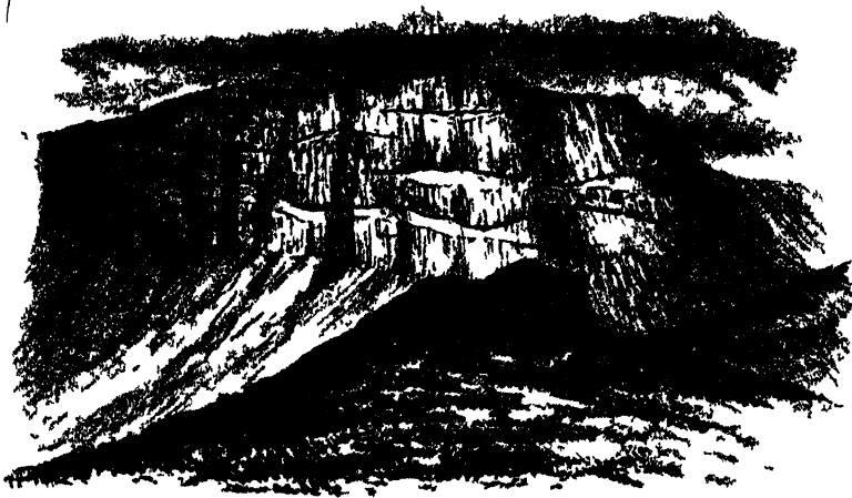
FIG 281 —View of the Scur of Eigg from the south west of the Loch a Bhealach showing the bedded character of the mass
