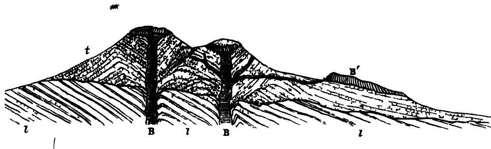
FIG. 226 — Section across Largo Law
