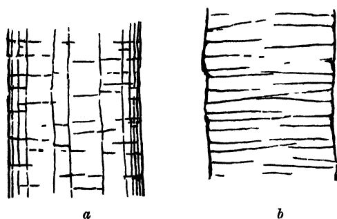
FIG 237 —Systems of joints in the dykes a, parallel, b, transverse
