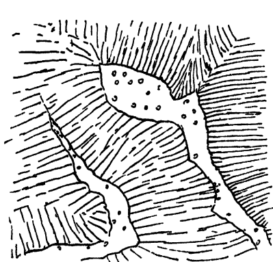
FIG 307.—Columnar Basalt invading Agglomerate of Volcanic Vent Coroghon Mòr, Isle of Canna. (Height above 20 feet.)
