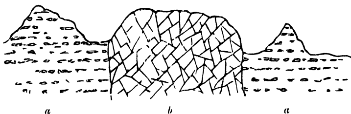
FIG. 297 —Section of Neck of Basalt, Bendoo, Ballintoy a a Chalk b neck
