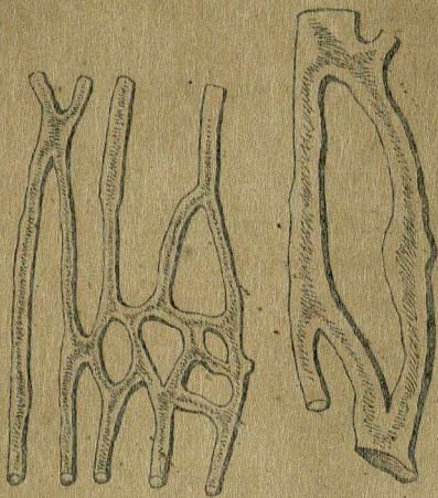
FIG. 1.—Laticiferous Tissue.
